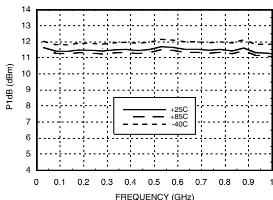
P1dB vs. Temperature @ 3V
