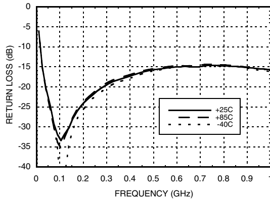
Output Return Loss vs. Temperature @ 3V
