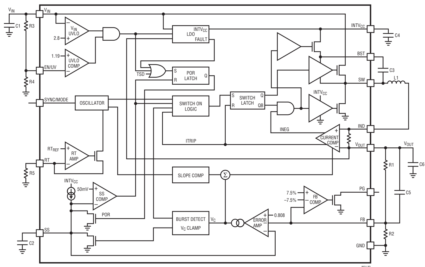
Figure 1. Block Diagram
