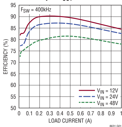
Efficiency at V_{OUT} = 5V
