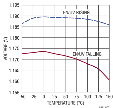
EN/UV Thresholds
