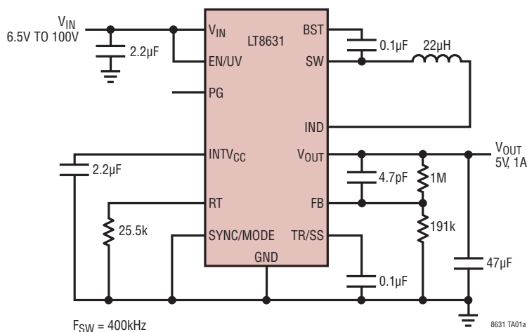
5V, 1A Step-Down Converter
