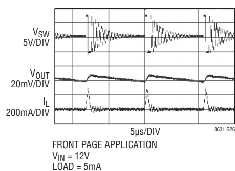
Burst Waveforms
