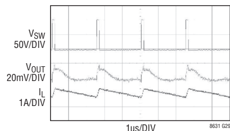
Switching Waveforms
