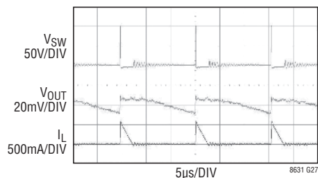
Burst Waveforms
