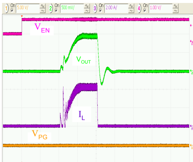
Figure 25. Over-Current at Startup, R_{LOAD}=200\text{ m}\Omega , 50 μs/div.
