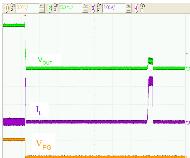
Figure 23. VOUT to GND Short Circuit, 200 μs/div.
