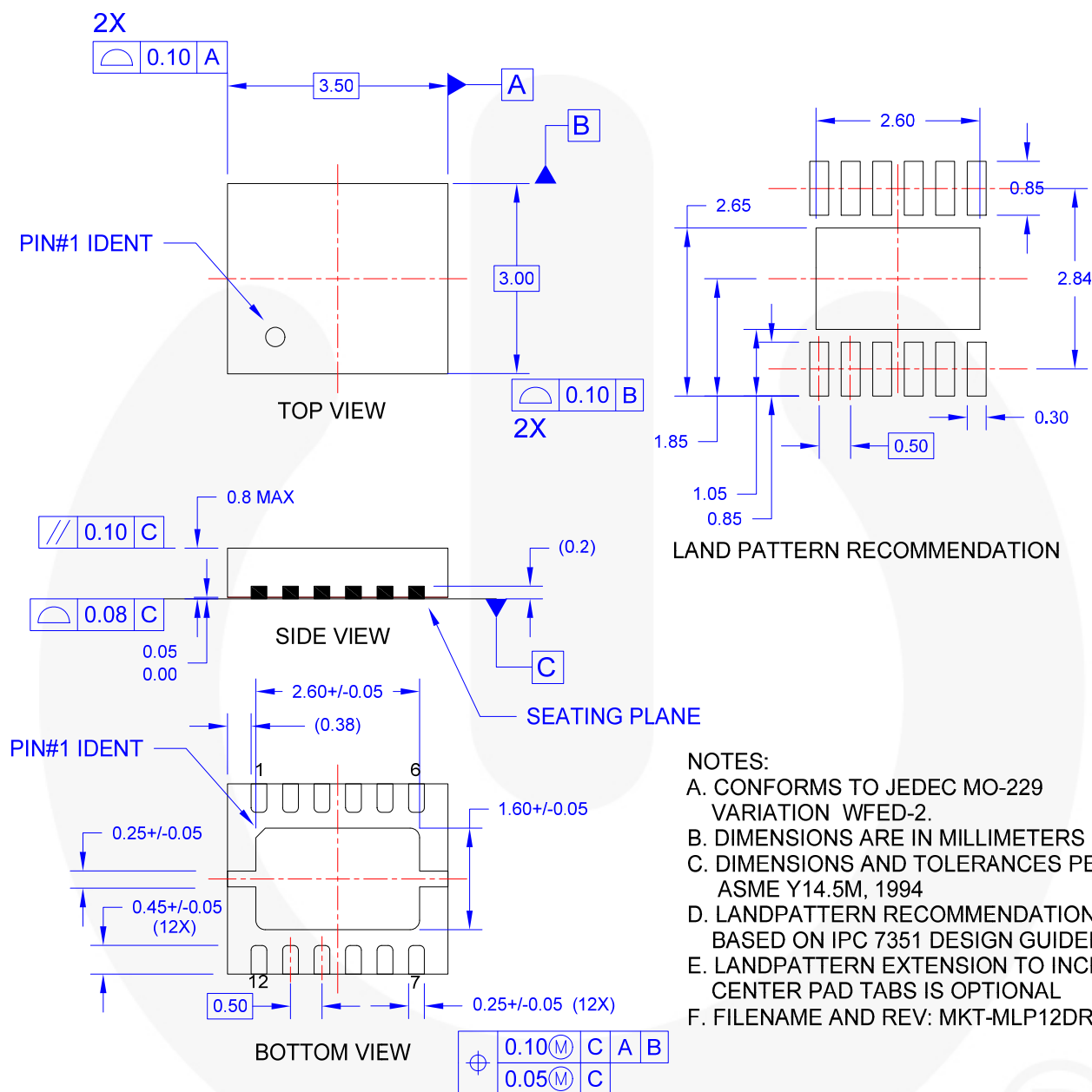
Figure 28. 12-lead 3 x 3.5 mm MLP
