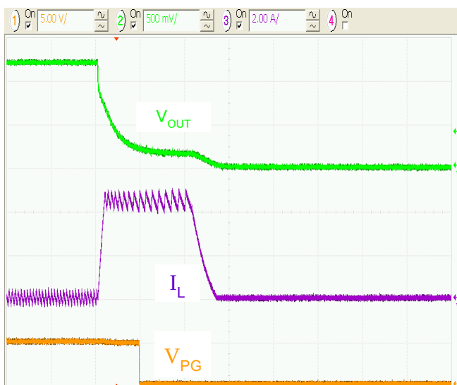
Figure 24. VOUT to GND Short Circuit, 5 μs/div.
