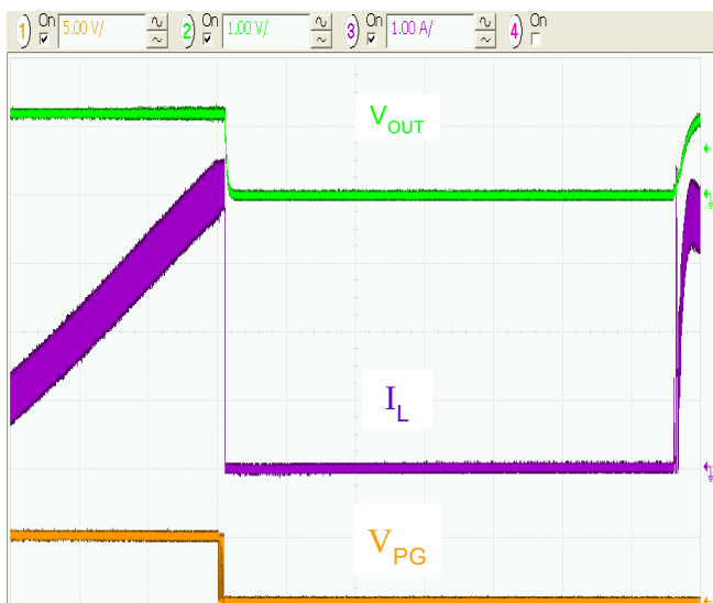
Figure 26. Progressive Overload, 200 μs/div.
