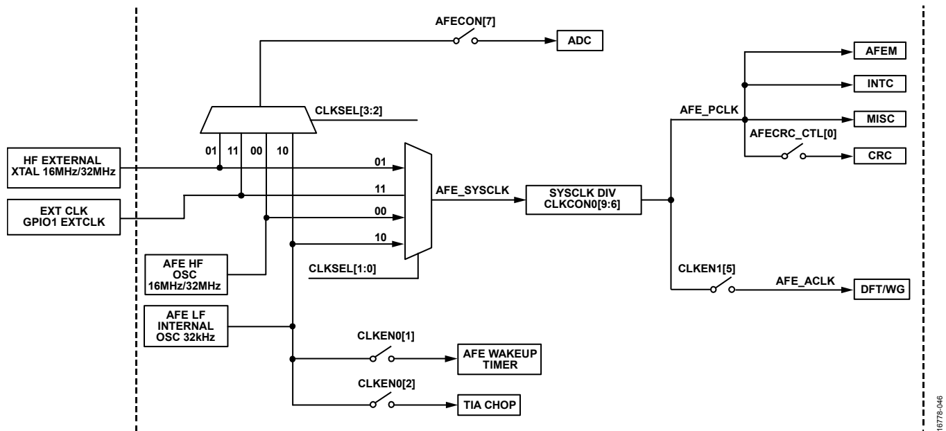
Figure 53. AD5940/AD5941 System Clock Architecture
