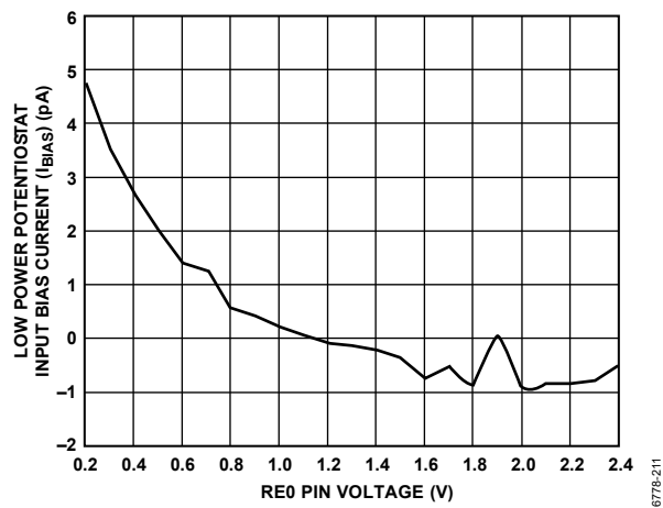
Figure 12. Low Power Potentiostat Input Bias Current ( I_{BIAS} ) vs. RE0 Pin Voltage
