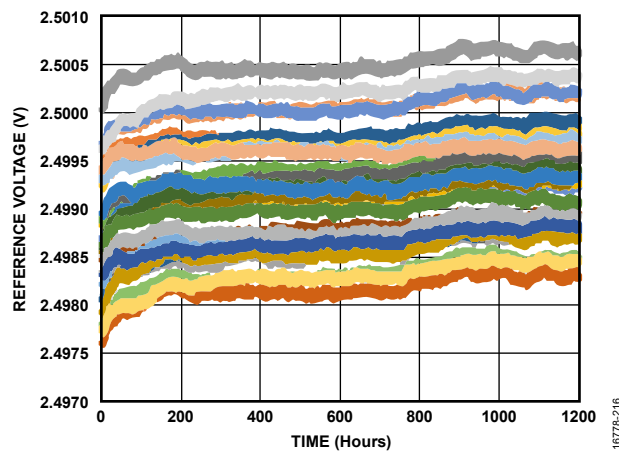
Figure 17. V_{REF} 2.5 V Lifetime Drift
