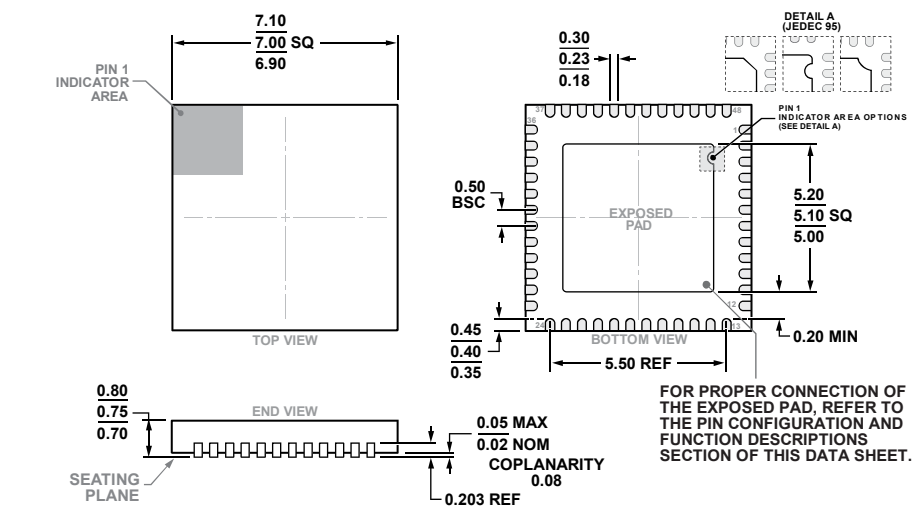
Figure 60. 48-Lead Lead Frame Chip Scale Package [LFCSP] 7 mm × 7 mm Body and 0.75 mm Package Height (CP-48-4)
