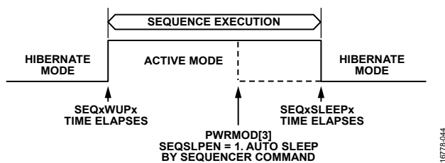
Figure 50. Sleep and Wake-Up Timing Diagram
