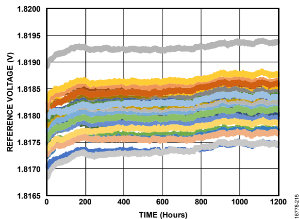
Figure 16. V_{REF} 1.8 V Lifetime Drift
