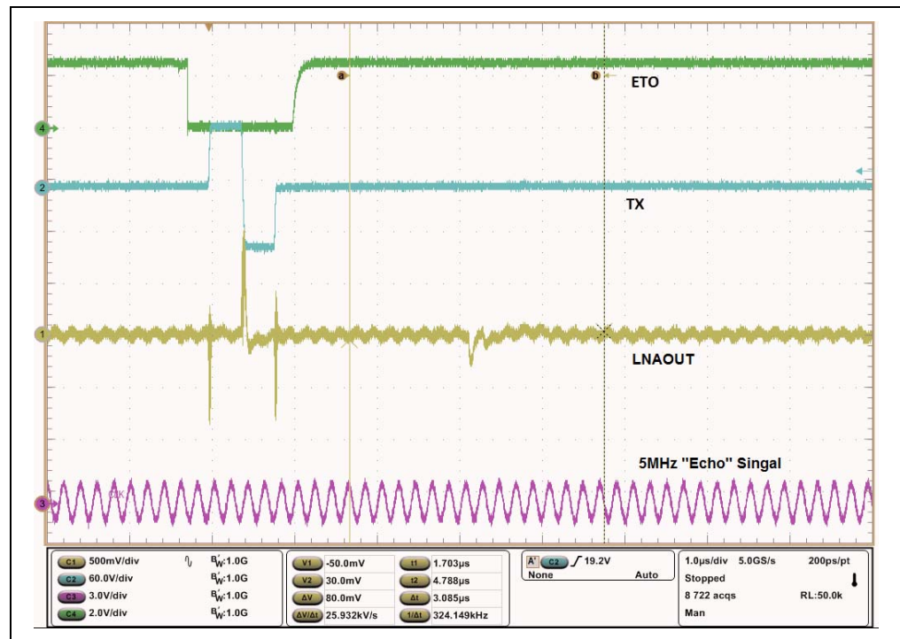
FIGURE C-9: LNAOut RX0 Signal After TX, 1-Cycle, ±80V.
