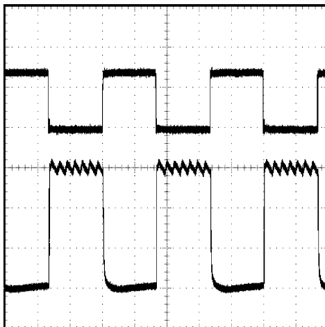
I LED = 6A nominal, V IN = 3.3V, V EE = -12V Top trace: DIM input, 2V/div, DC Bottom trace: I LED , 2A/div, DC T = 10μs/div Figure 8. 30kHz PWM Dimming Waveform Showing Inductor Ripple Current
