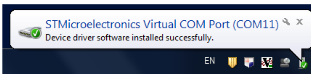
Figure 5. Notification message
