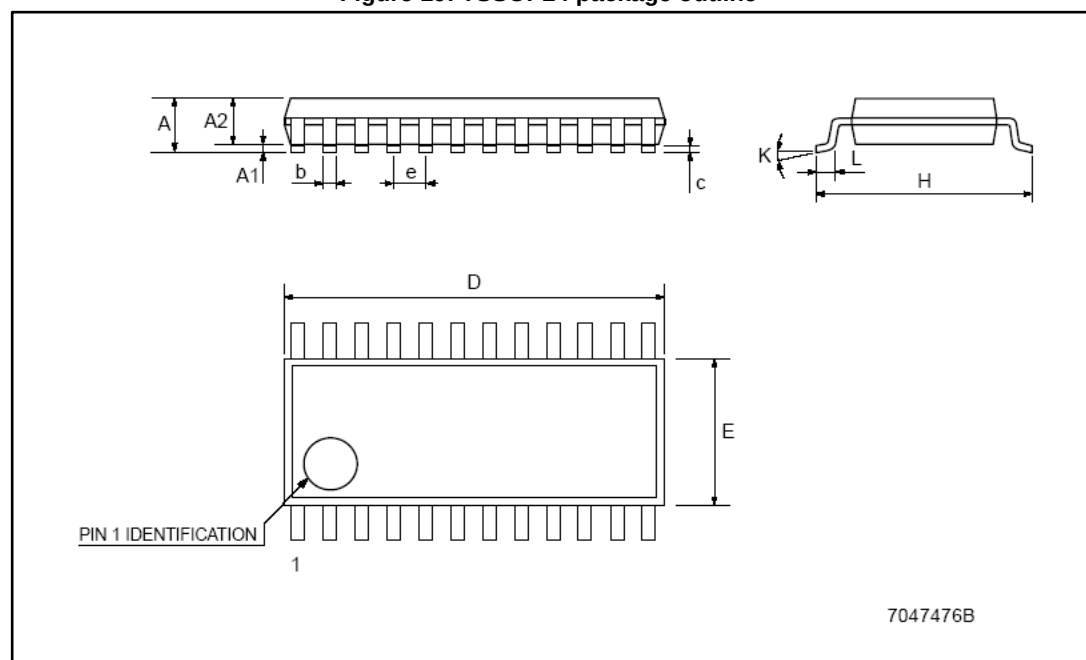
Figure 19: TSSOP24 package outline
