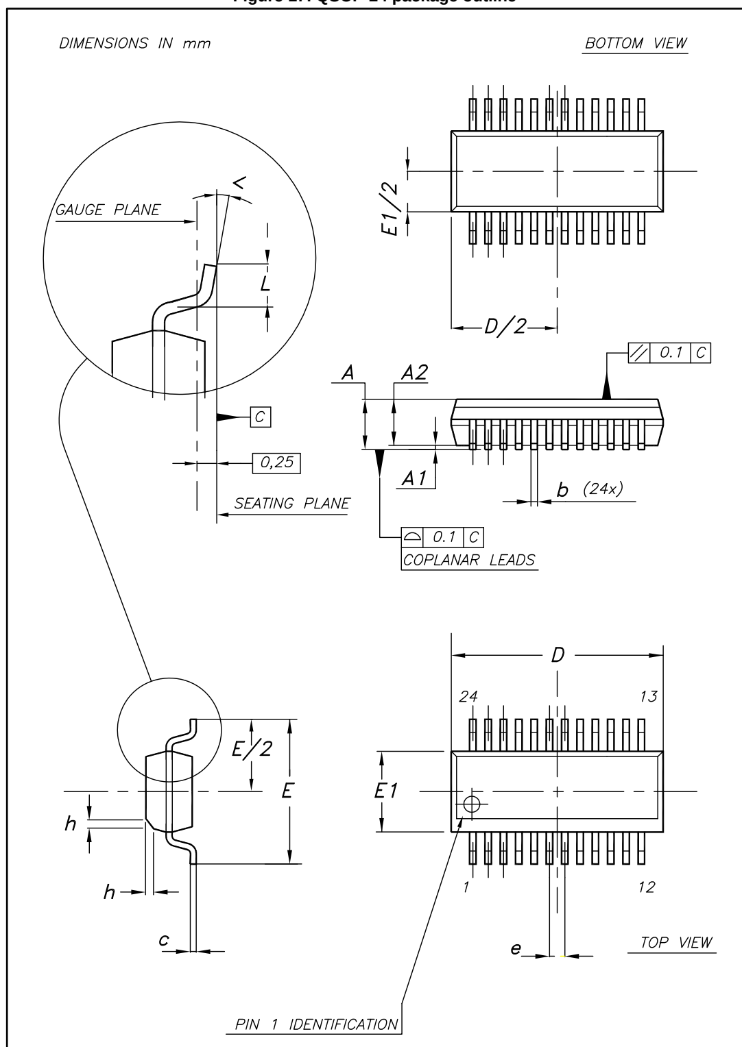
Figure 17: QSOP-24 package outline
