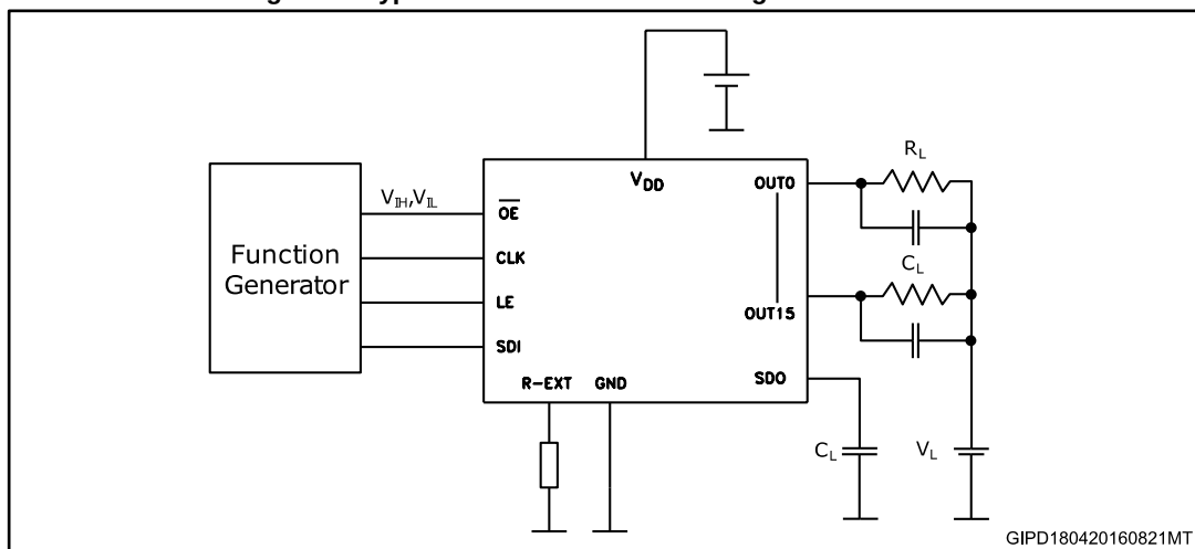
Figure 9: Typical test circuit for switching characteristics
