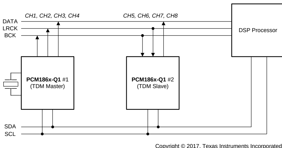
Figure 59. TDM With Two PCM186x-Q1
