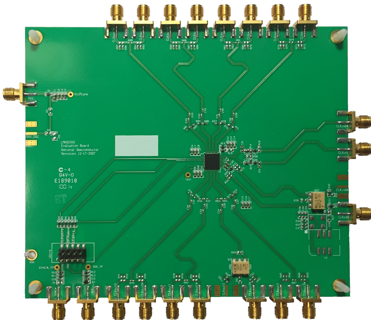
Figure 1. LMK01000EVM
