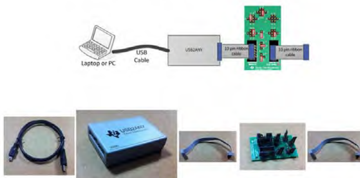
Figure 8. USB2ANY-uWIRE Set up
