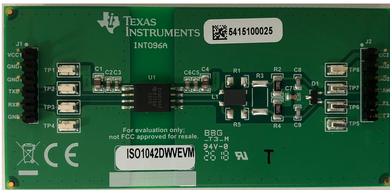
Figure 3. ISO1042DWVEVM Photograph
