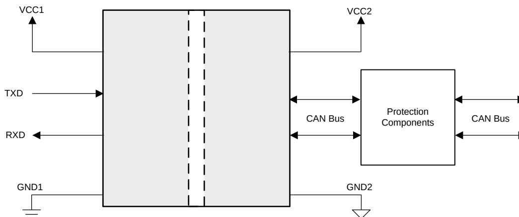
Figure 2. ISO1042DWVEVM Configuration
