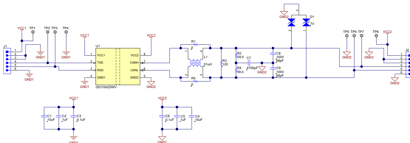
Figure 4. ISO1042DWVEVM Schematic
