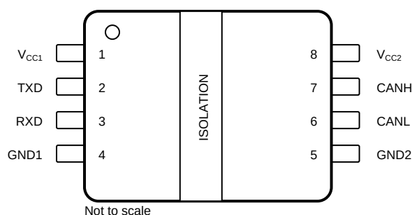
Figure 1. ISO1042DWV Pin Configuration
