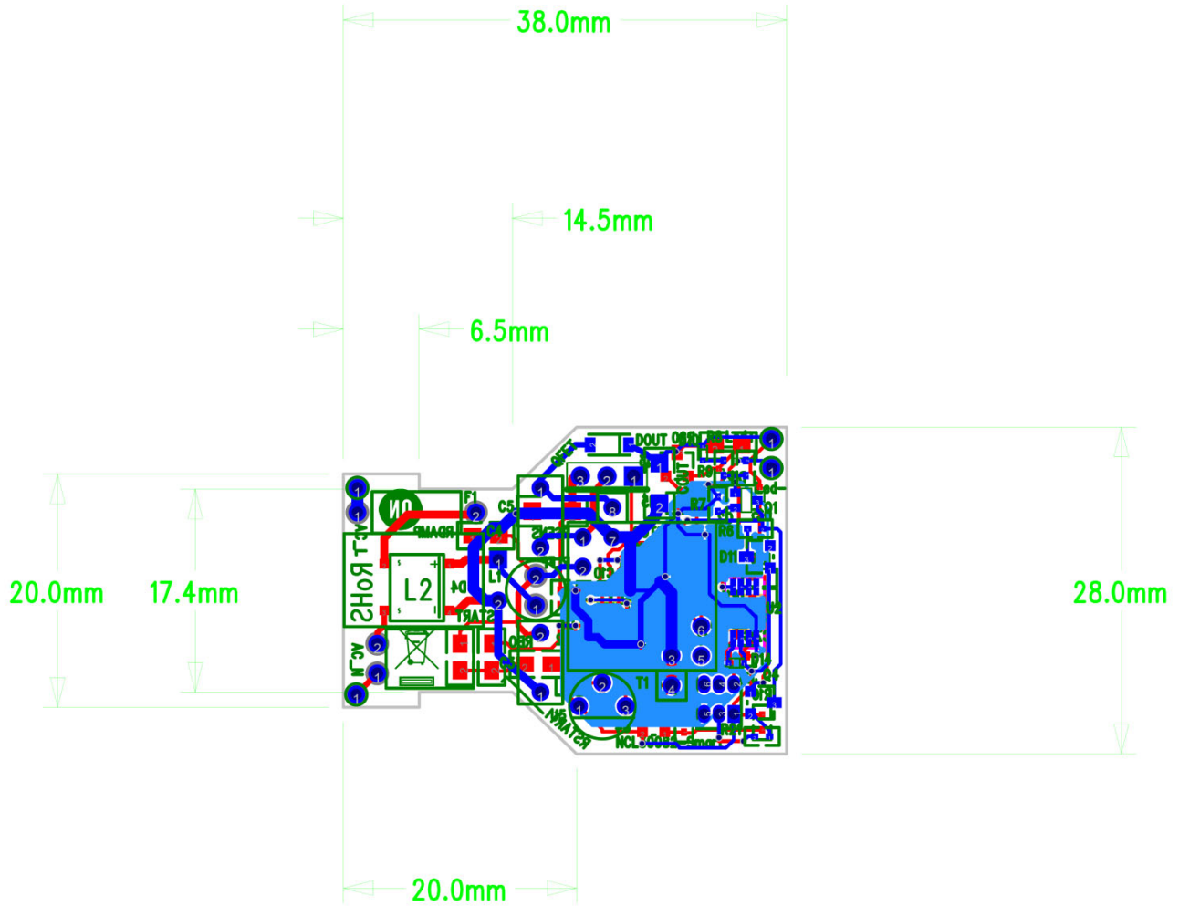
Figure 8. PCB Outline
