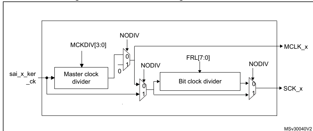
Figure 360. Audio block clock generator overview
