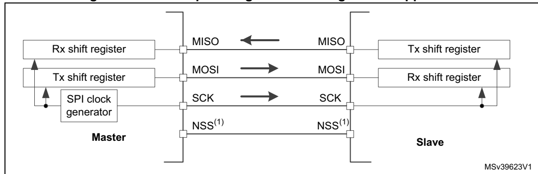
Figure 305. Full-duplex single master/ single slave application
