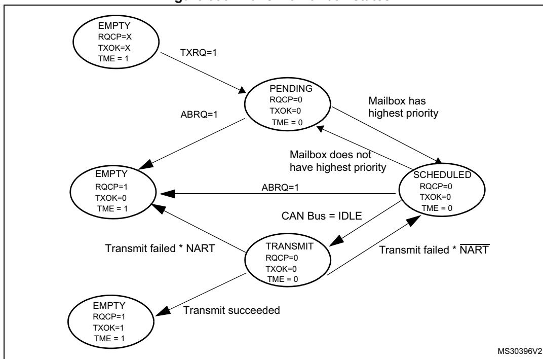
Figure 390. Transmit mailbox states
