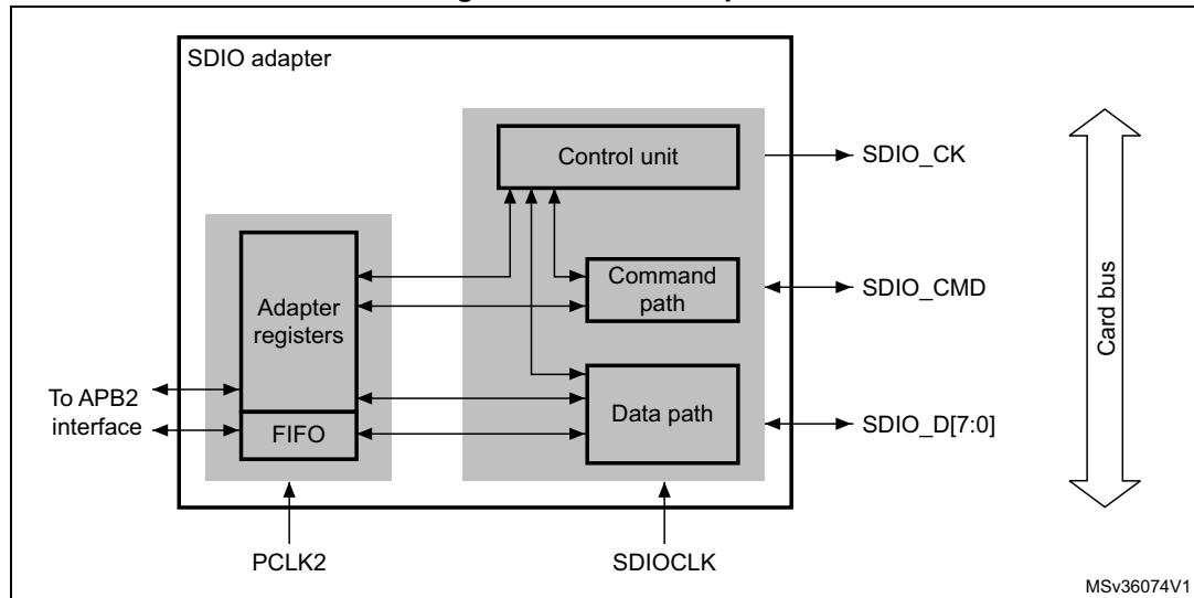
Figure 376. SDIO adapter
