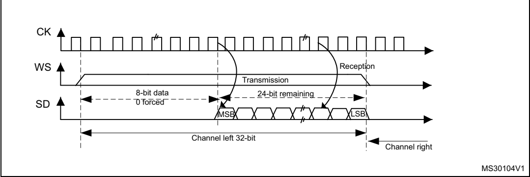
Figure 329. LSB justified 24-bit frame length with CPOL = 0
