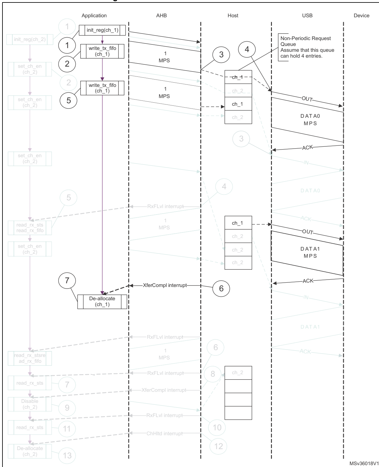
Figure 412. Normal bulk/control OUT/SETUP
