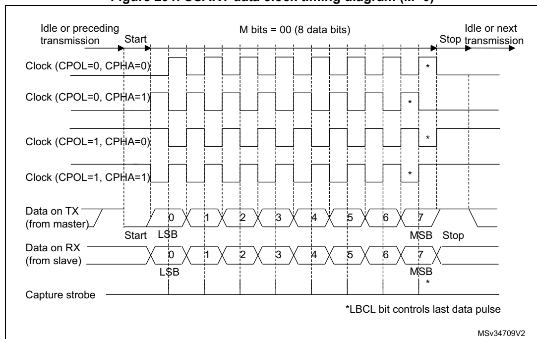
Figure 291. USART data clock timing diagram (M=0)
