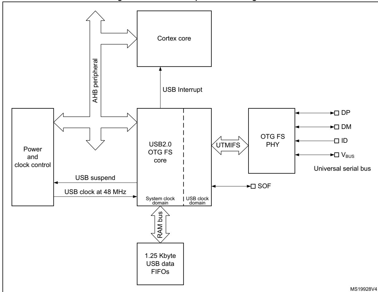
Figure 400. OTG full-speed block diagram
