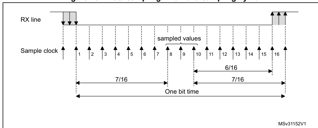
Figure 284. Data sampling when oversampling by 16
