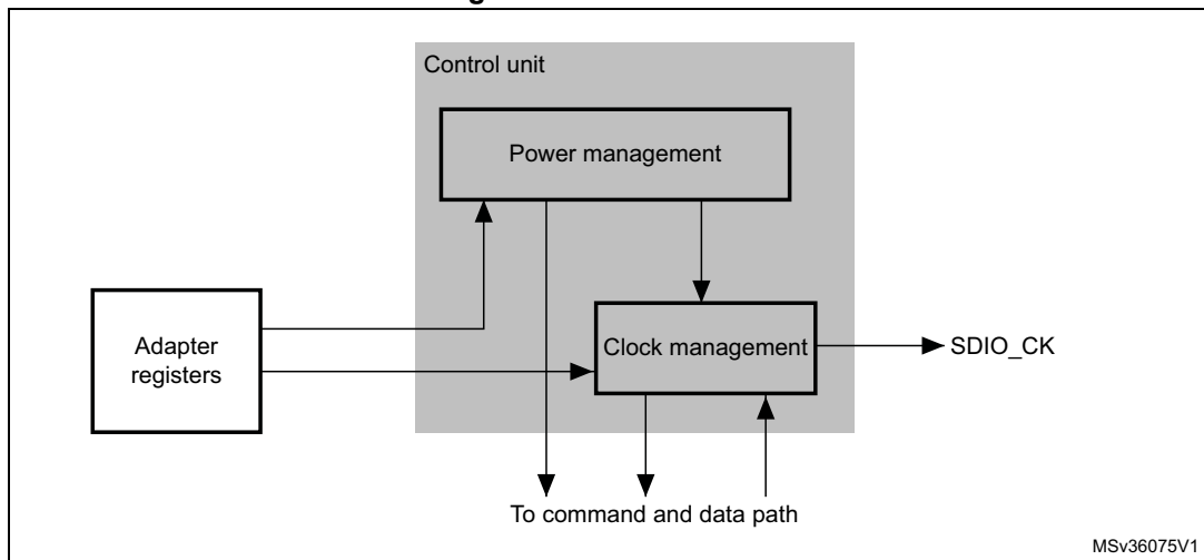
Figure 377. Control unit
