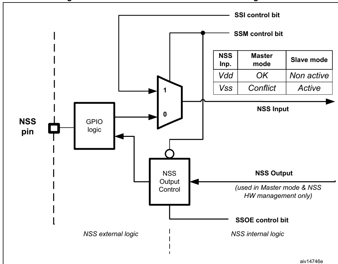
Figure 310. Hardware/software slave select management
