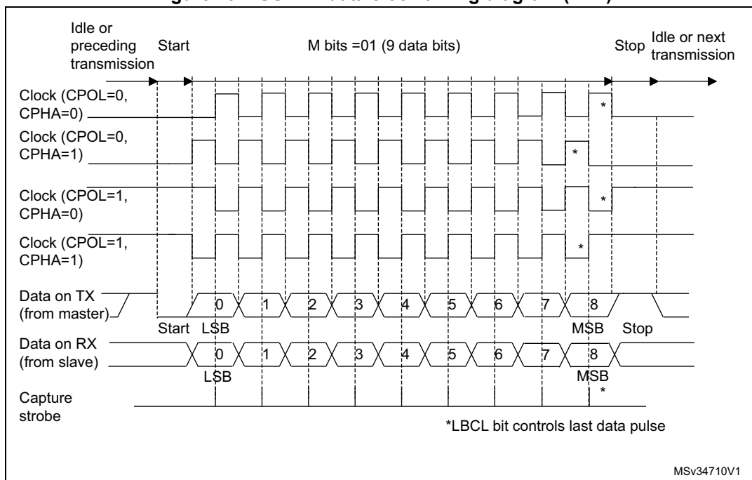
Figure 292. USART data clock timing diagram (M=1)
