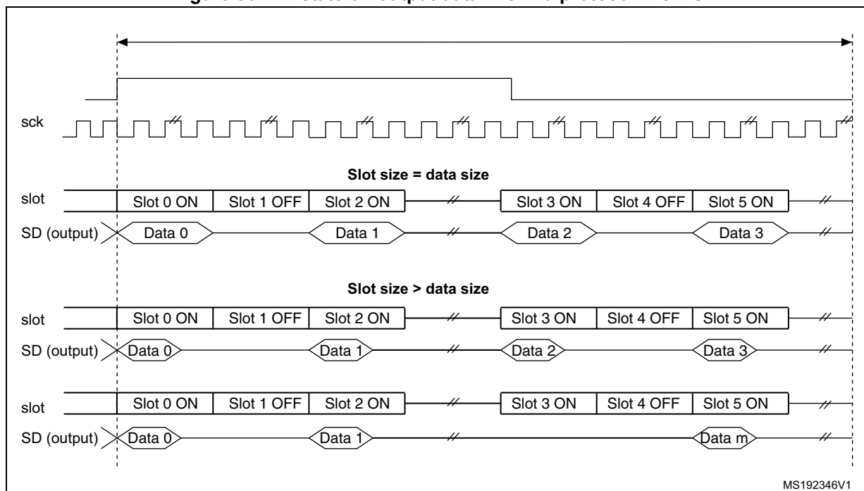
Figure 367. Tristate on output data line in a protocol like I2S
