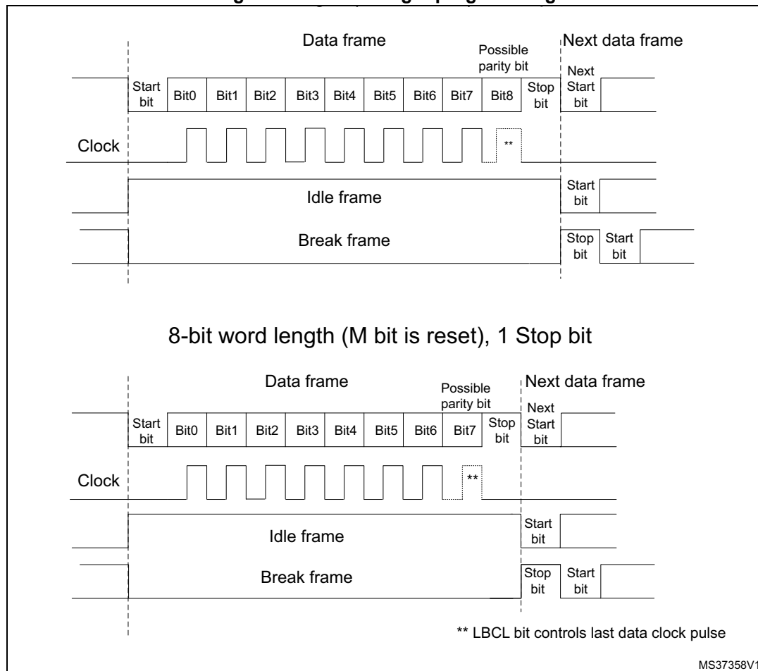
Figure 280. Word length programming
