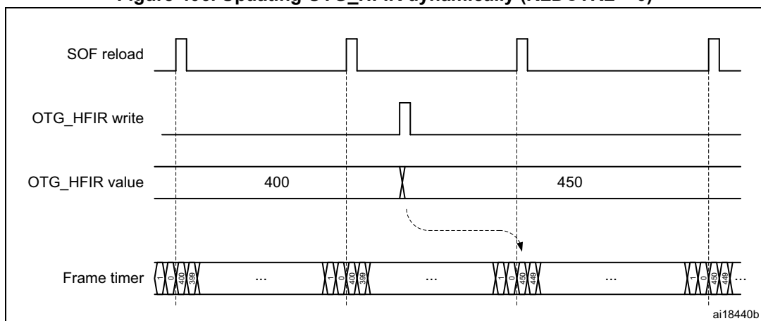
Figure 406. Updating OTG_HFIR dynamically (RLDCTRL = 0)
