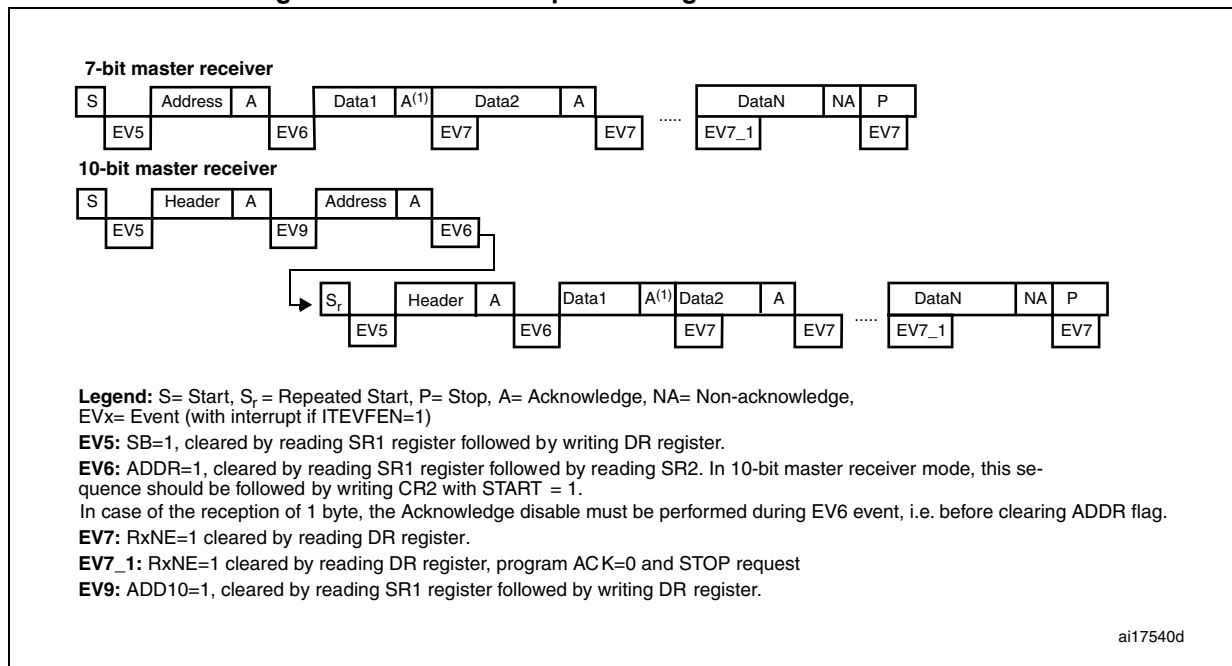
Figure 277. Transfer sequence diagram for master receiver
