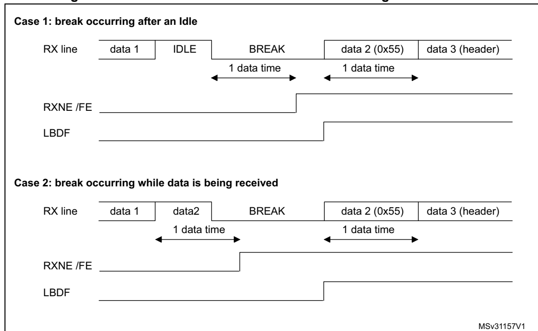
Figure 289. Break detection in LIN mode vs. Framing error detection
