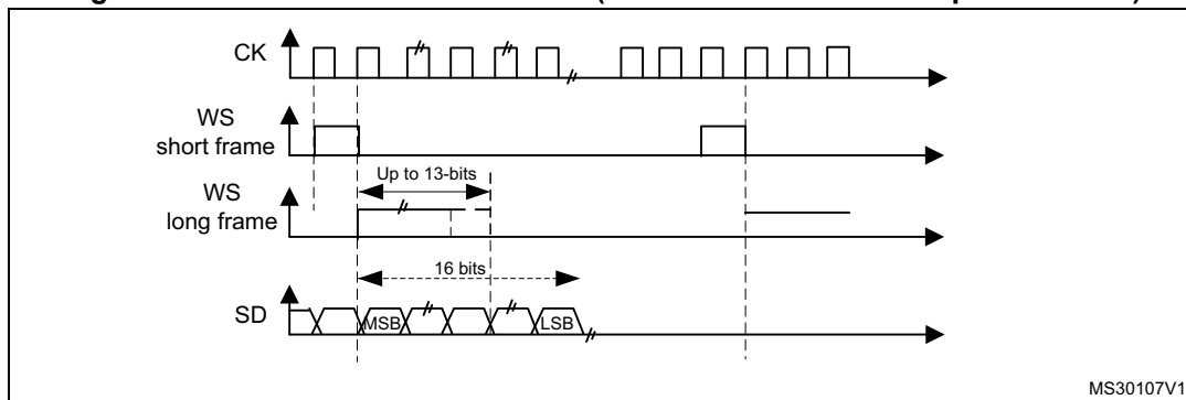
Figure 335. PCM standard waveforms (16-bit extended to 32-bit packet frame)
