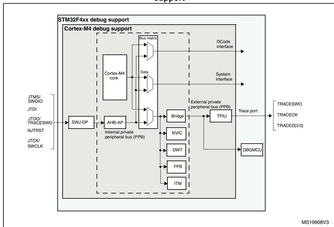
Figure 442. Block diagram of STM32 MCU and Cortex®-M4 with FPU-level debug support
