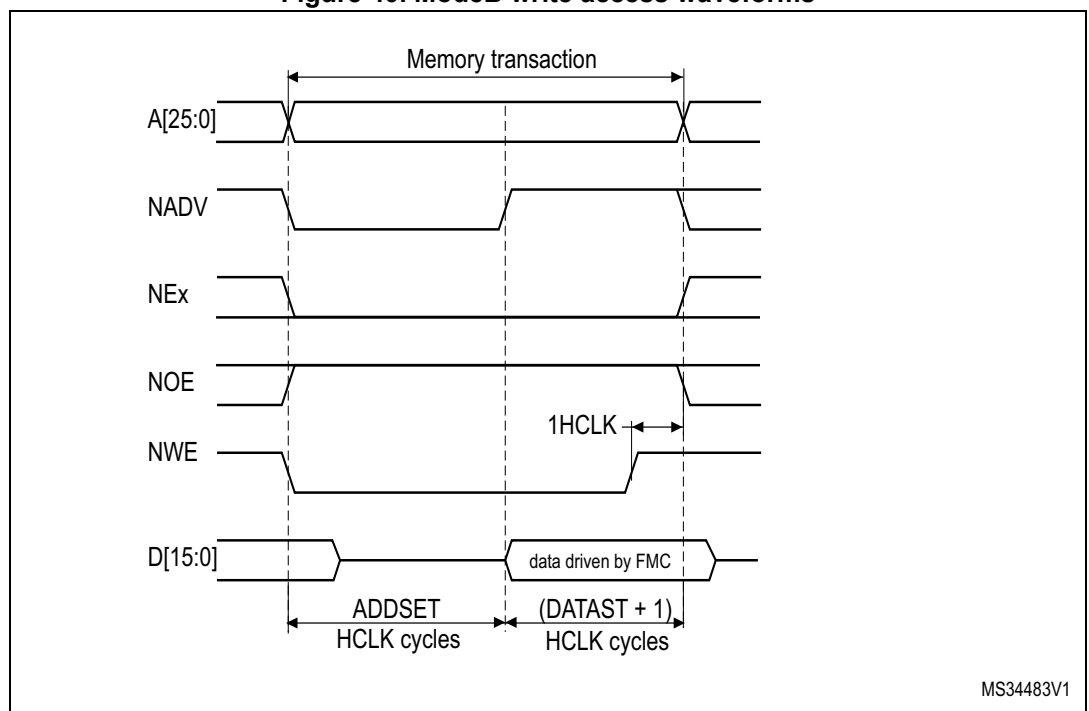
Figure 40. ModeB write access waveforms
