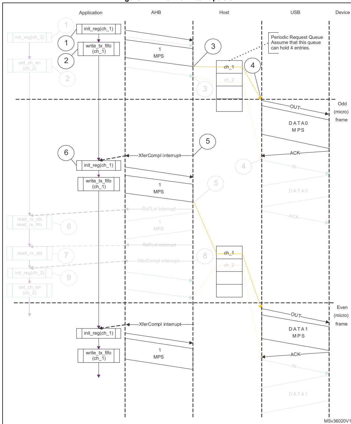
Figure 414. Normal interrupt OUT
