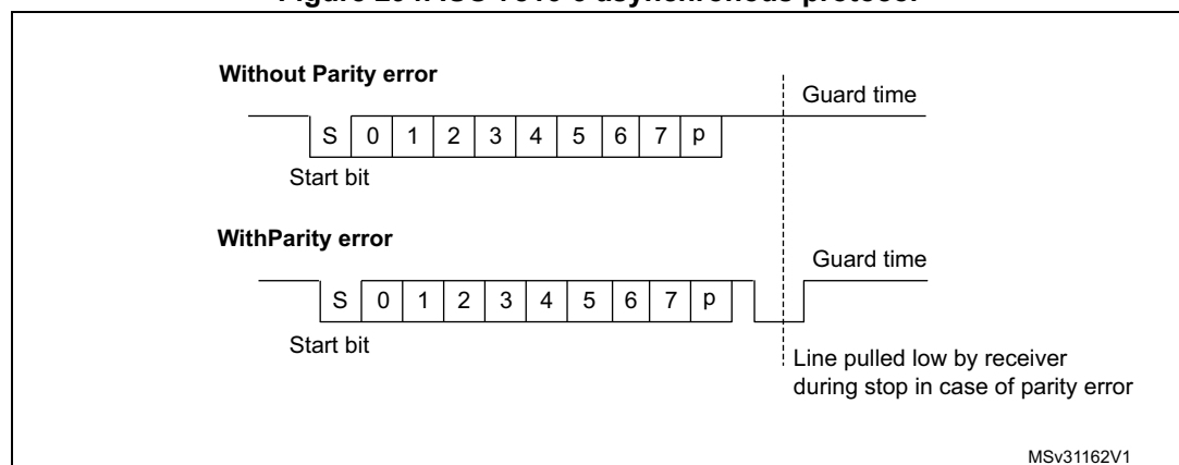
Figure 294. ISO 7816-3 asynchronous protocol
