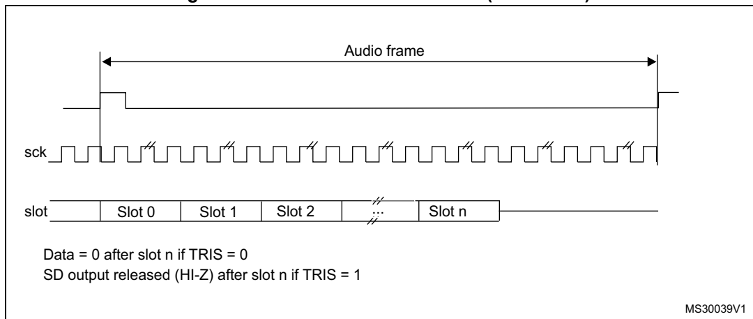
Figure 357. FS role is start of frame (FSDEF = 0)
