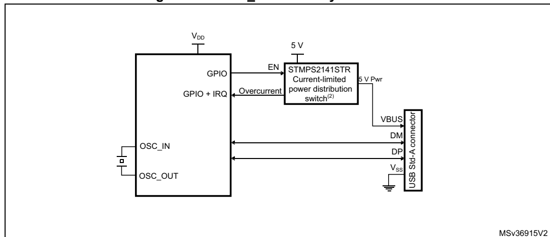
Figure 404. USB_FS host-only connection
