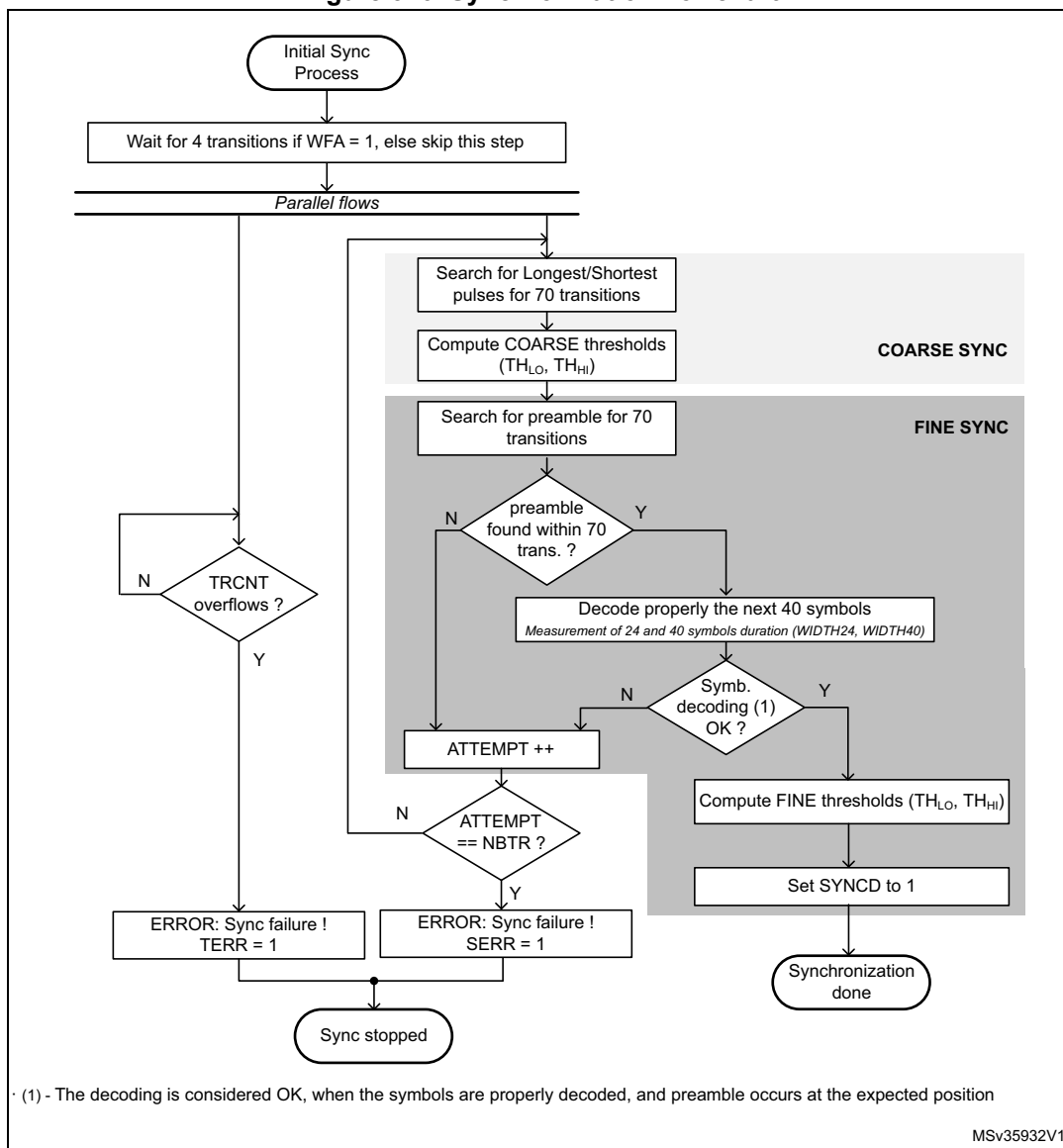
Figure 346. Synchronization flowchart
