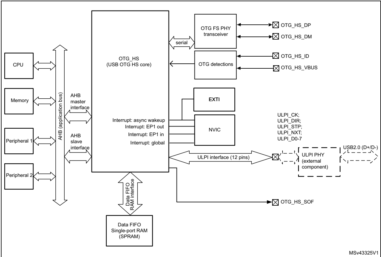
Figure 401. OTG high-speed block diagram
