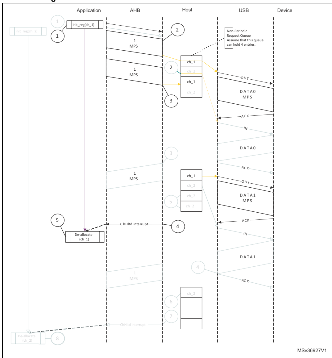
Figure 418. Normal bulk/control OUT/SETUP transactions - DMA
