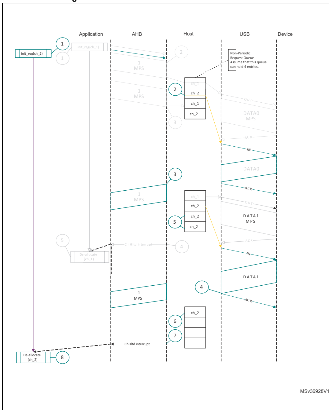
Figure 419. Normal bulk/control IN transaction - DMA
