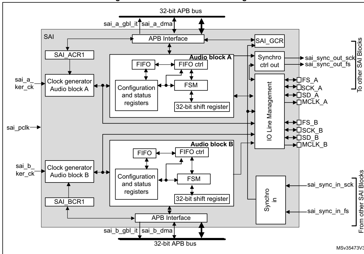
Figure 354. SAI functional block diagram
