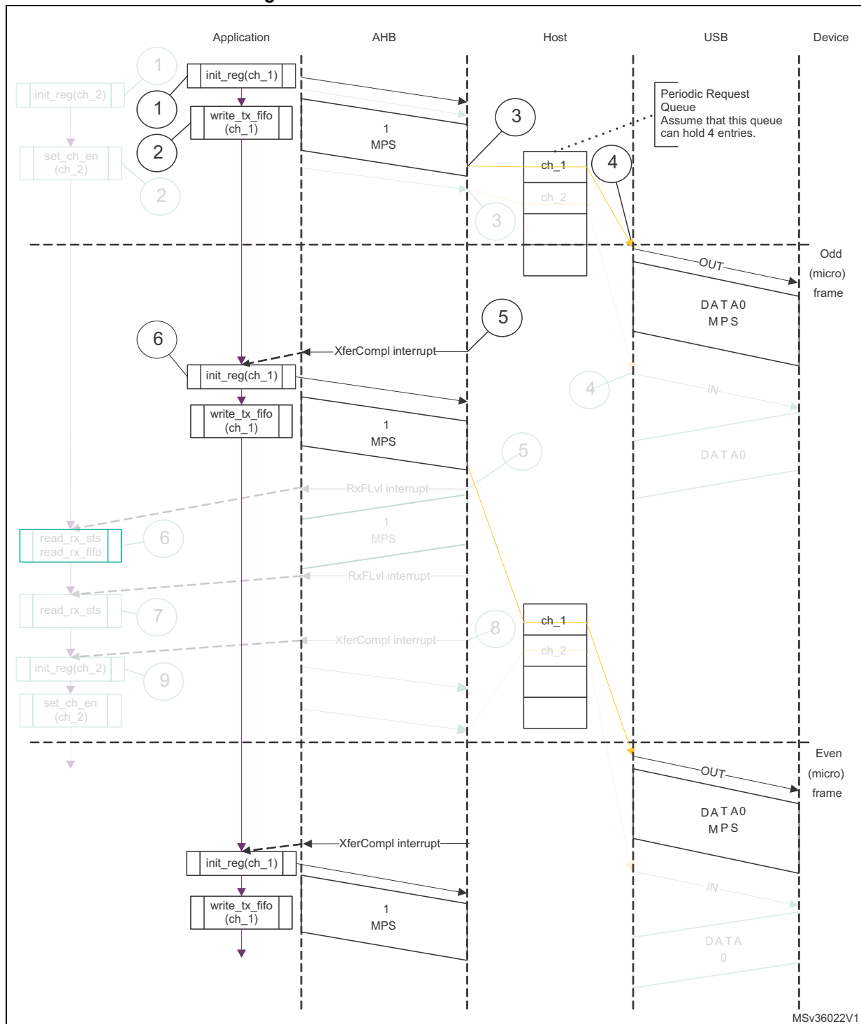
Figure 416. Isochronous OUT transactions
