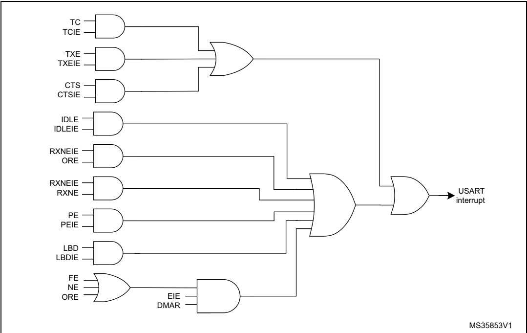
Figure 303. USART interrupt mapping diagram
