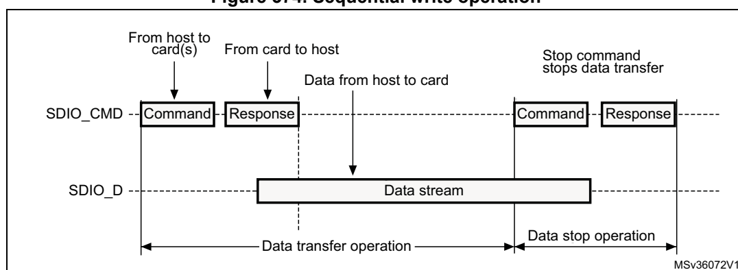
Figure 374. Sequential write operation
