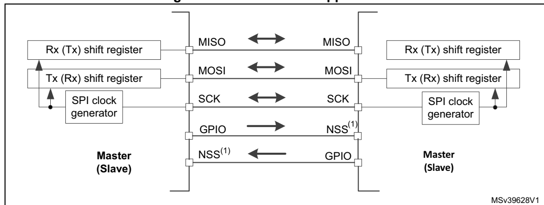
Figure 309. Multi-master application
