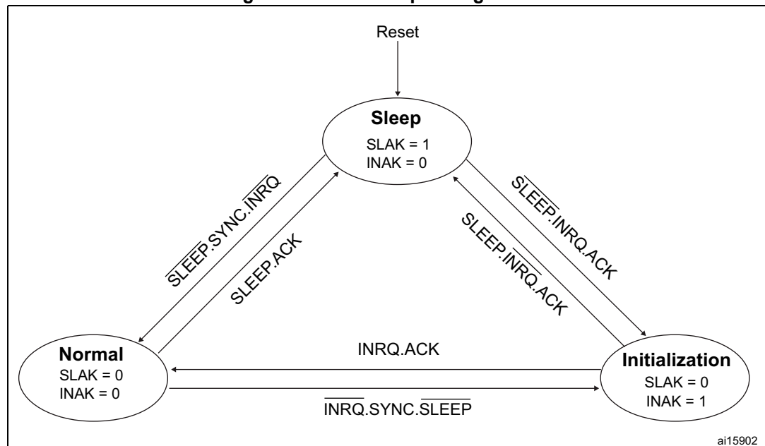
Figure 386. bxCAN operating modes
