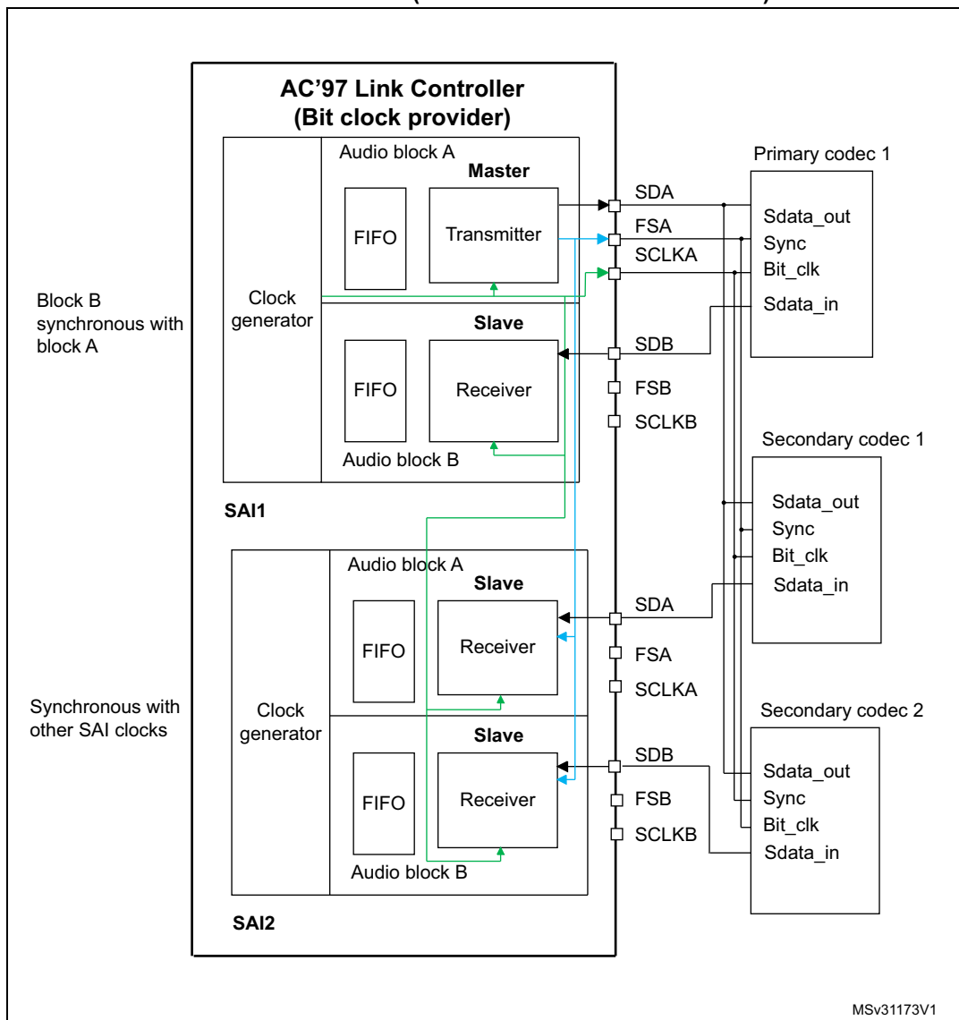
Figure 362. Example of typical AC'97 configuration on devices featuring at least 2 embedded SAI (three external AC'97 decoders)
