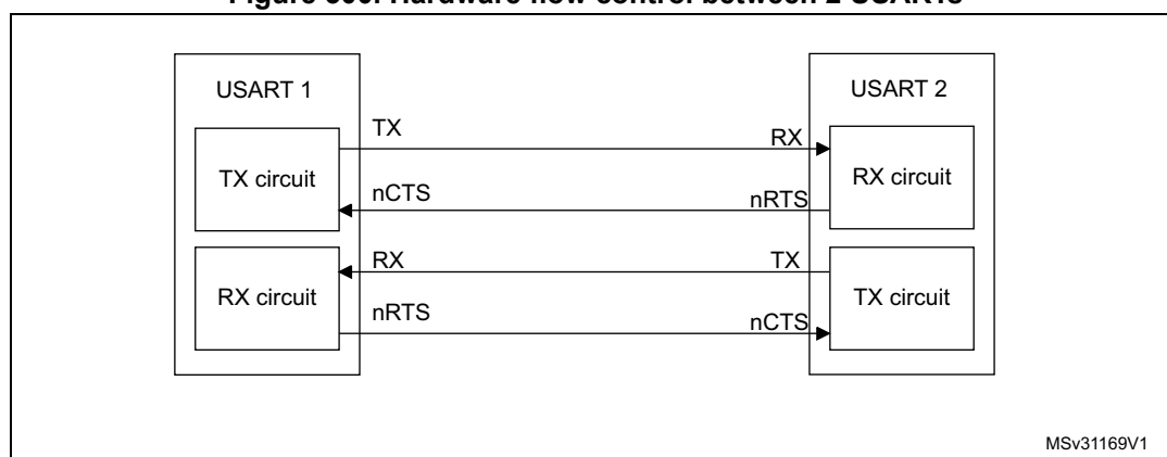
Figure 300. Hardware flow control between 2 USARTs
