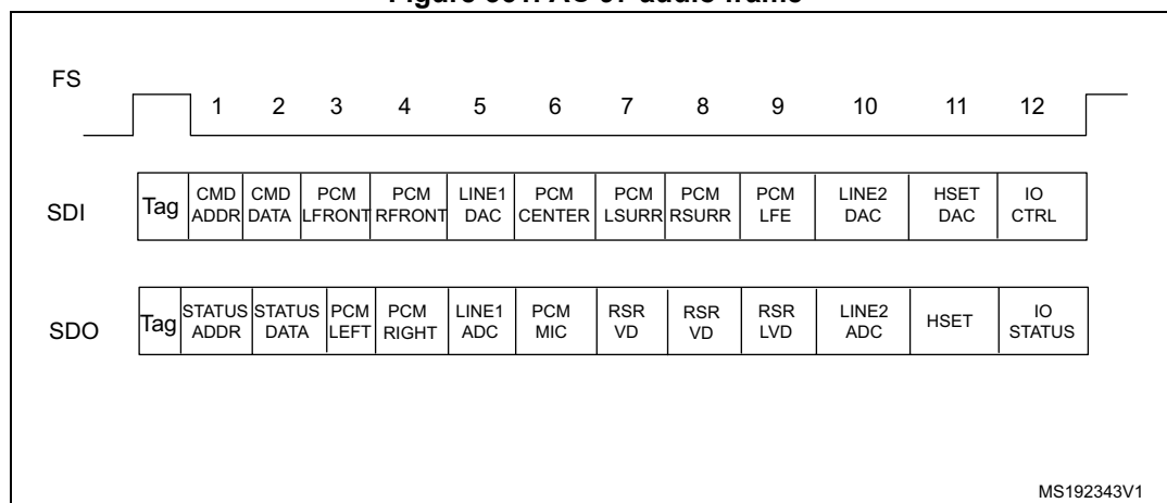
Figure 361. AC'97 audio frame
