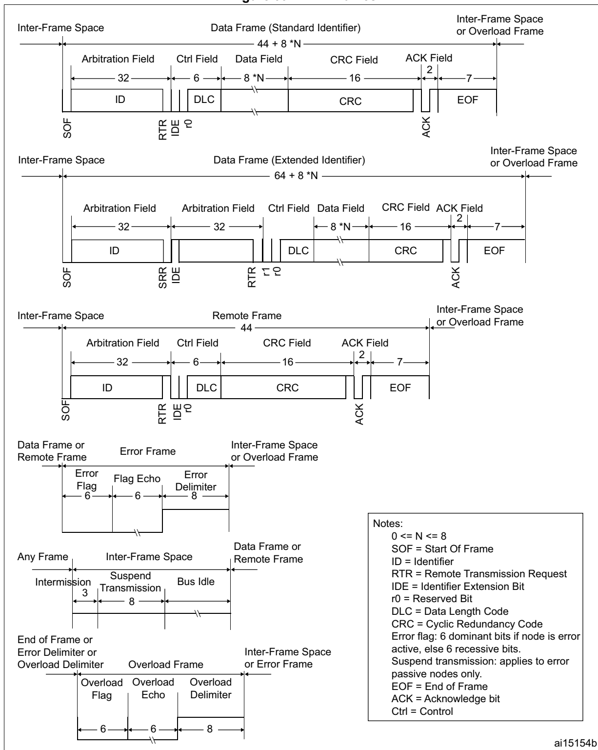
Figure 397. CAN frames
