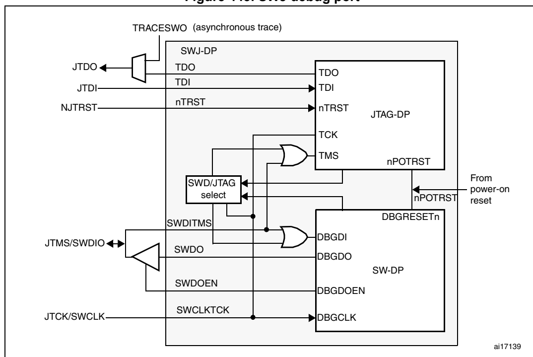
Figure 443. SWJ debug port
