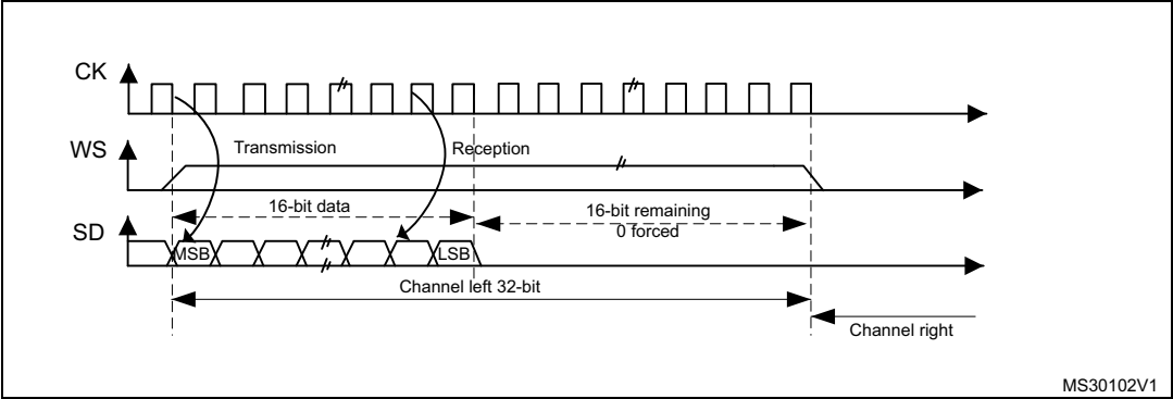
Figure 327. MSB justified 16-bit extended to 32-bit packet frame with CPOL = 0
