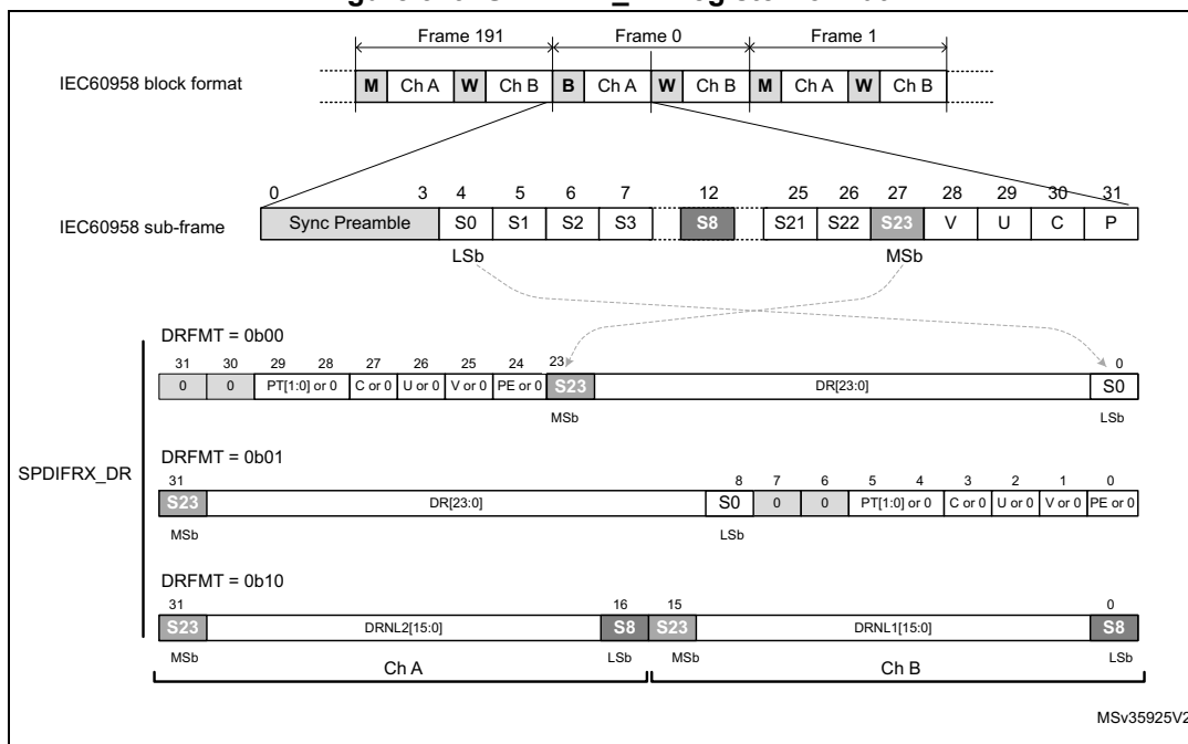
Figure 349. SPDIFRX_DR register format
