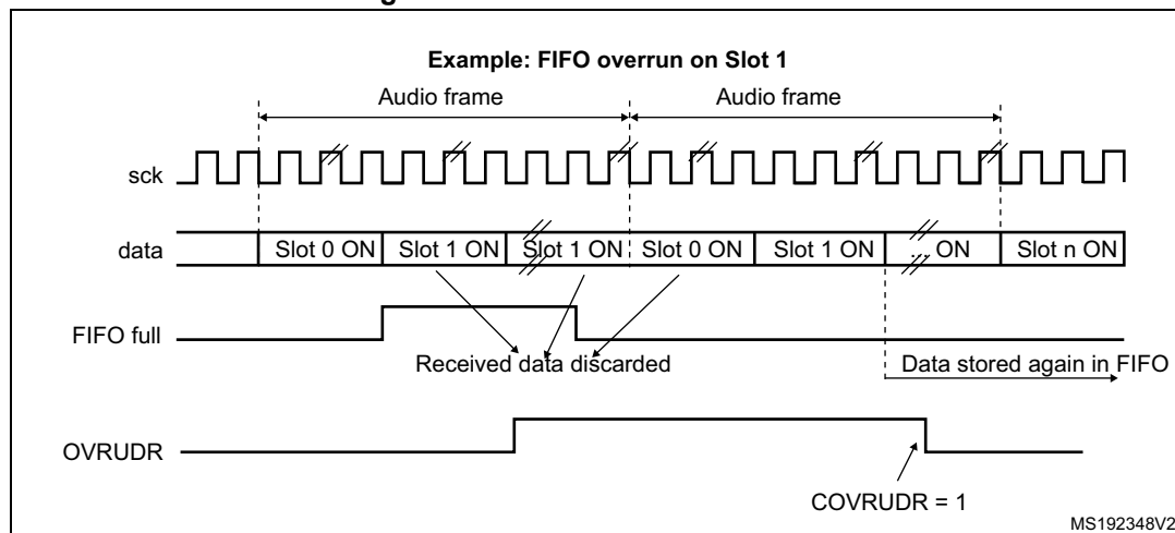
Figure 368. Overrun detection error
