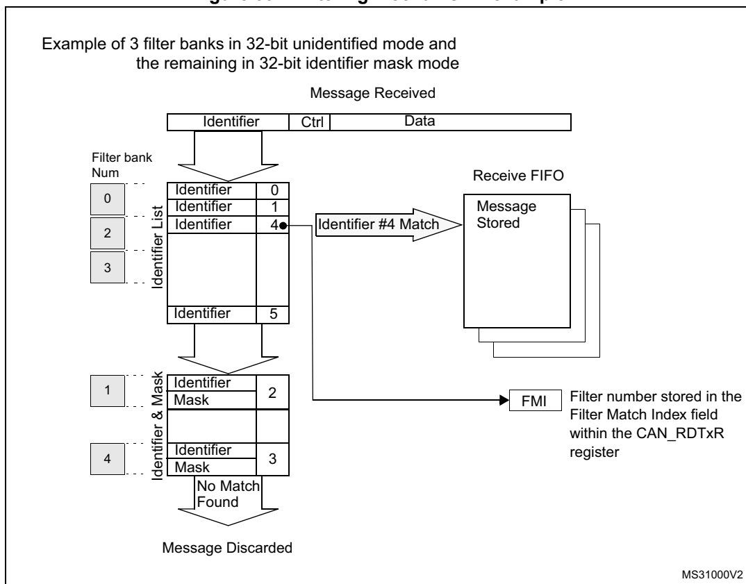
Figure 394. Filtering mechanism - example
