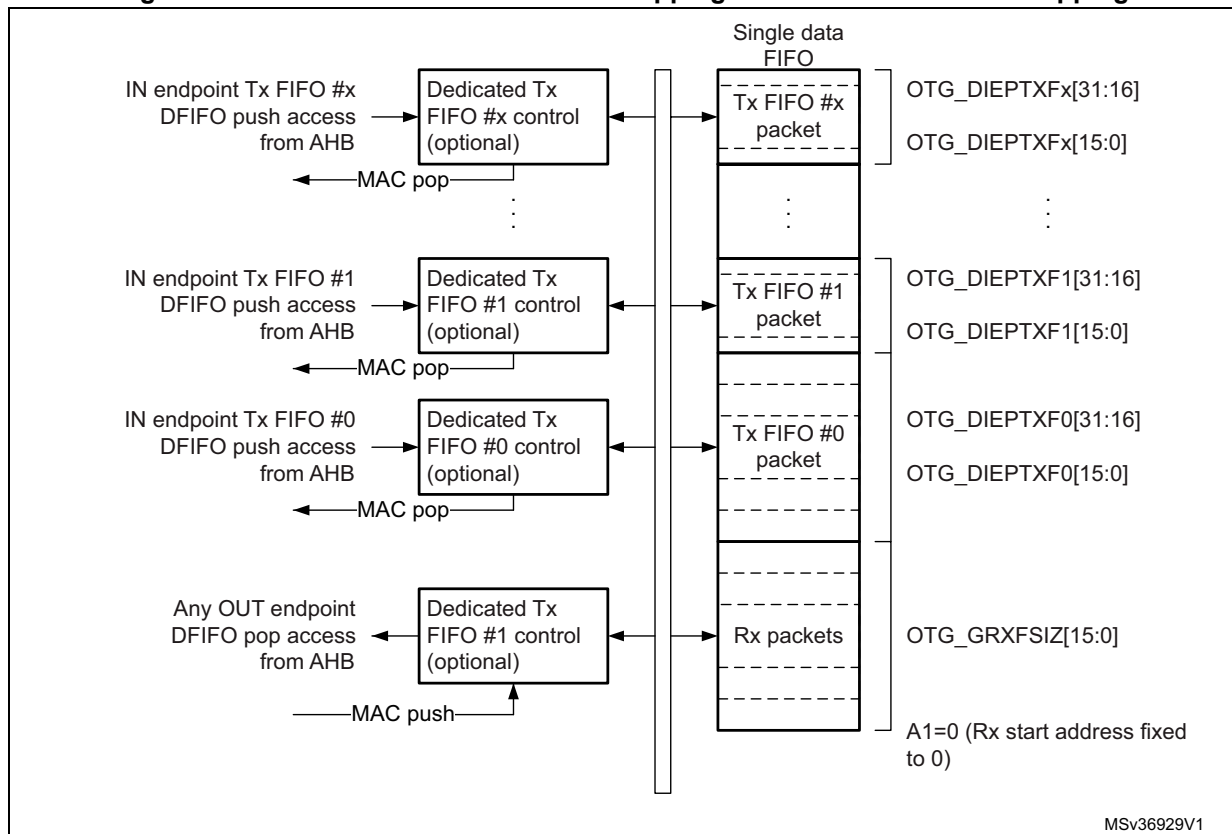
Figure 407. Device-mode FIFO address mapping and AHB FIFO access mapping
