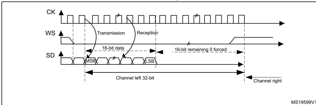
Figure 323. I 2 S Philips standard (16-bit extended to 32-bit packet frame with CPOL = 0)
