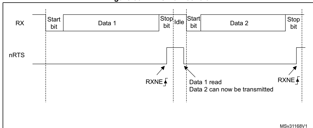
Figure 301. RTS flow control
