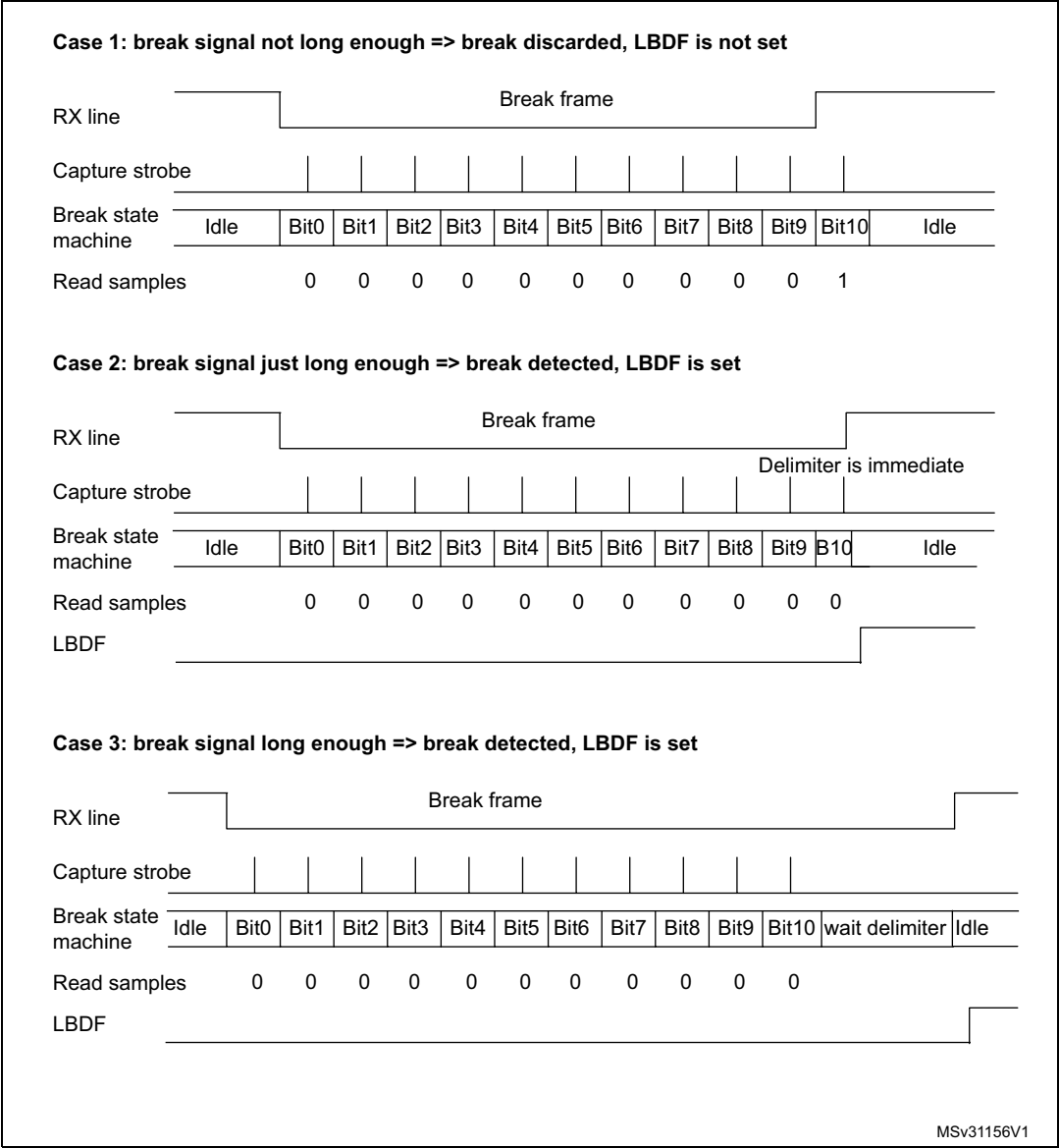
Figure 288. Break detection in LIN mode (11-bit break length - LBDL bit is set)
