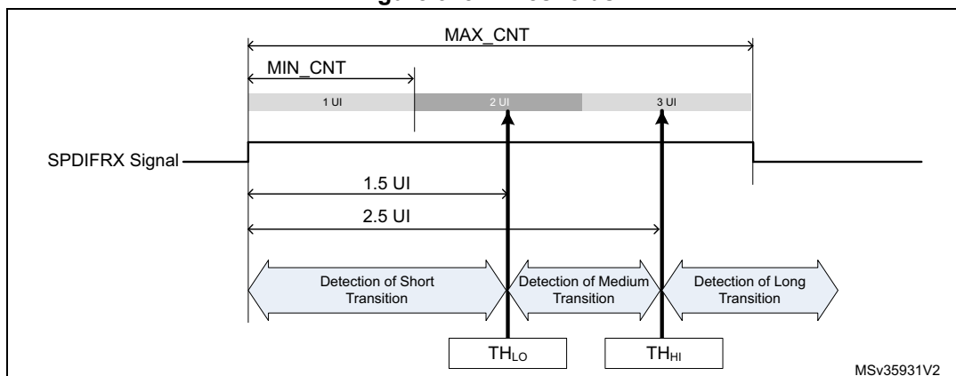
Figure 345. Thresholds
