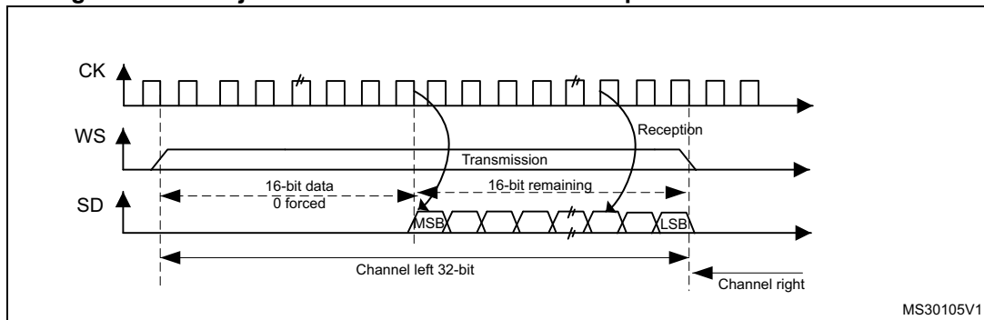
Figure 332. LSB justified 16-bit extended to 32-bit packet frame with CPOL = 0
