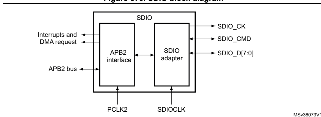
Figure 375. SDIO block diagram
