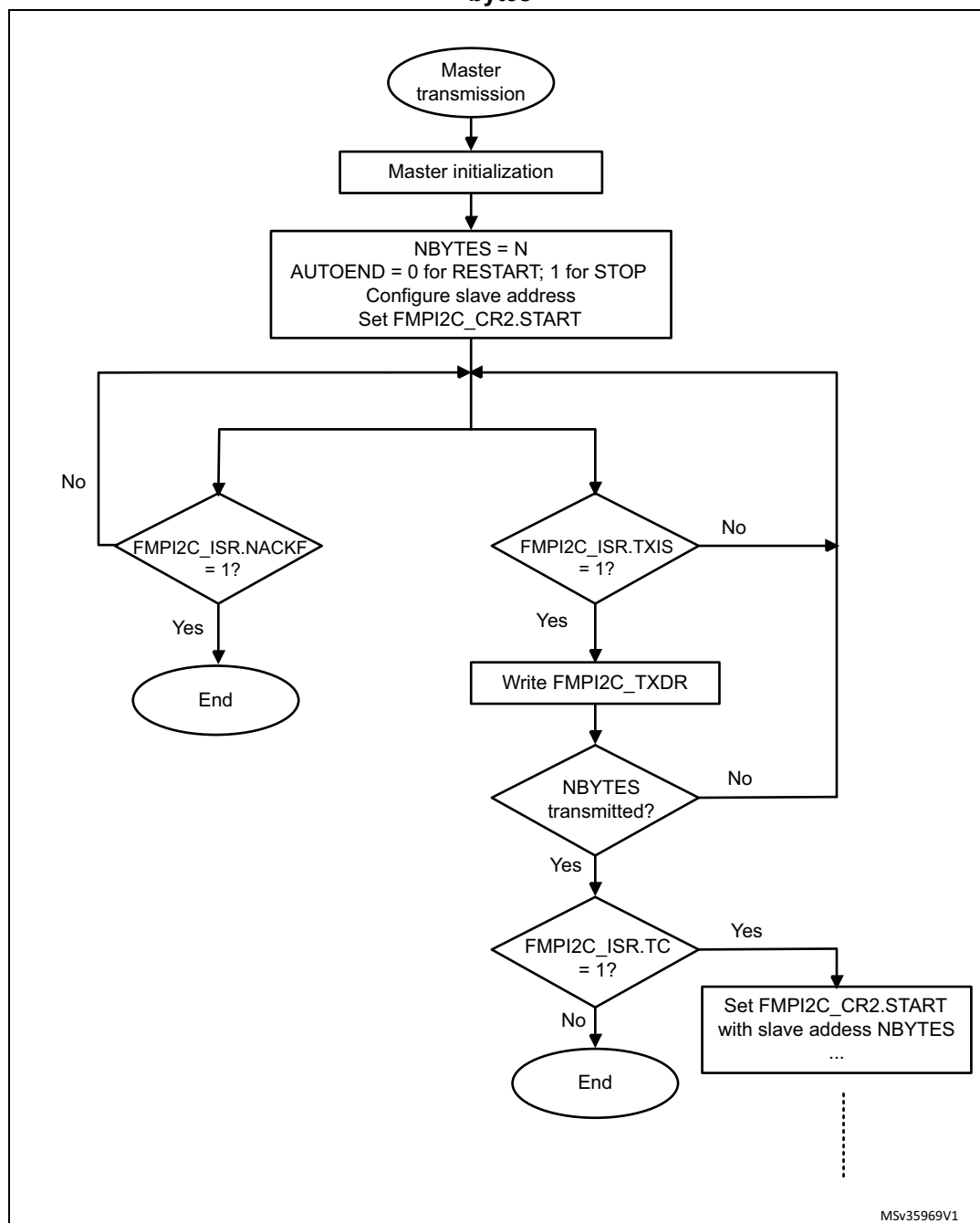
Figure 258. Transfer sequence flowchart for FMPI2C master transmitter for N \leq 255 bytes
