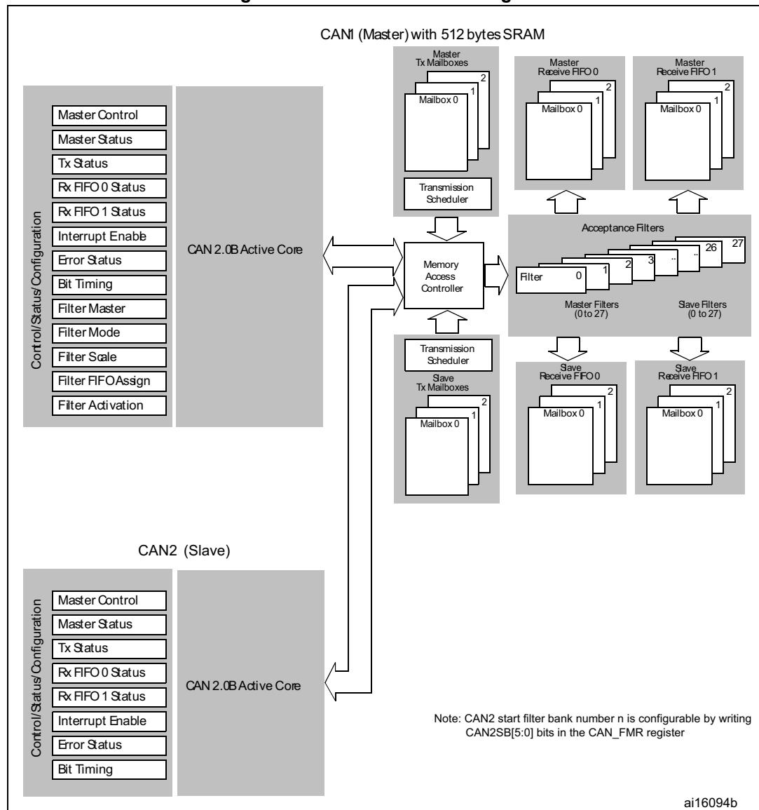
Figure 385. Dual-CAN block diagram
