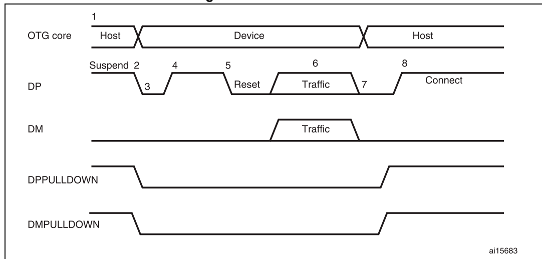
Figure 430. A-device HNP
