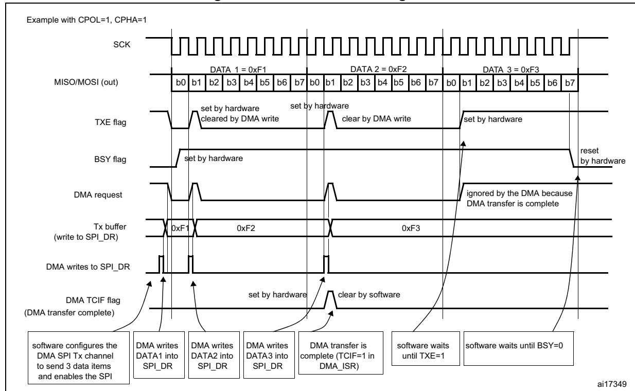
Figure 314. Transmission using DMA
