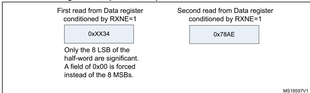
Figure 331. Operations required to receive 0x3478AE
