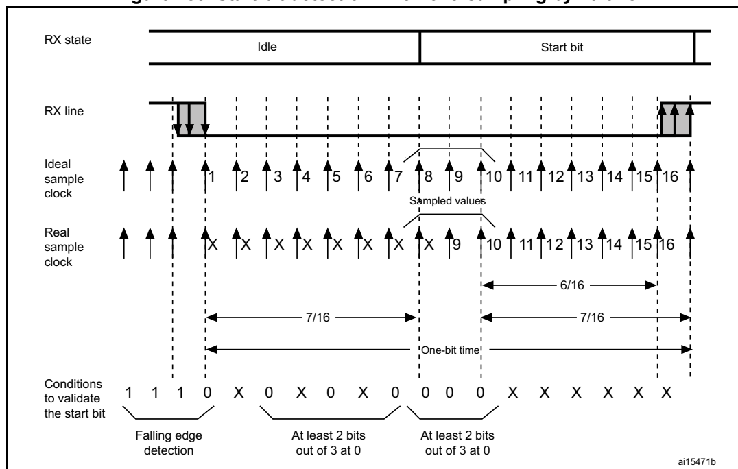
Figure 283. Start bit detection when oversampling by 16 or 8
