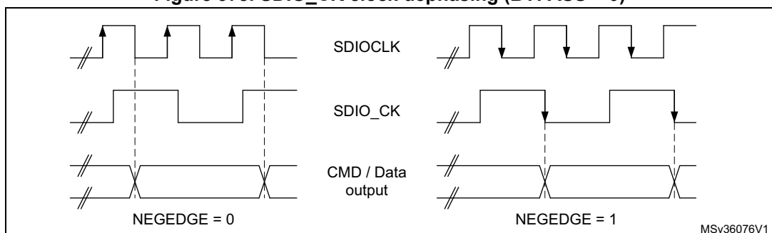
Figure 378. SDIO_CK clock dephasing (BYPASS = 0)
