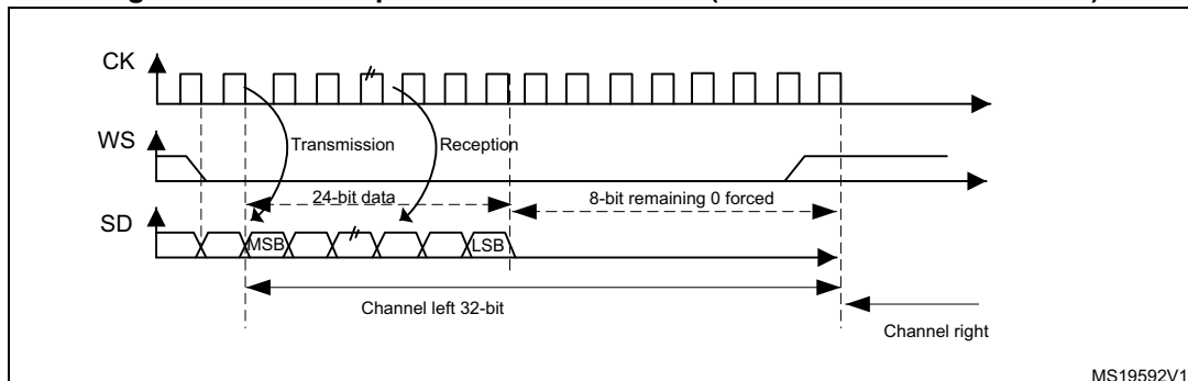
Figure 320. I 2 S Philips standard waveforms (24-bit frame with CPOL = 0)
