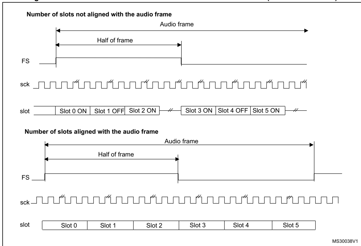
Figure 356. FS role is start of frame + channel side identification (FSDEF = TRIS = 1)
