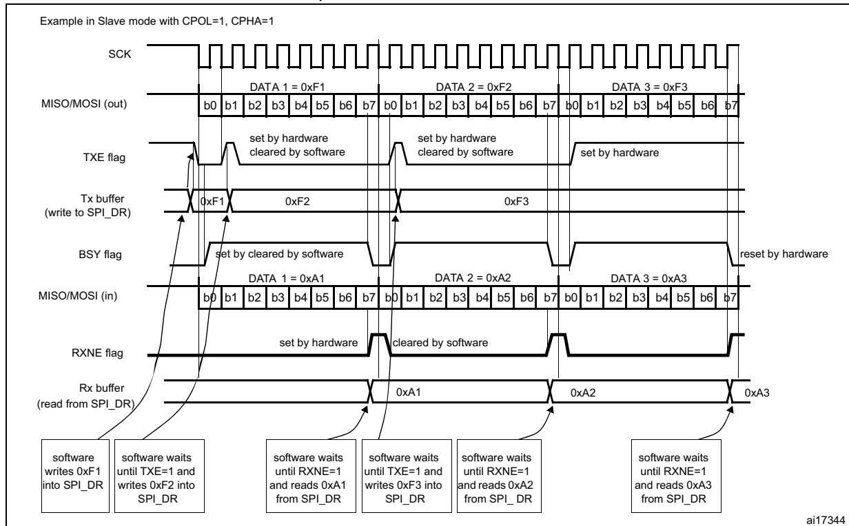
Figure 313. TXE/RXNE/BSY behavior in slave / full-duplex mode (BIDIMODE=0, RXONLY=0) in the case of continuous transfers
