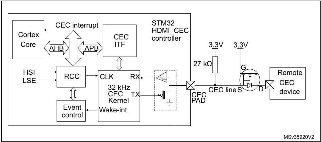
Figure 432. HDMI-CEC block diagram
