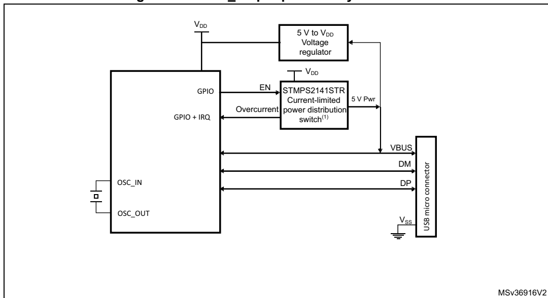
Figure 403. USB_FS peripheral-only connection
