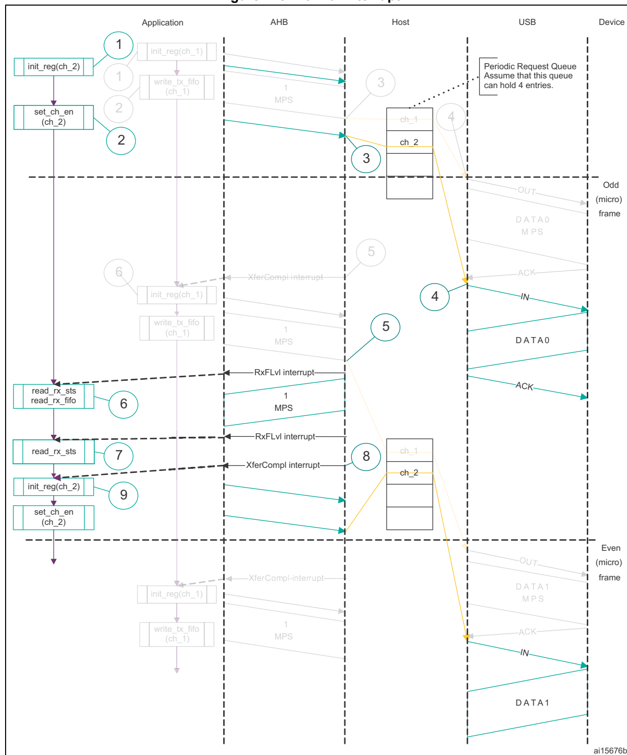
Figure 415. Normal interrupt IN
