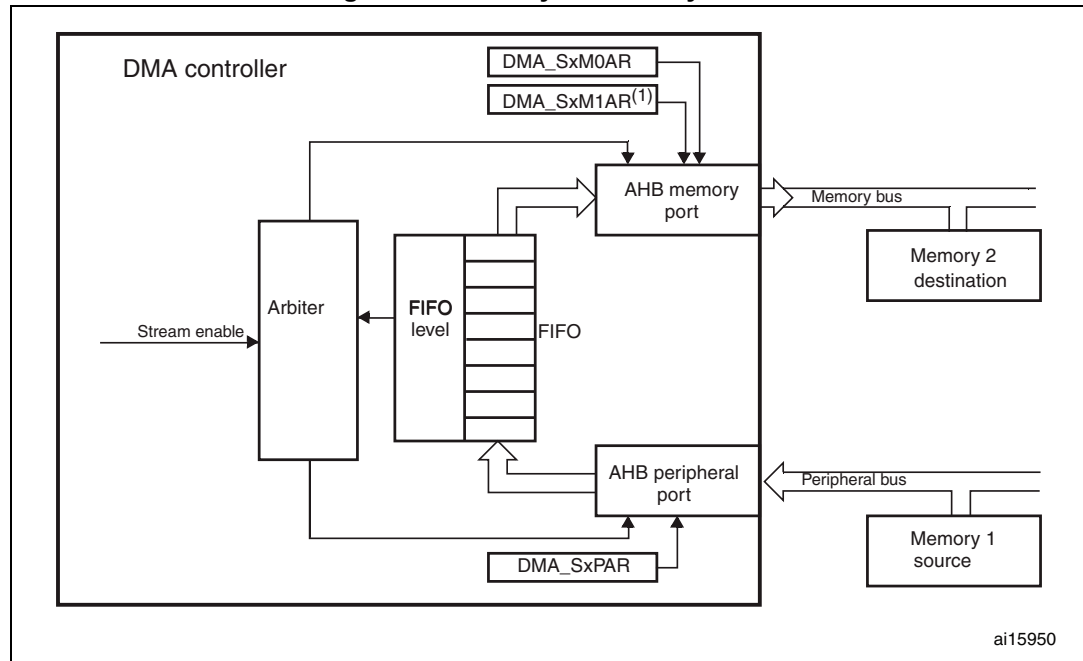
Figure 28. Memory-to-memory mode
