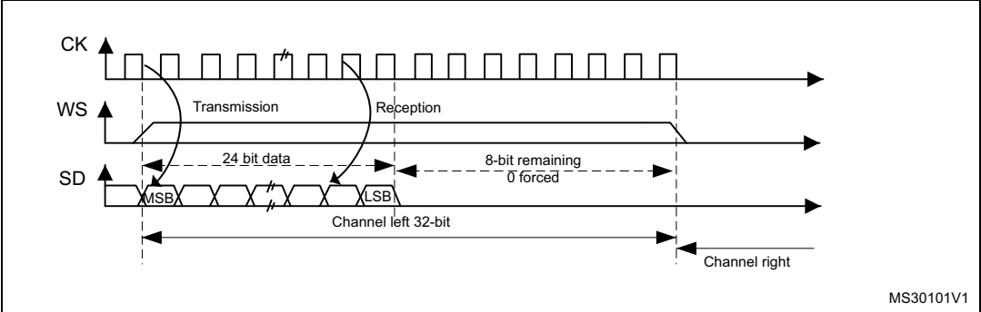
Figure 326. MSB justified 24-bit frame length with CPOL = 0
