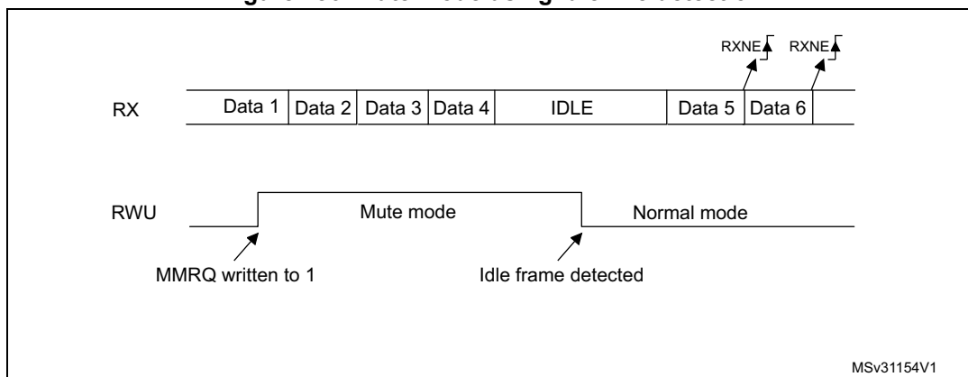
Figure 286. Mute mode using Idle line detection
