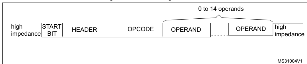
Figure 433. Message structure
