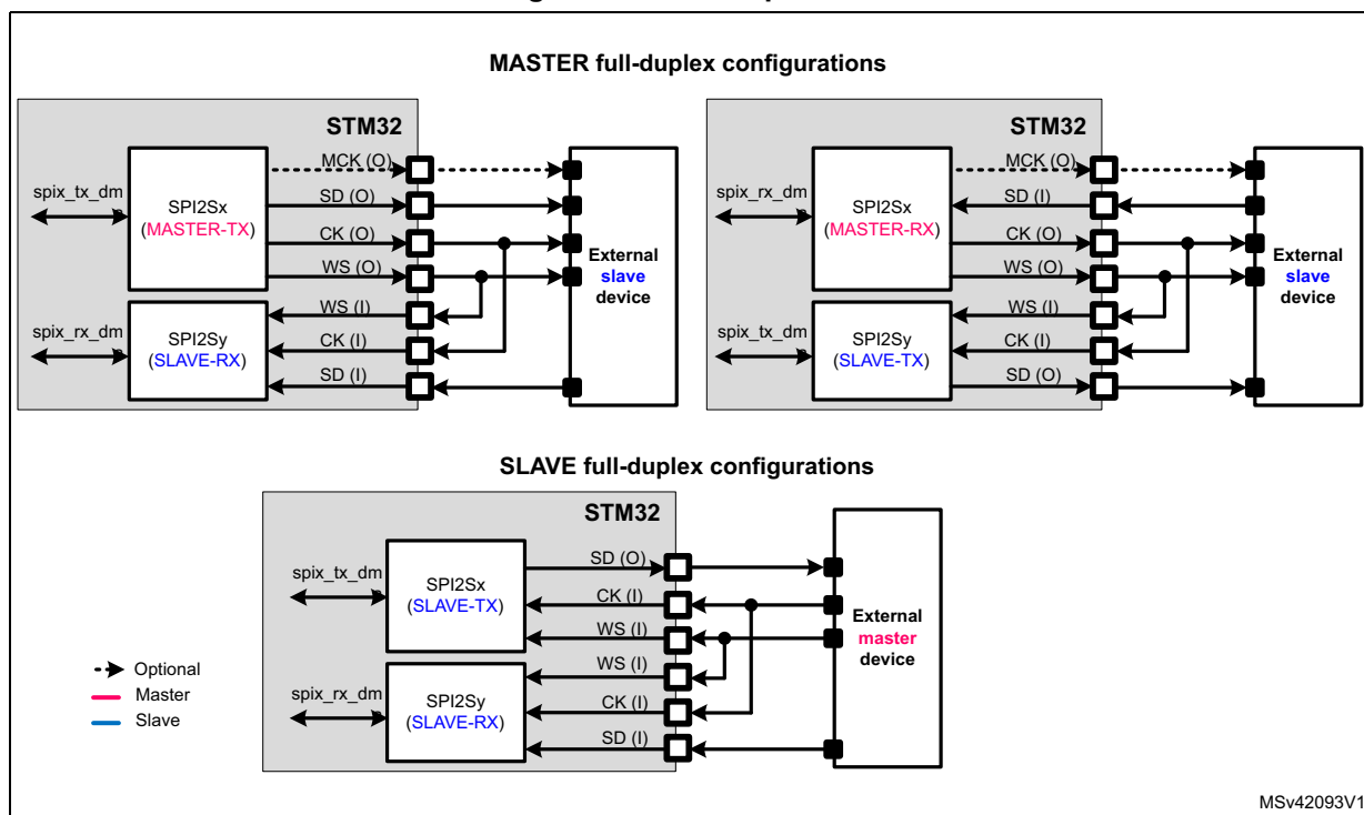
Figure 318. Full-duplex communication
