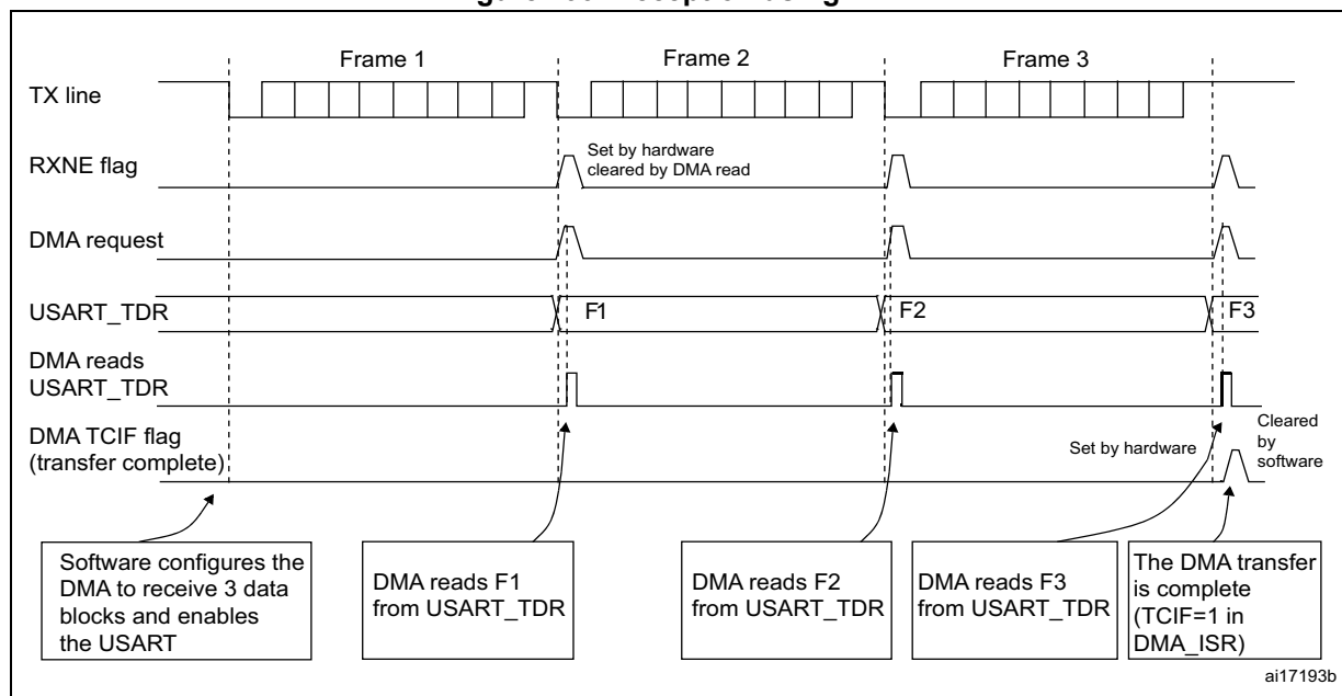
Figure 299. Reception using DMA
