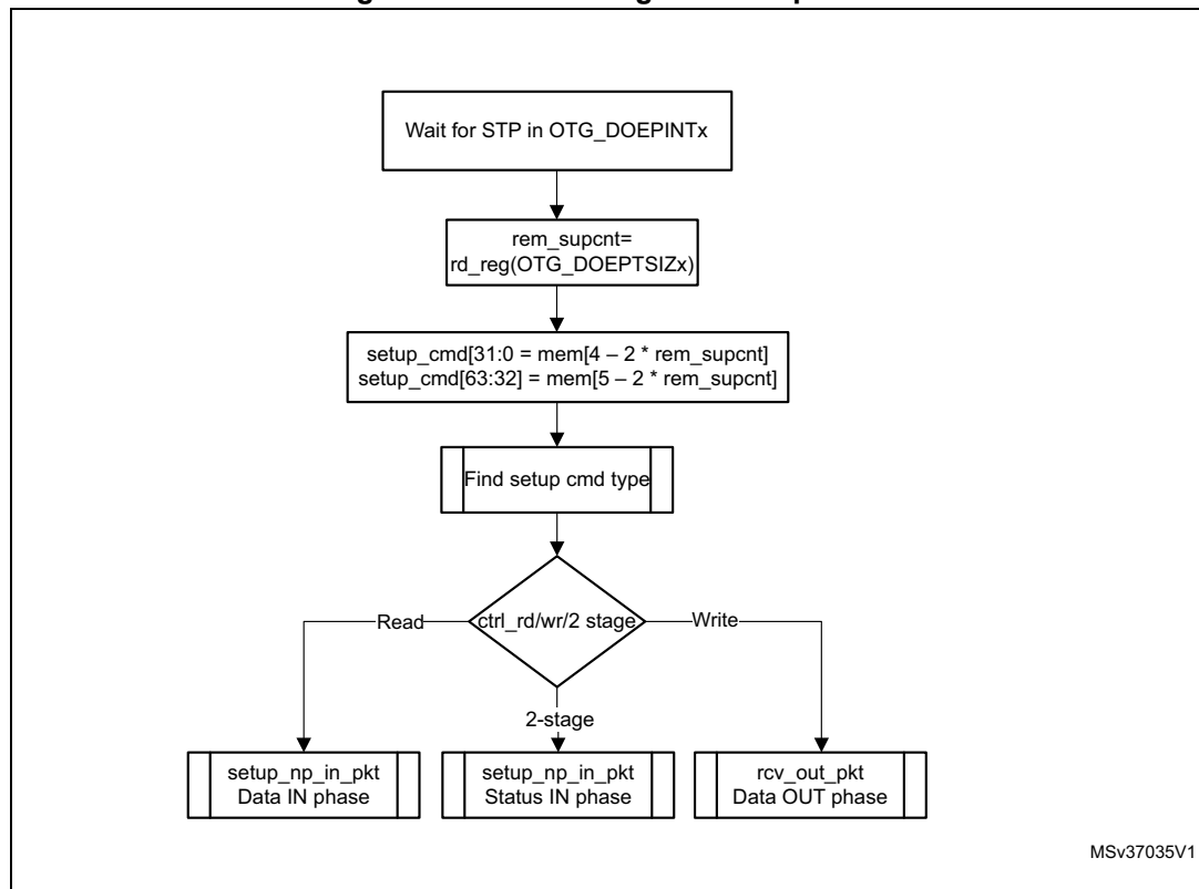
Figure 425. Processing a SETUP packet
