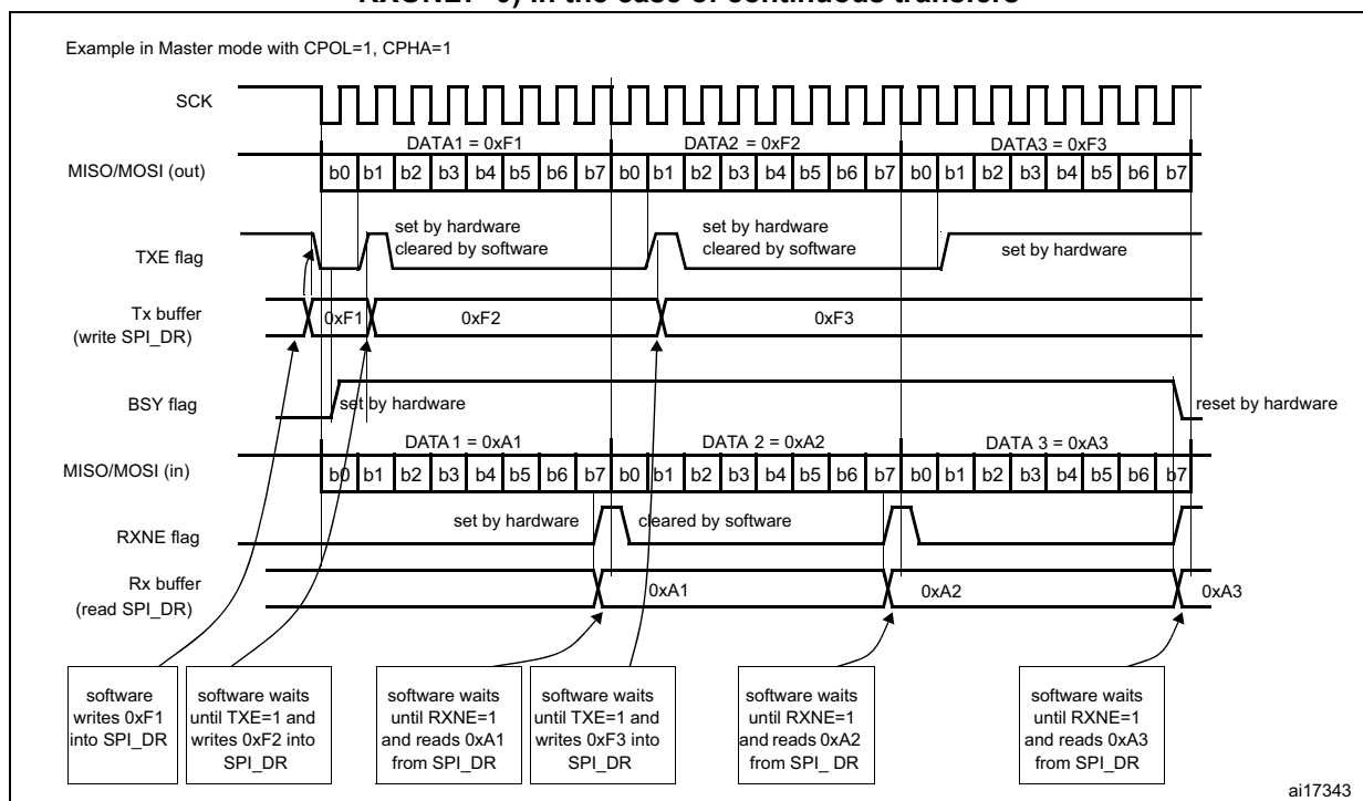
Figure 312. TXE/RXNE/BSY behavior in master / full-duplex mode (BIDIMODE=0, RXONLY=0) in the case of continuous transfers
