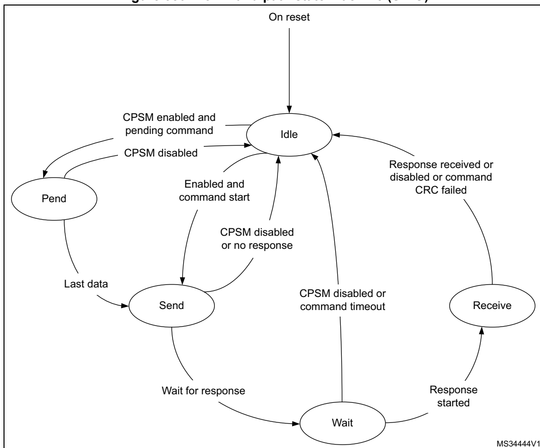
Figure 380. Command path state machine (SDIO)
