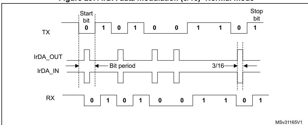
Figure 297. IrDA data modulation (3/16) -Normal mode
