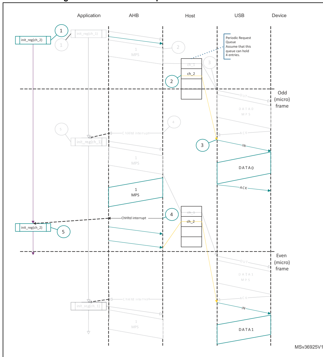
Figure 421. Normal interrupt IN transactions - DMA mode
