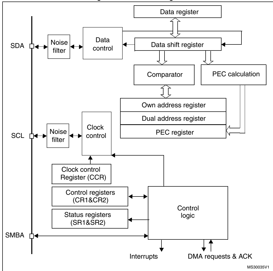
Figure 273. I 2 C block diagram
