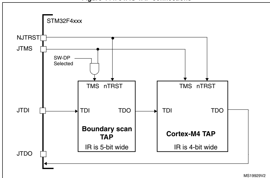
Figure 444. JTAG TAP connections
