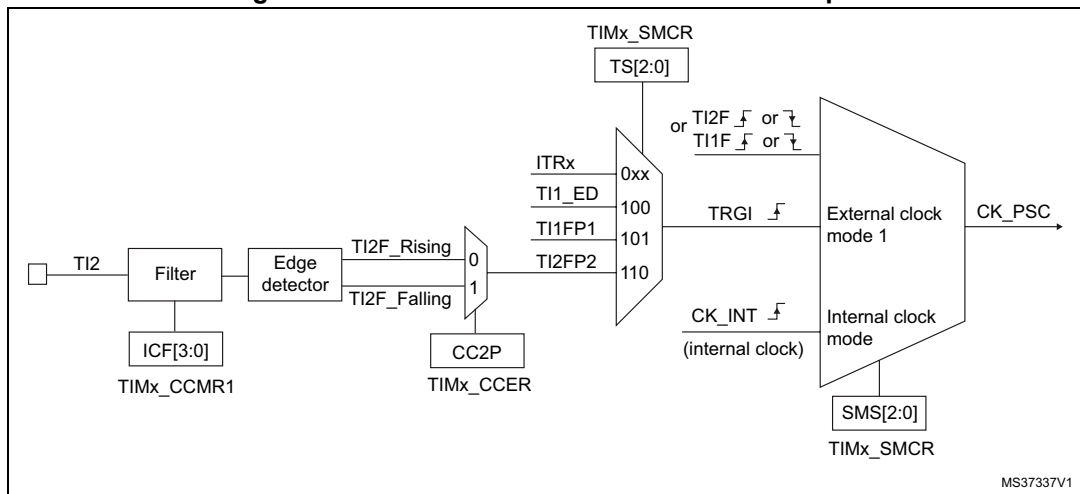
Figure 215. TI2 external clock connection example
