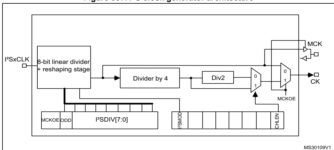
Figure 337. I 2 S clock generator architecture
