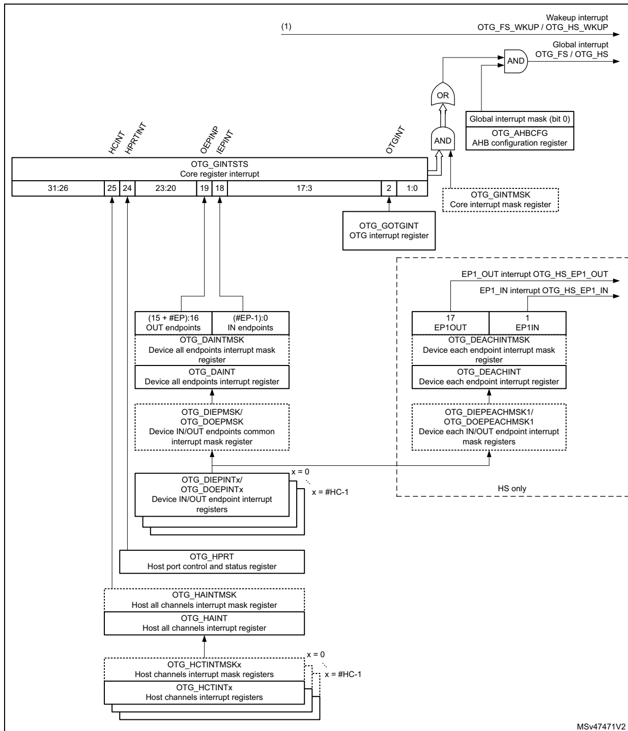
Figure 409. Interrupt hierarchy
