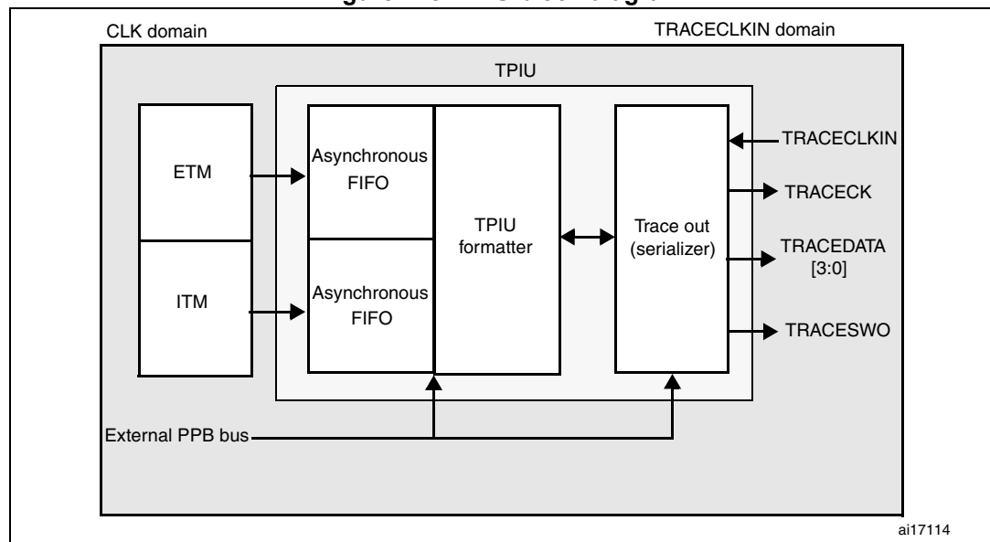
Figure 445. TPIU block diagram
