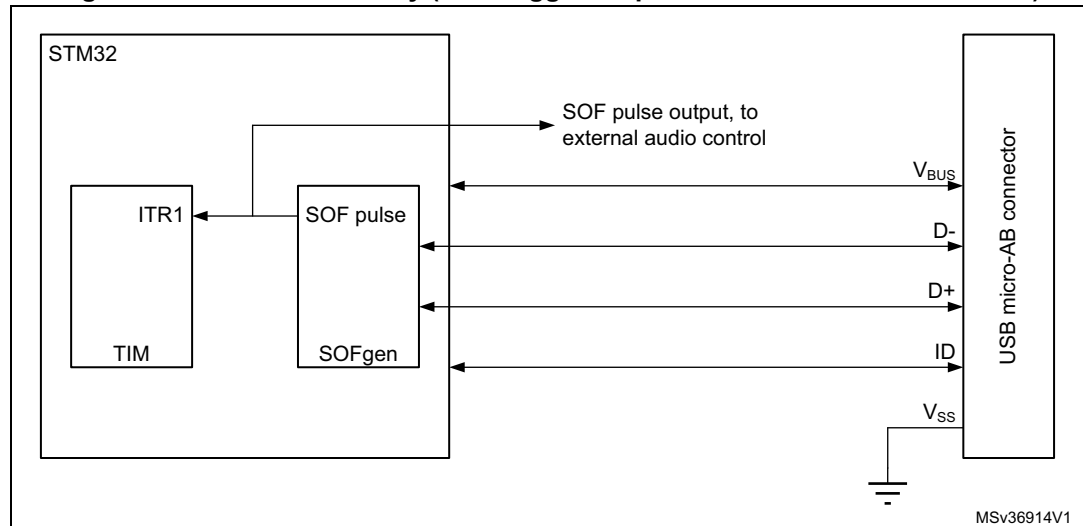
Figure 405. SOF connectivity (SOF trigger output to TIM and ITR1 connection)
