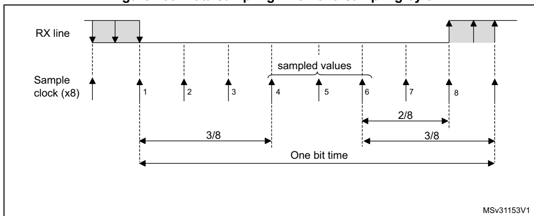
Figure 285. Data sampling when oversampling by 8
