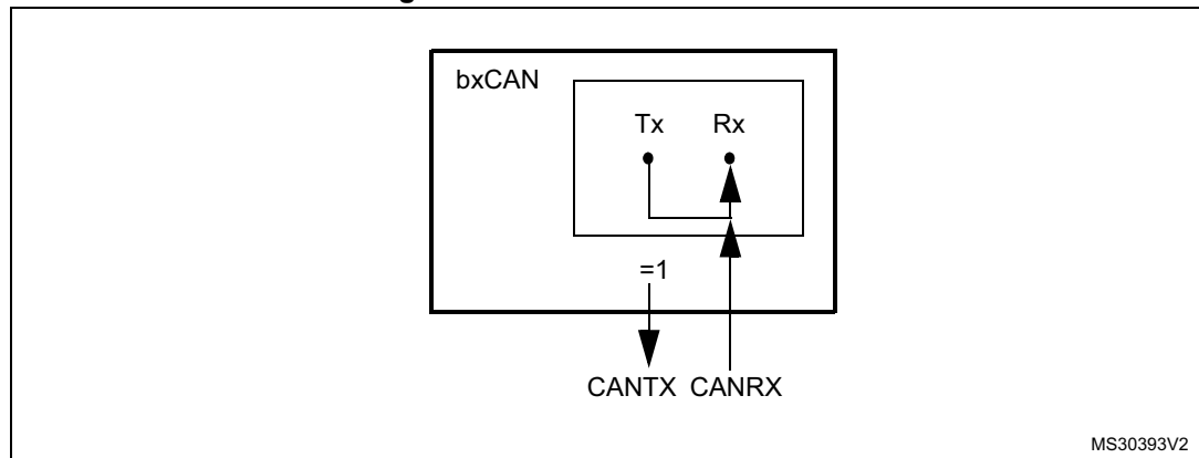
Figure 387. bxCAN in silent mode
