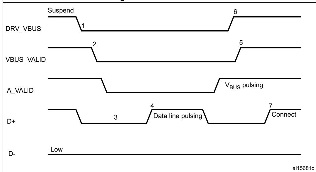
Figure 428. A-device SRP
