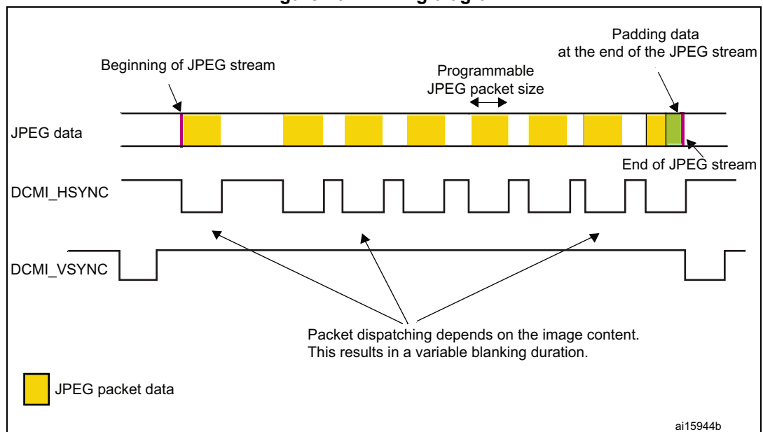
Figure 104. Timing diagram
