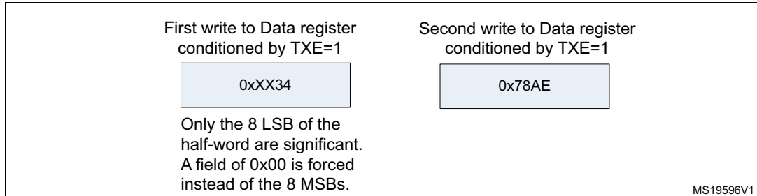
Figure 330. Operations required to transmit 0x3478AE
