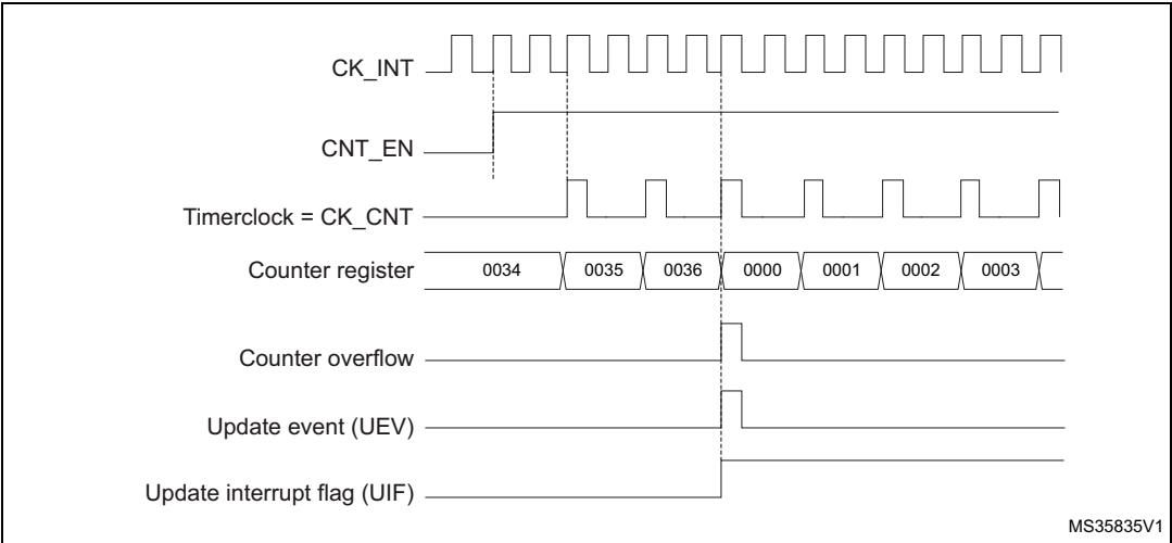
Figure 231. Counter timing diagram, internal clock divided by 2
