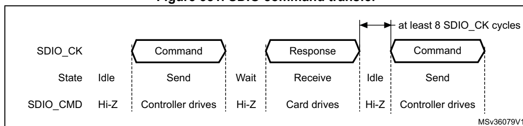
Figure 381. SDIO command transfer
