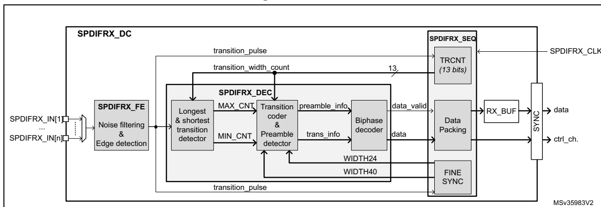
Figure 343. SPDIFRX decoder
