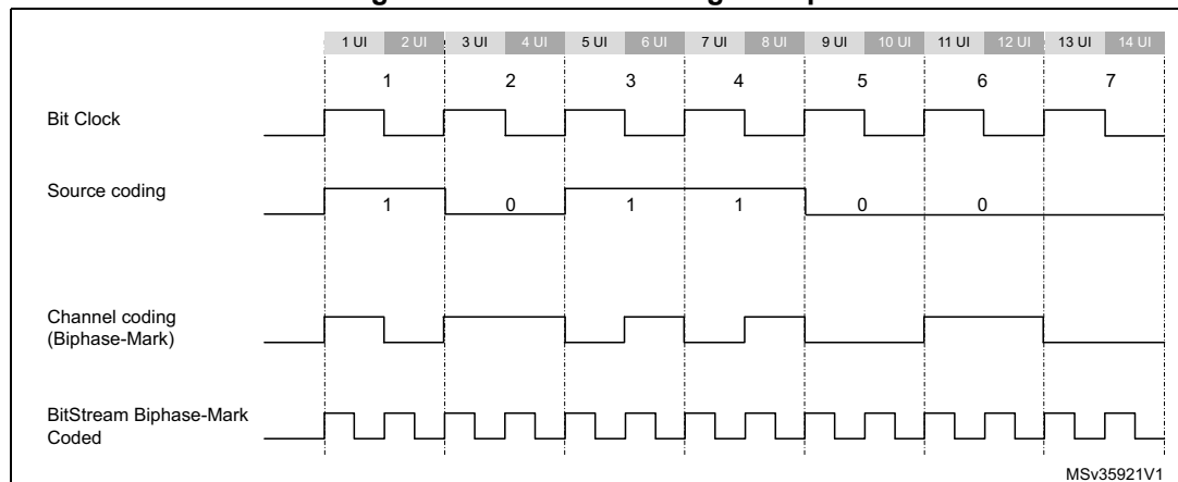
Figure 342. Channel coding example
