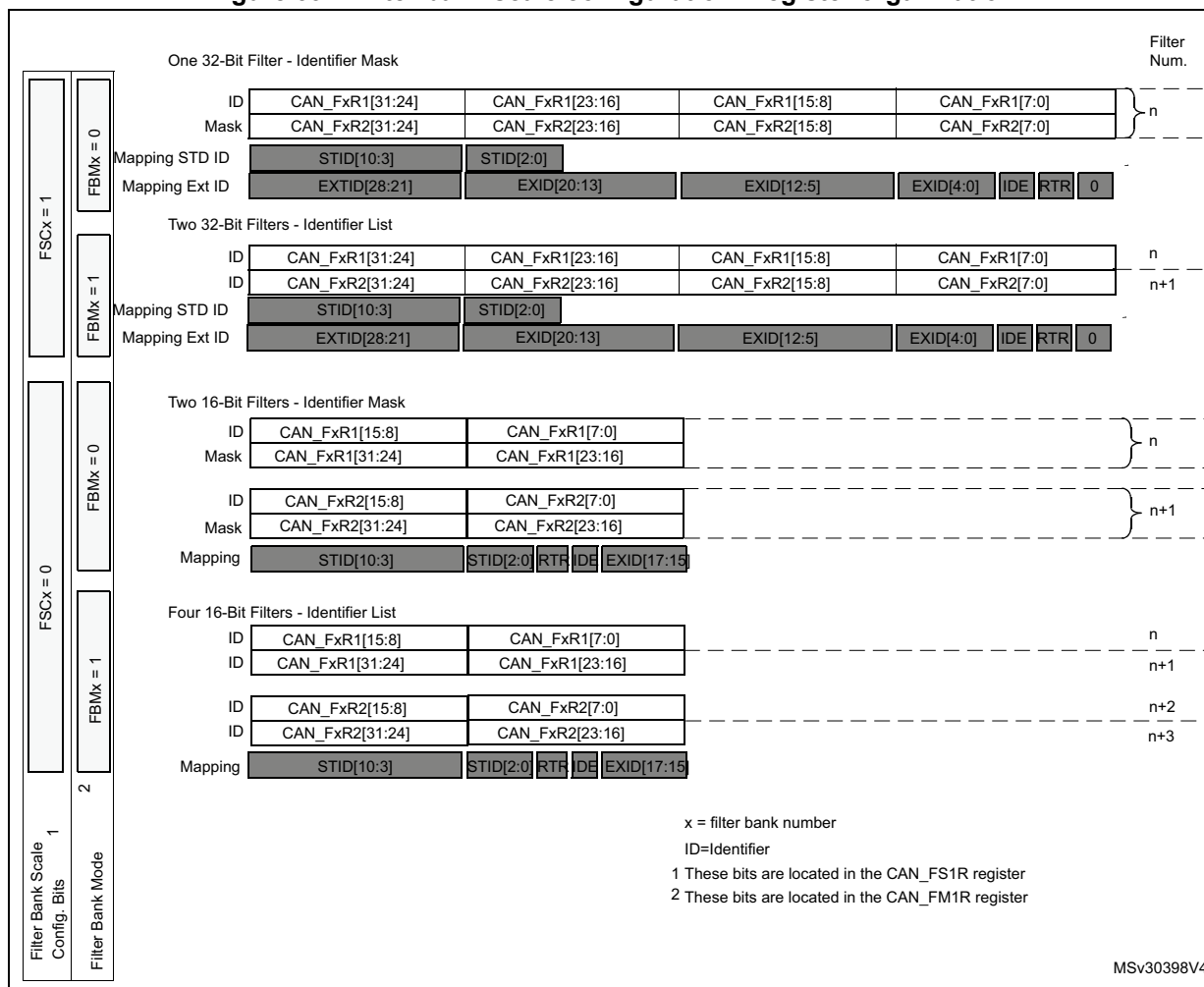
Figure 392. Filter bank scale configuration - register organization
