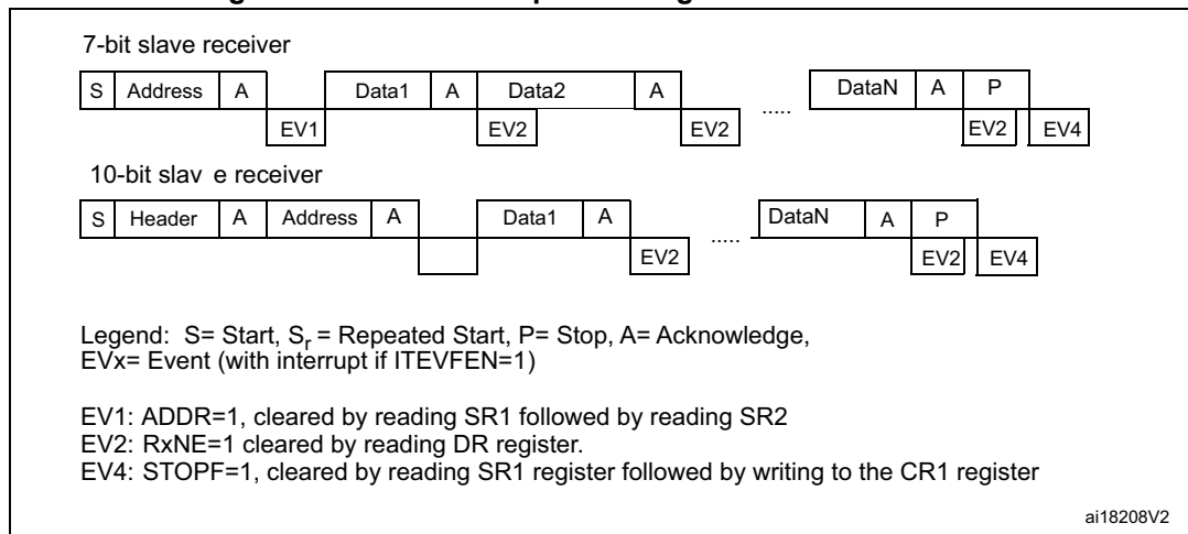
Figure 275. Transfer sequence diagram for slave receiver
