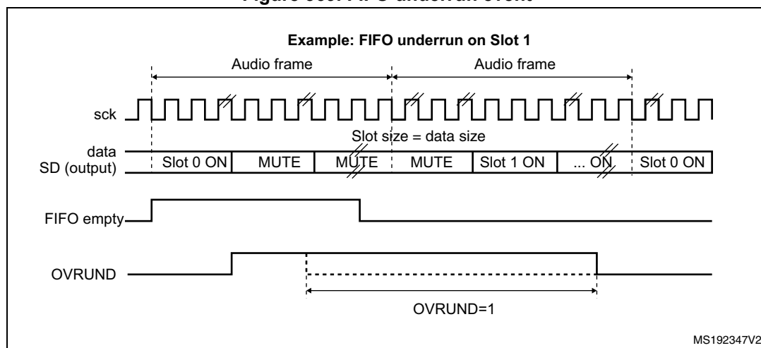
Figure 369. FIFO underrun event
