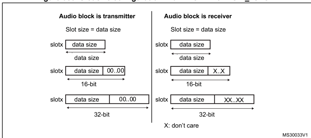
Figure 358. Slot size configuration with FBOFF = 0 in SAI_xSLOTR
