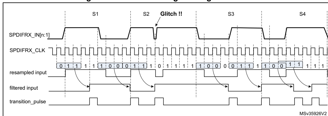
Figure 344. Noise filtering and edge detection
