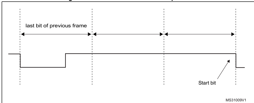
Figure 438. SFT of three nominal bit periods
