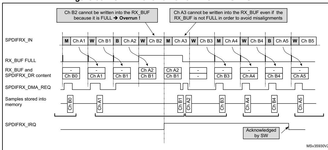
Figure 352. S/PDIF overrun error when RXSTEO = 1
