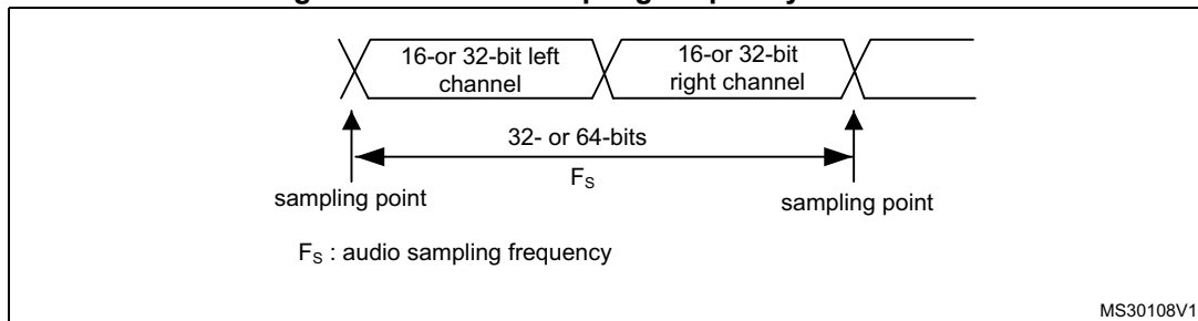
Figure 336. Audio sampling frequency definition
