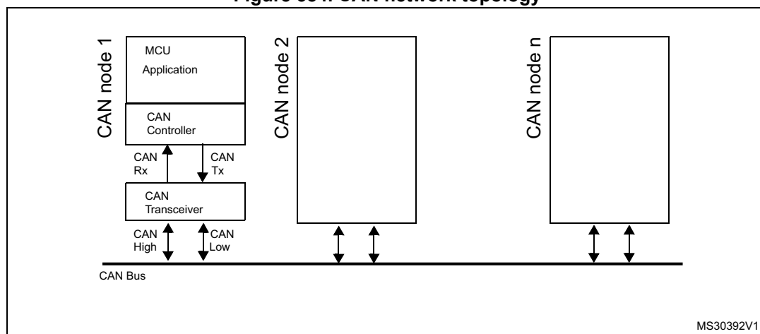
Figure 384. CAN network topology
