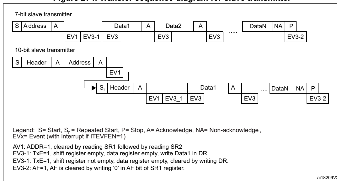
Figure 274. Transfer sequence diagram for slave transmitter
