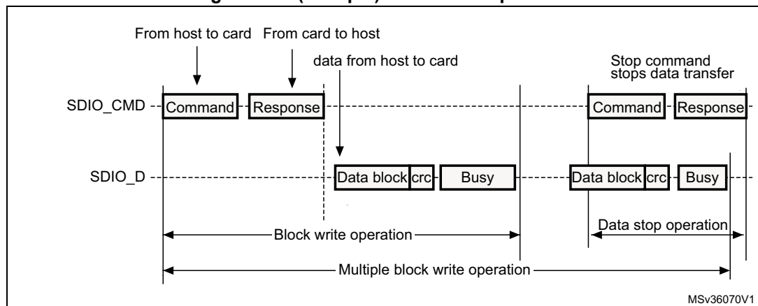
Figure 372. (Multiple) block write operation
