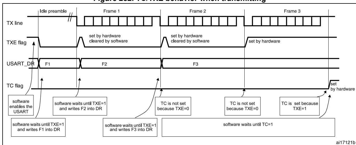
Figure 282. TC/TXE behavior when transmitting
