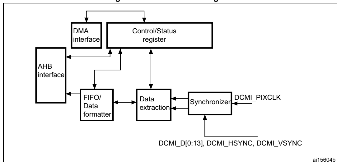
Figure 101. DCMI block diagram
