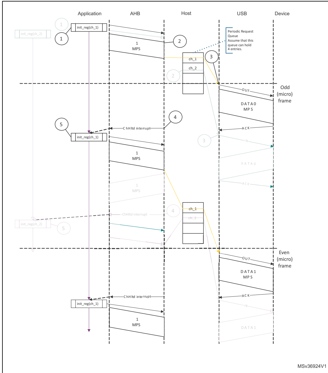
Figure 420. Normal interrupt OUT transactions - DMA mode
