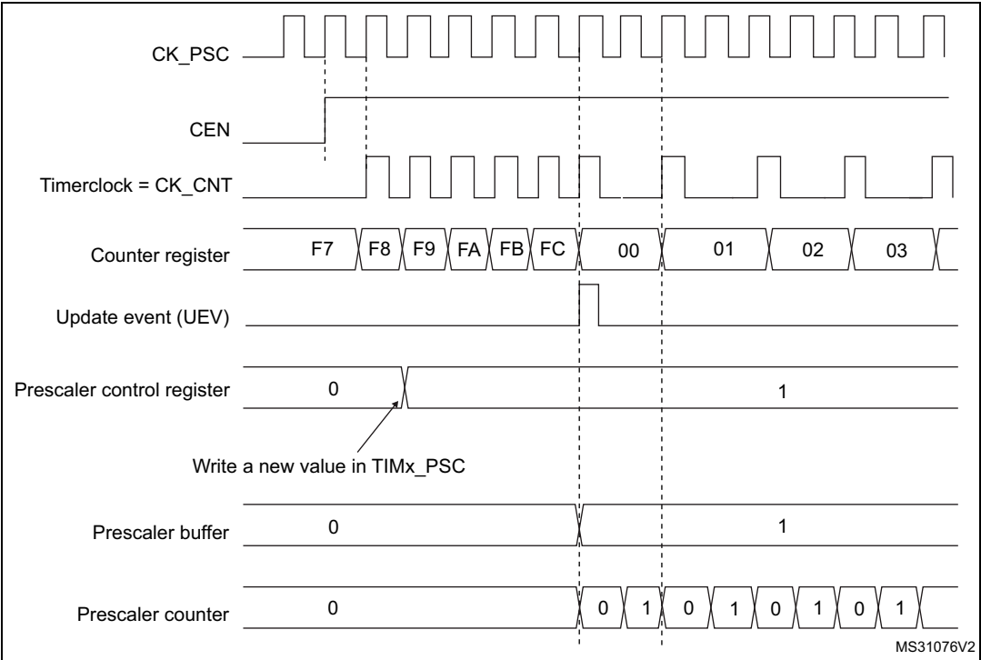
Figure 206. Counter timing diagram with prescaler division change from 1 to 2
