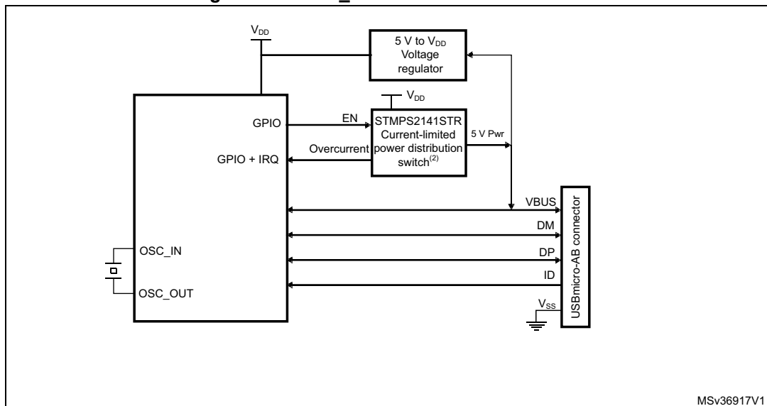
Figure 402. OTG_FS A-B device connection
