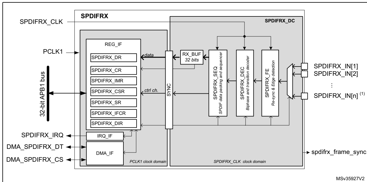
Figure 338. SPDIFRX block diagram
