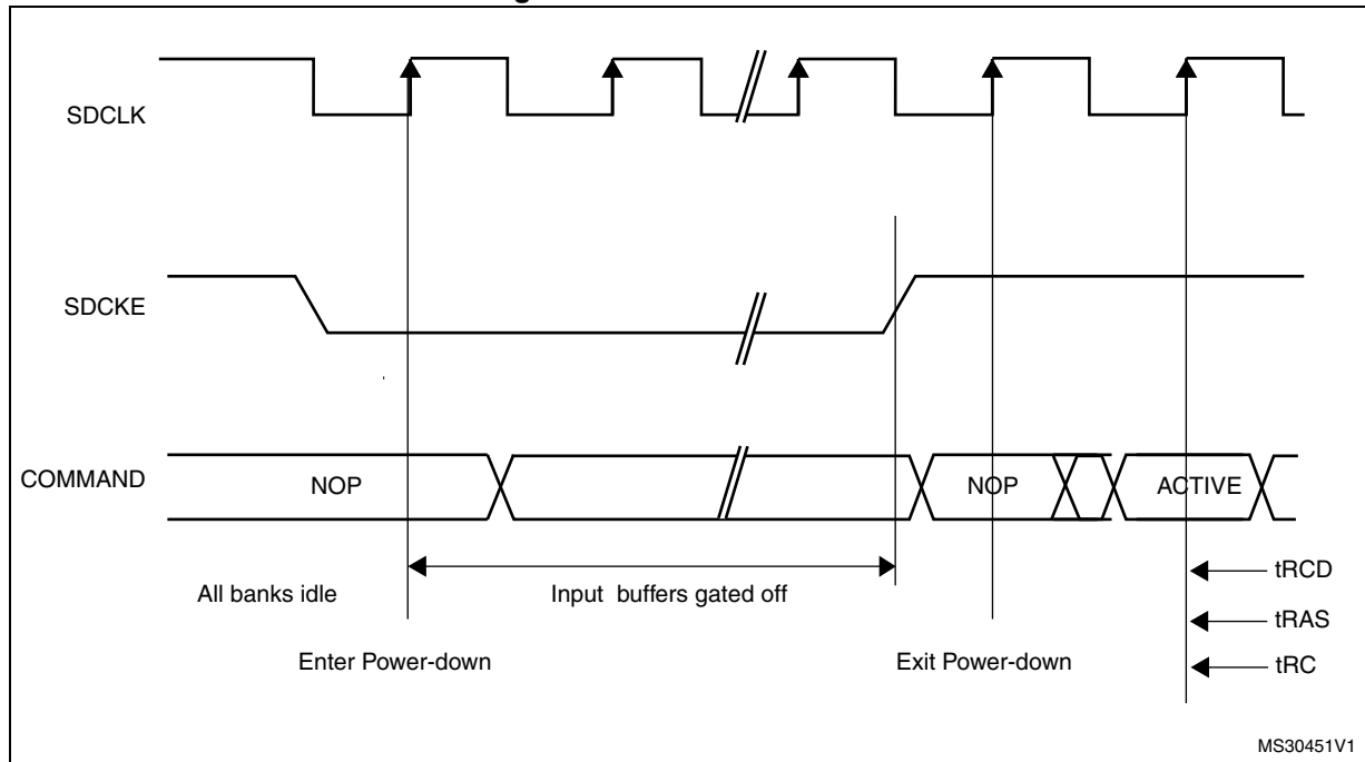
Figure 60. Power-down mode
