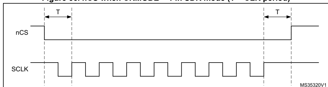
Figure 66. nCS when CKMODE = 1 in SDR mode (T = CLK period)
