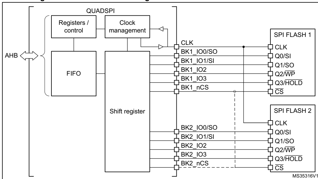
Figure 62. QUADSPI block diagram when dual-flash mode is enabled
