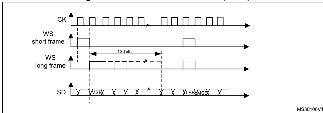
Figure 334. PCM standard waveforms (16-bit)
