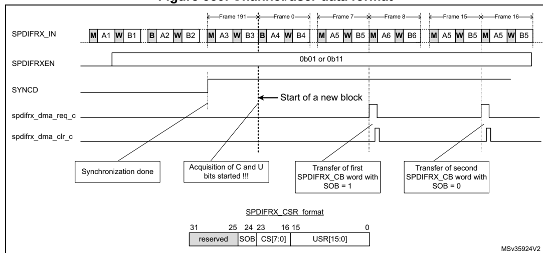
Figure 350. Channel/user data format
