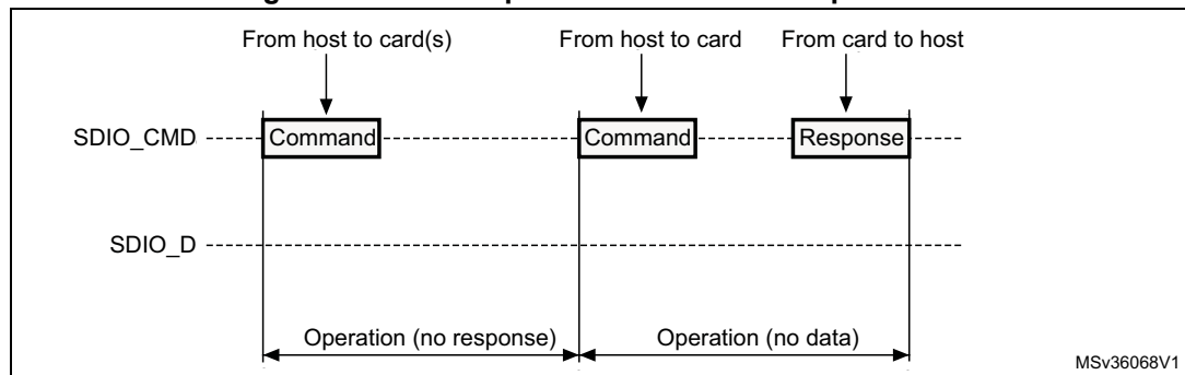
Figure 371. (Multiple) block read operation
