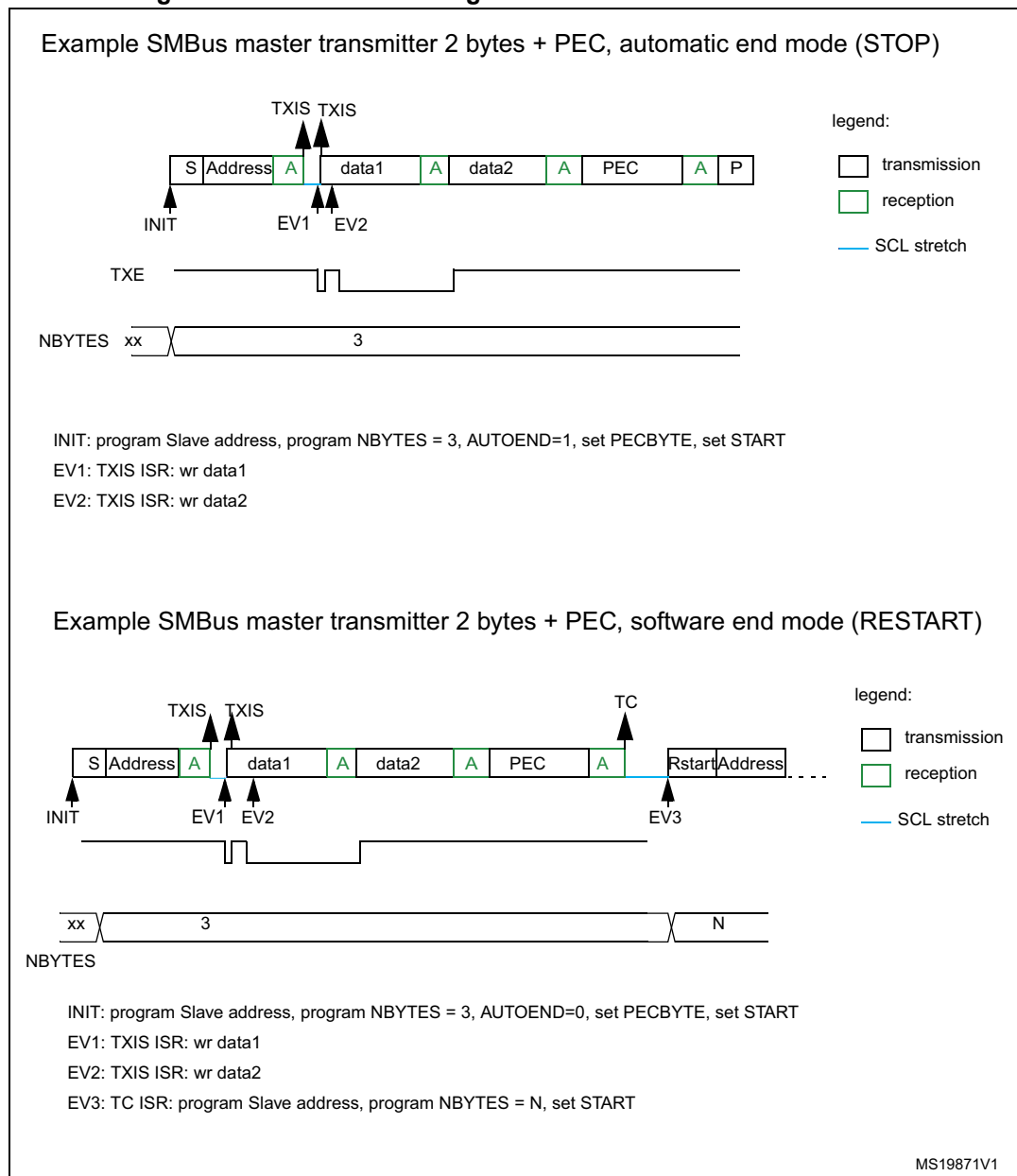
Figure 269. Bus transfer diagrams for SMBus master transmitter
