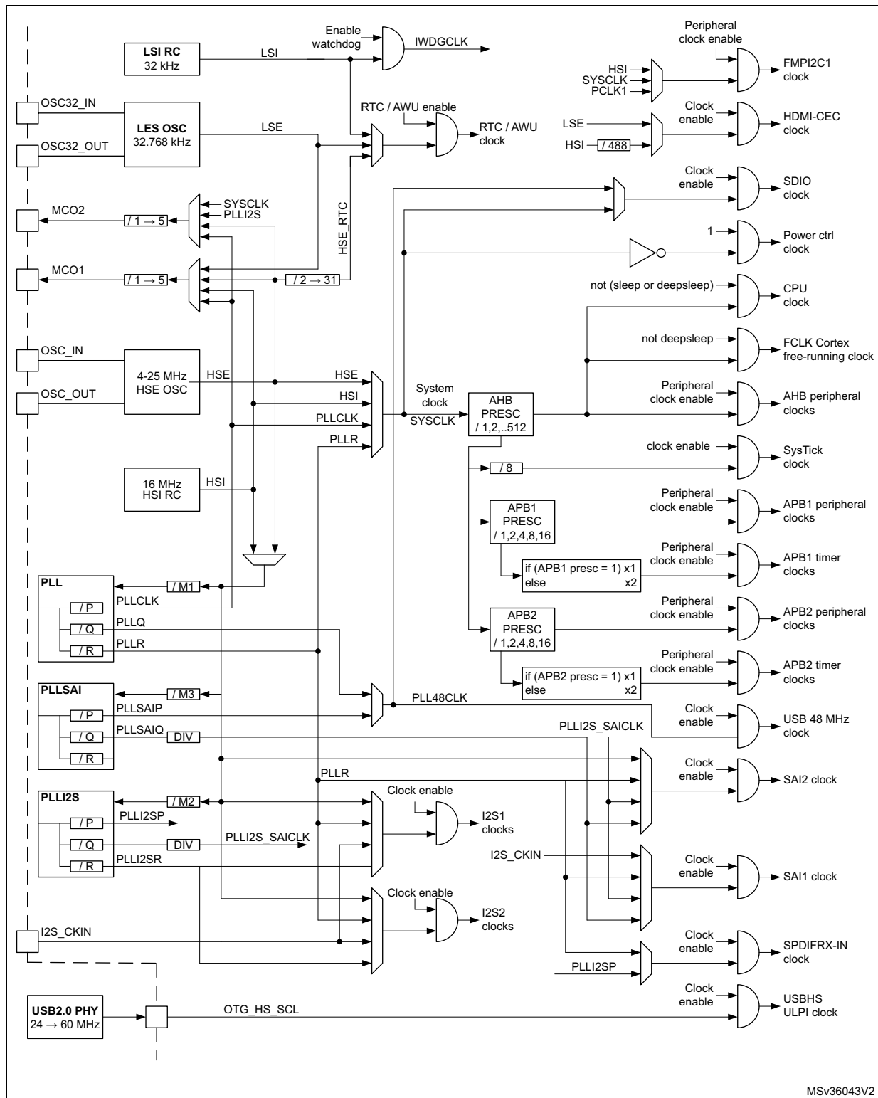
Figure 14. Clock tree
