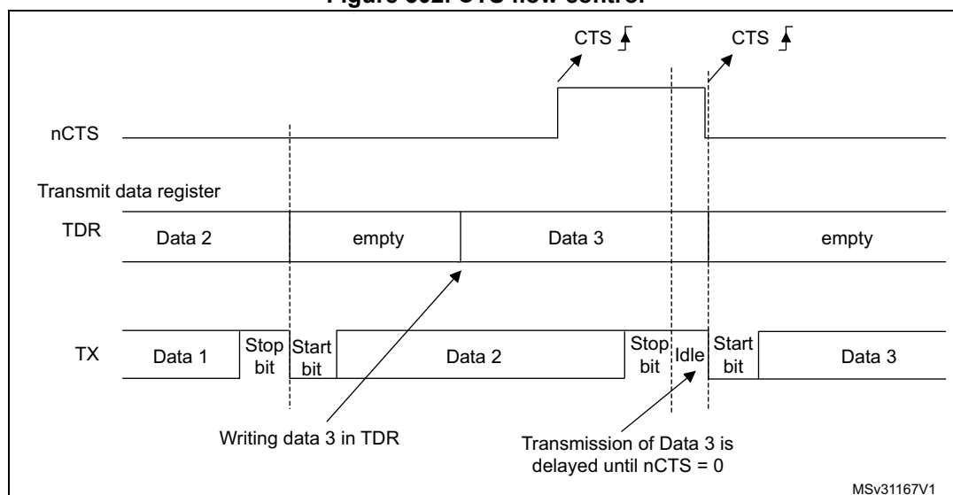
Figure 302. CTS flow control
