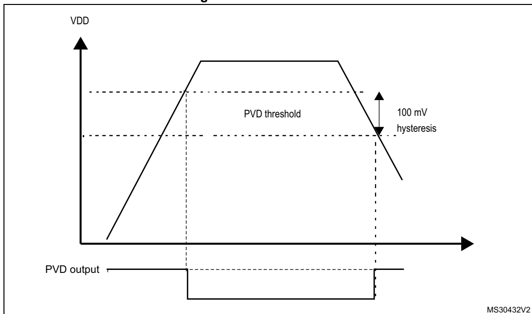
Figure 12. PVD thresholds
