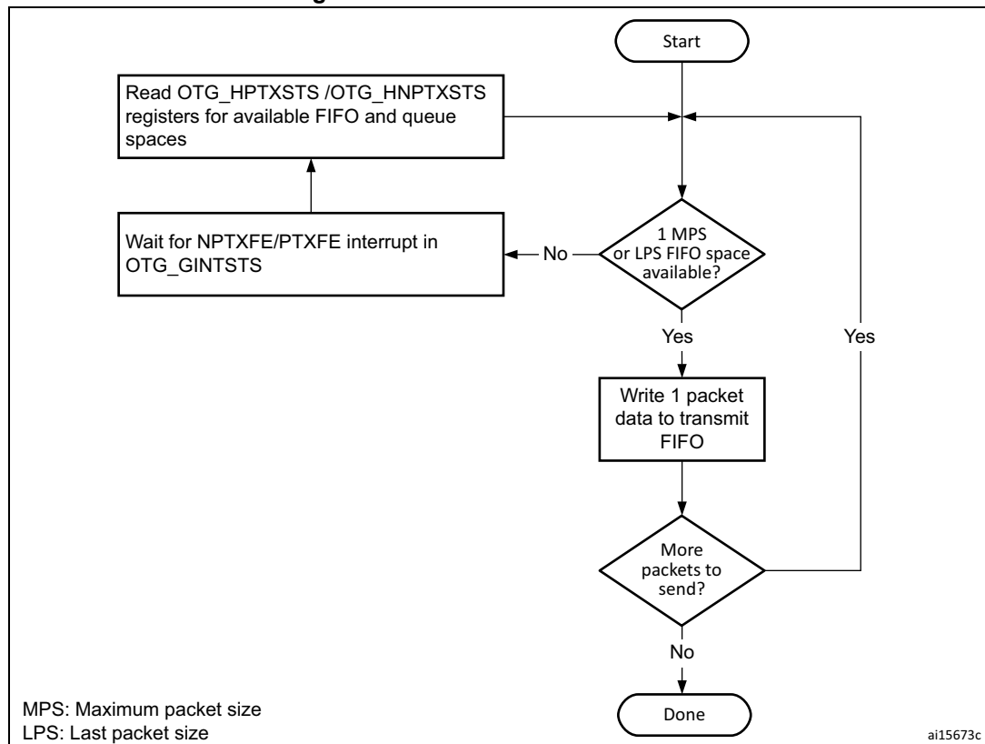
Figure 410. Transmit FIFO write task
