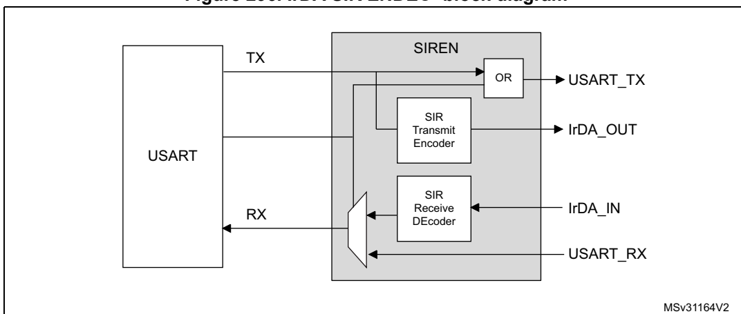
Figure 296. IrDA SIR ENDEC- block diagram
