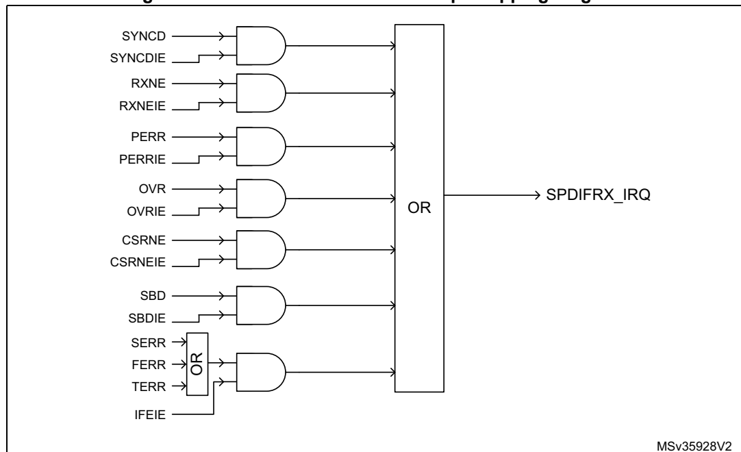
Figure 353. SPDIFRX interface interrupt mapping diagram
