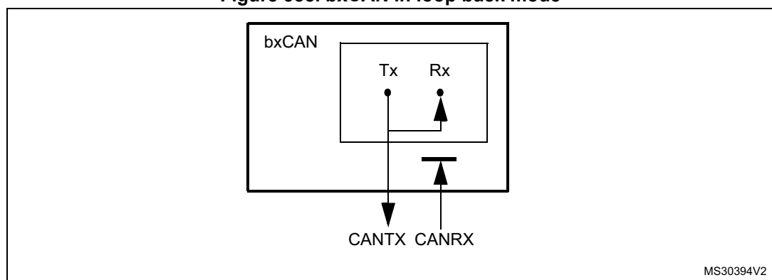
Figure 388. bxCAN in loop back mode
