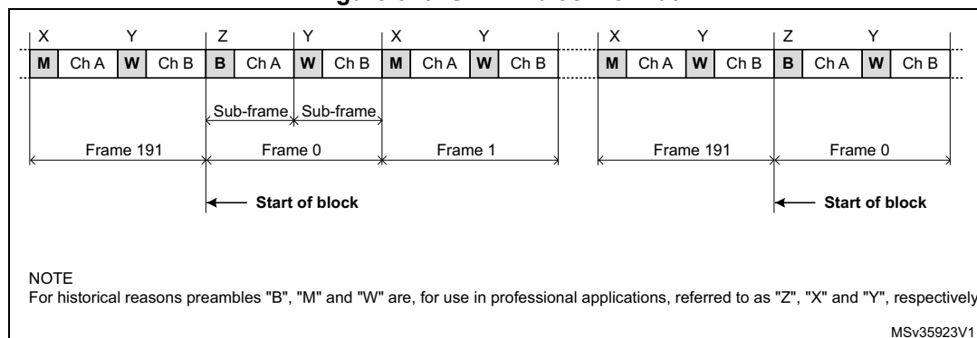
Figure 340. S/PDIF block format
