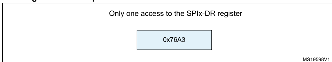
Figure 333. Example of 16-bit data frame extended to 32-bit channel frame
