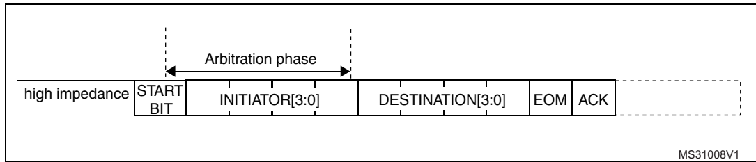
Figure 437. Arbitration phase
