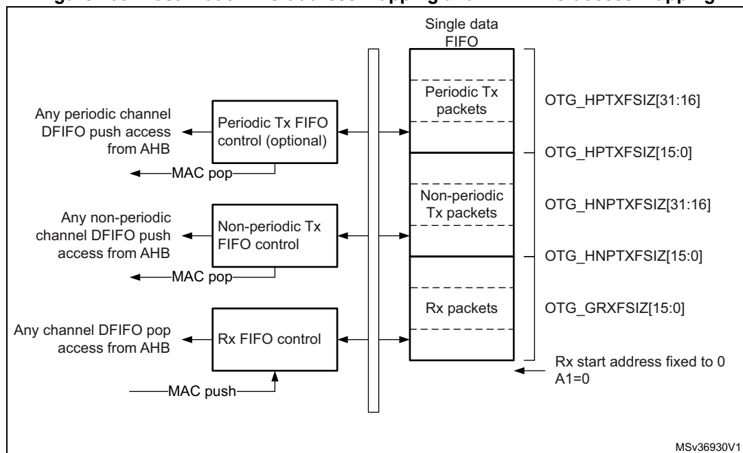
Figure 408. Host-mode FIFO address mapping and AHB FIFO access mapping
