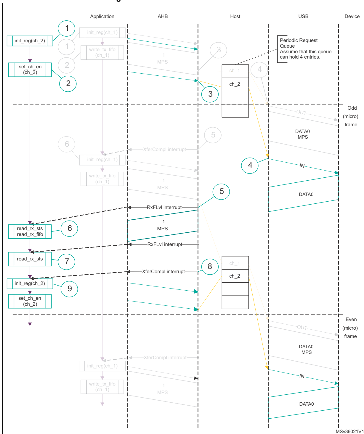
Figure 417. Isochronous IN transactions
