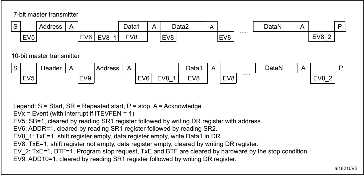
Figure 276. Transfer sequence diagram for master transmitter
