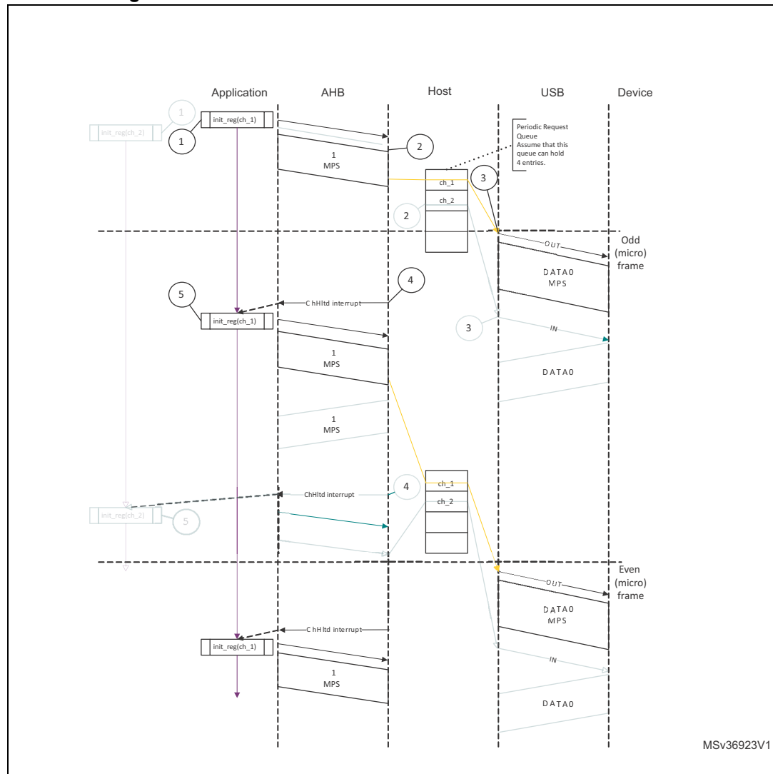
Figure 422. Normal isochronous OUT transaction - DMA mode
