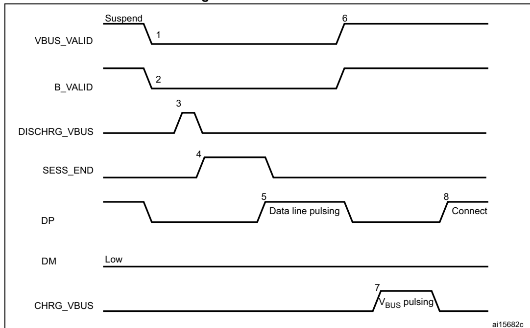
Figure 429. B-device SRP
