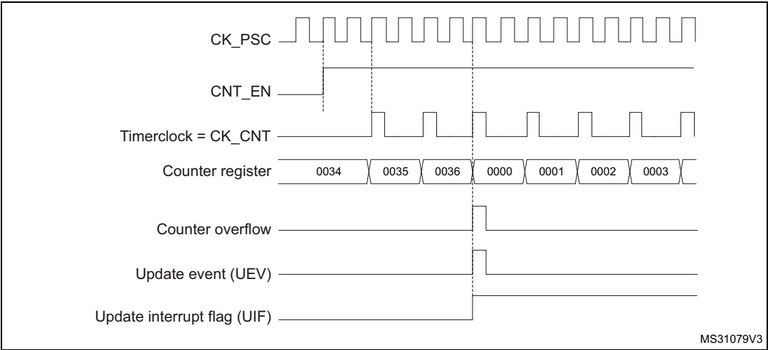
Figure 209. Counter timing diagram, internal clock divided by 2
