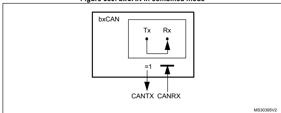
Figure 389. bxCAN in combined mode
