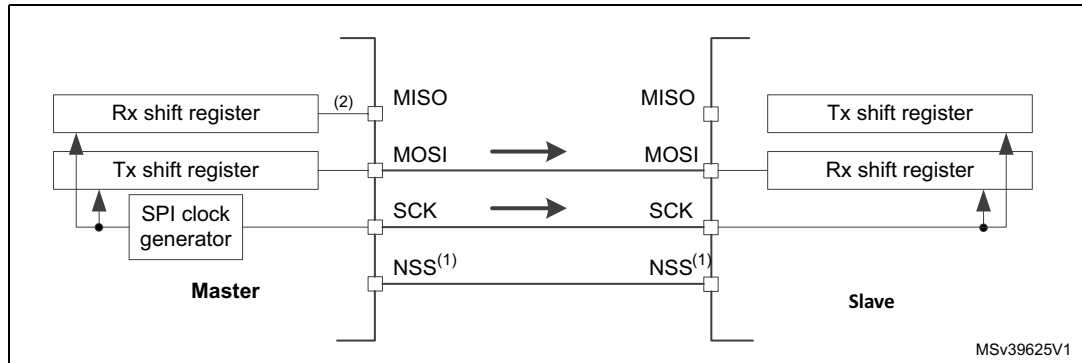
Figure 307. Simplex single master/single slave application (master in transmit-only/ slave in receive-only mode)
