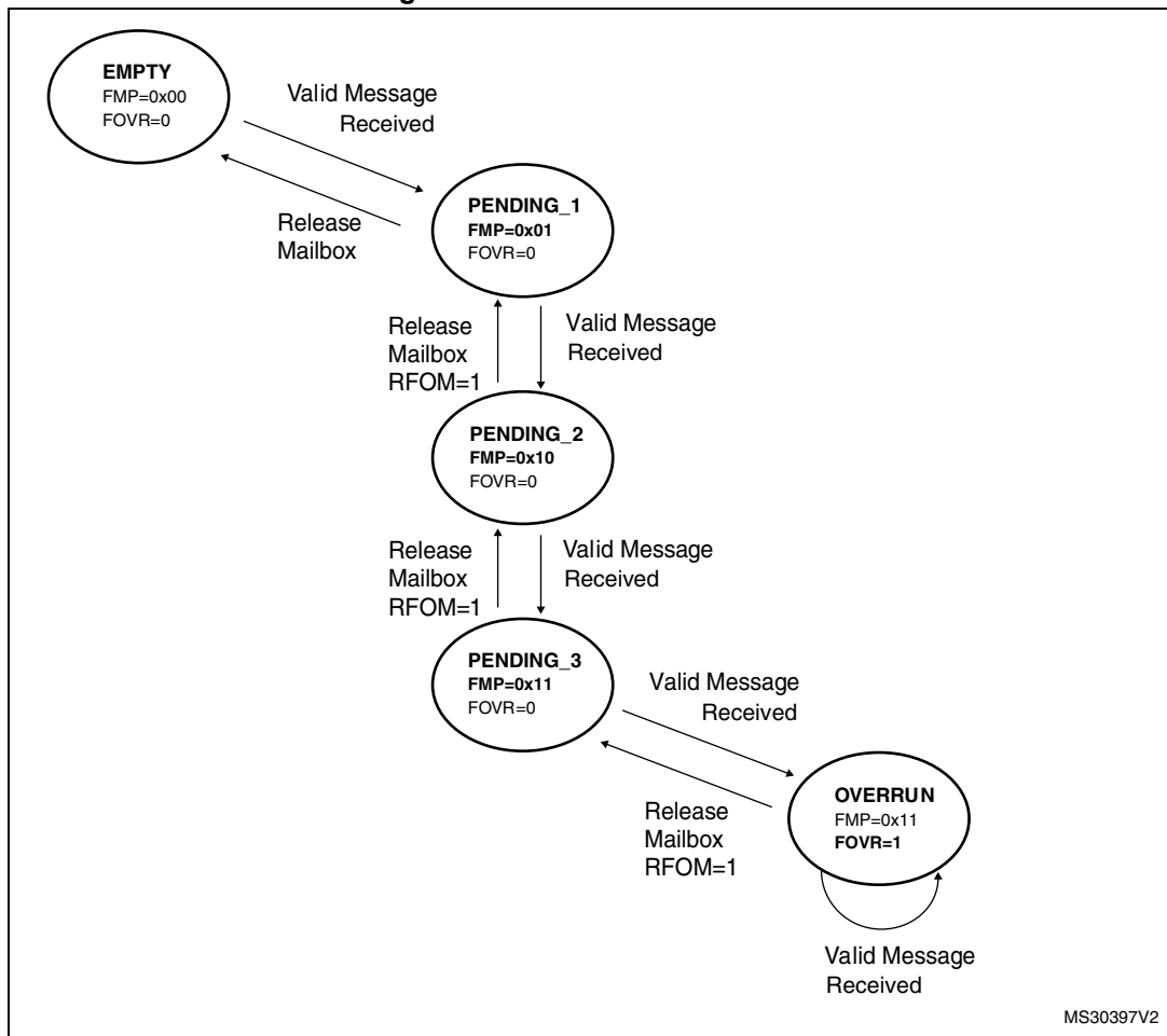
Figure 391. Receive FIFO states
