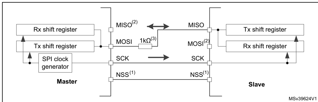
Figure 306. Half-duplex single master/ single slave application
