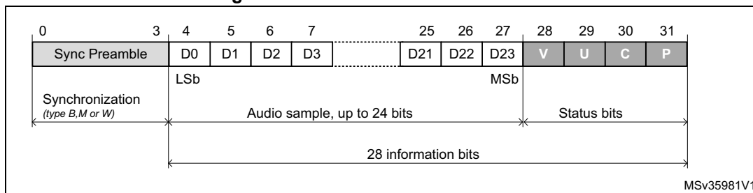
Figure 339. S/PDIF Sub-Frame Format
