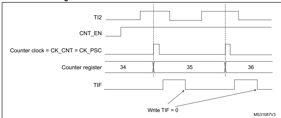
Figure 216. Control circuit in external clock mode 1
