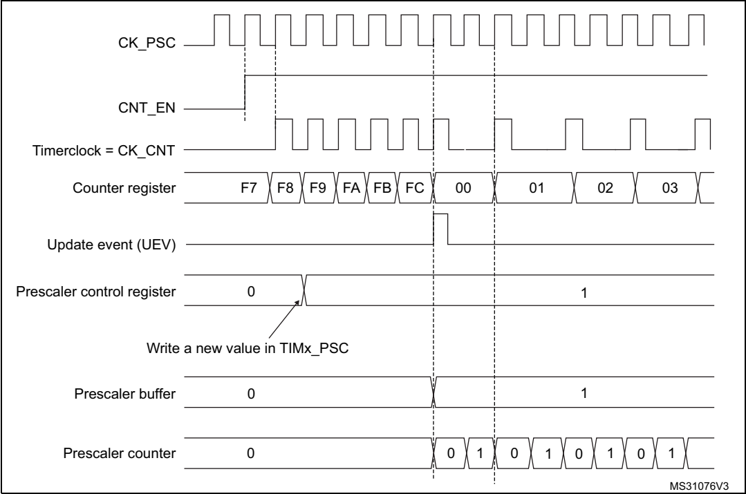
Figure 228. Counter timing diagram with prescaler division change from 1 to 2
