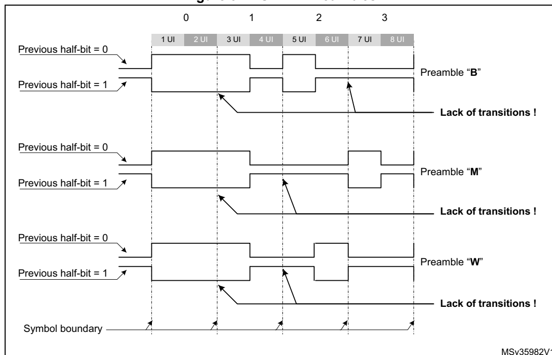
Figure 341. S/PDIF Preambles
