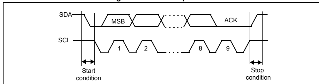
Figure 272. I 2 C bus protocol
