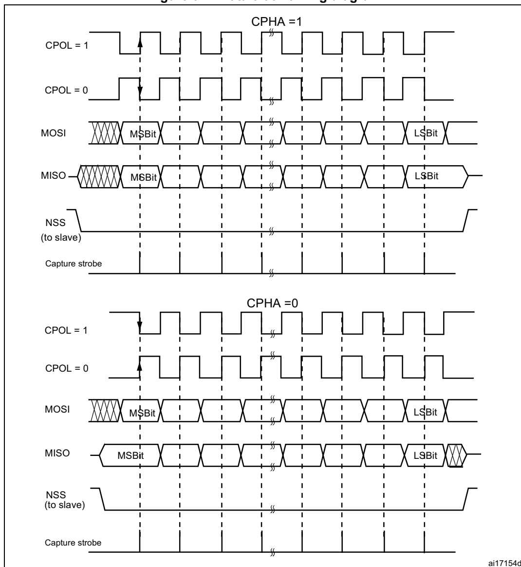
Figure 311. Data clock timing diagram
