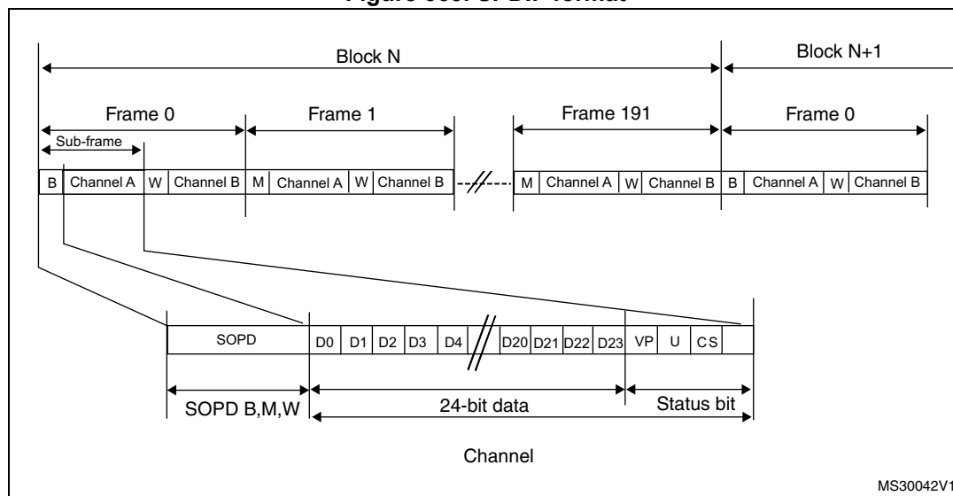
Figure 363. SPDIF format
