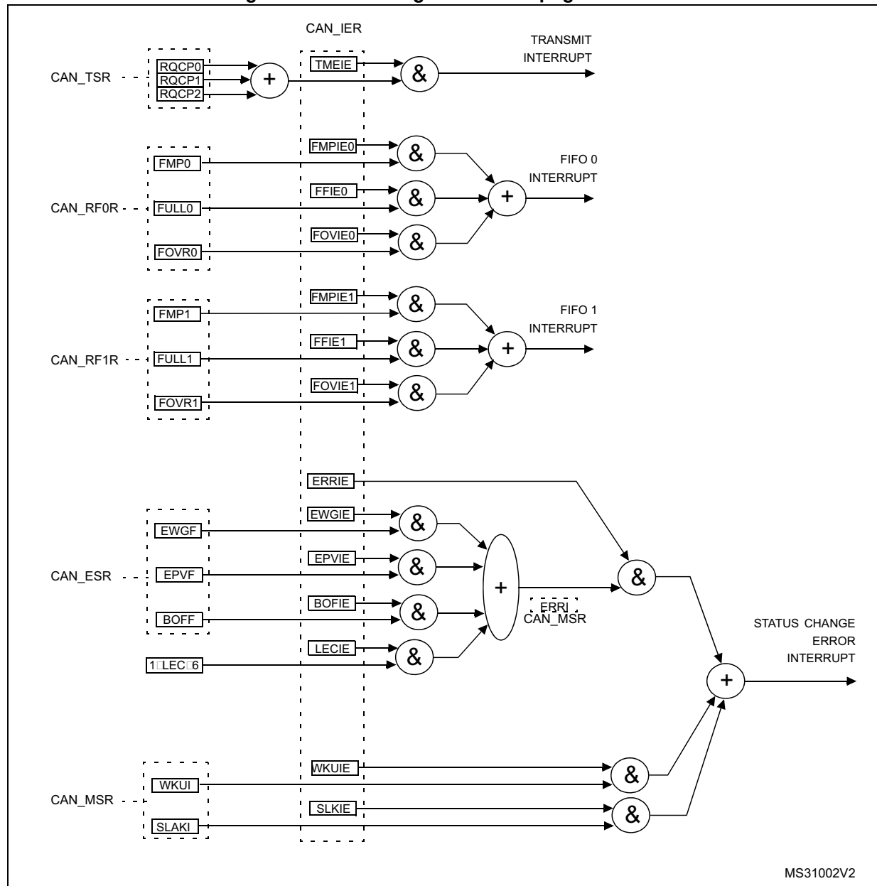
Figure 398. Event flags and interrupt generation
