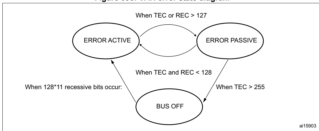
Figure 395. CAN error state diagram
