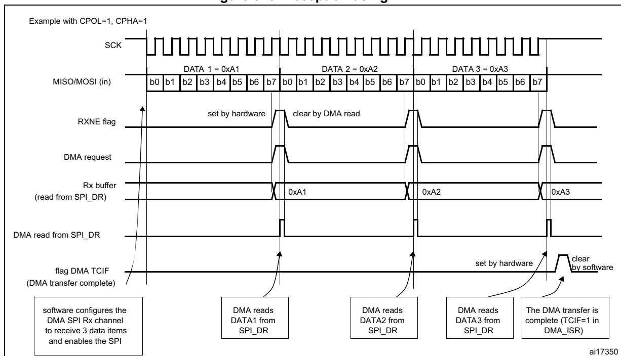
Figure 315. Reception using DMA
