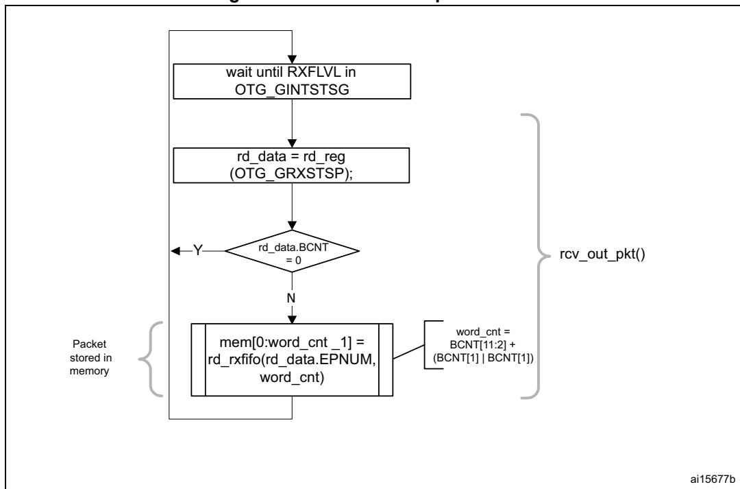
Figure 424. Receive FIFO packet read
