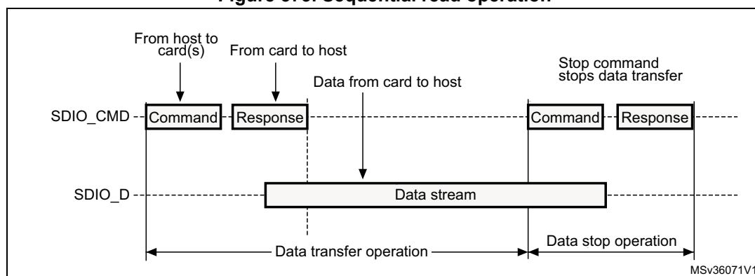
Figure 373. Sequential read operation
