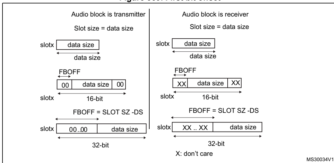
Figure 359. First bit offset
