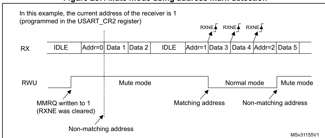
Figure 287. Mute mode using address mark detection
