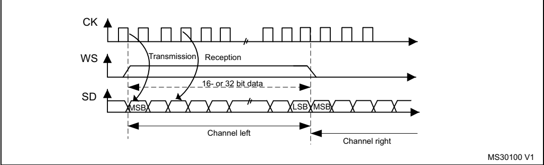
Figure 325. MSB Justified 16-bit or 32-bit full-accuracy length with CPOL = 0
