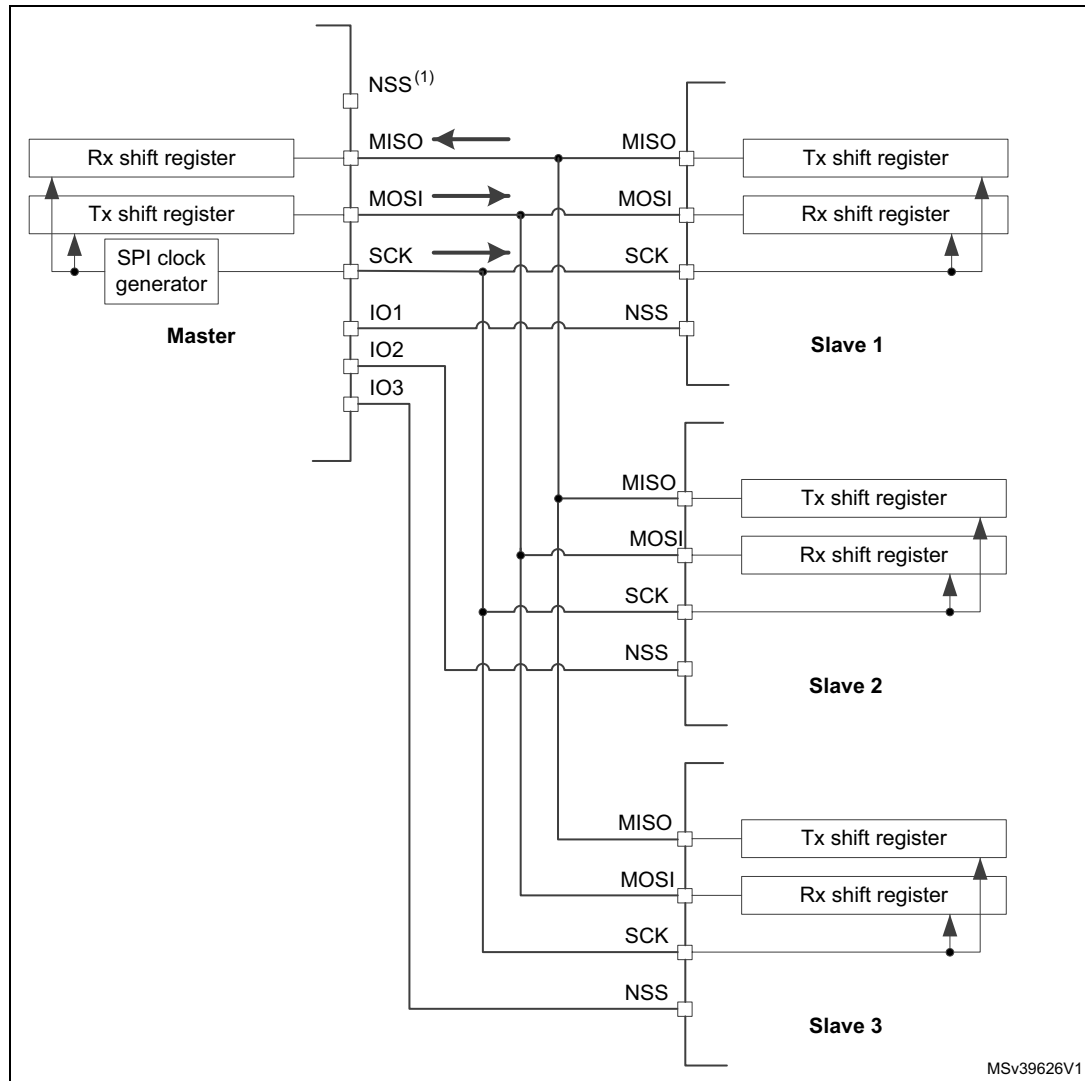
Figure 308. Master and three independent slaves
