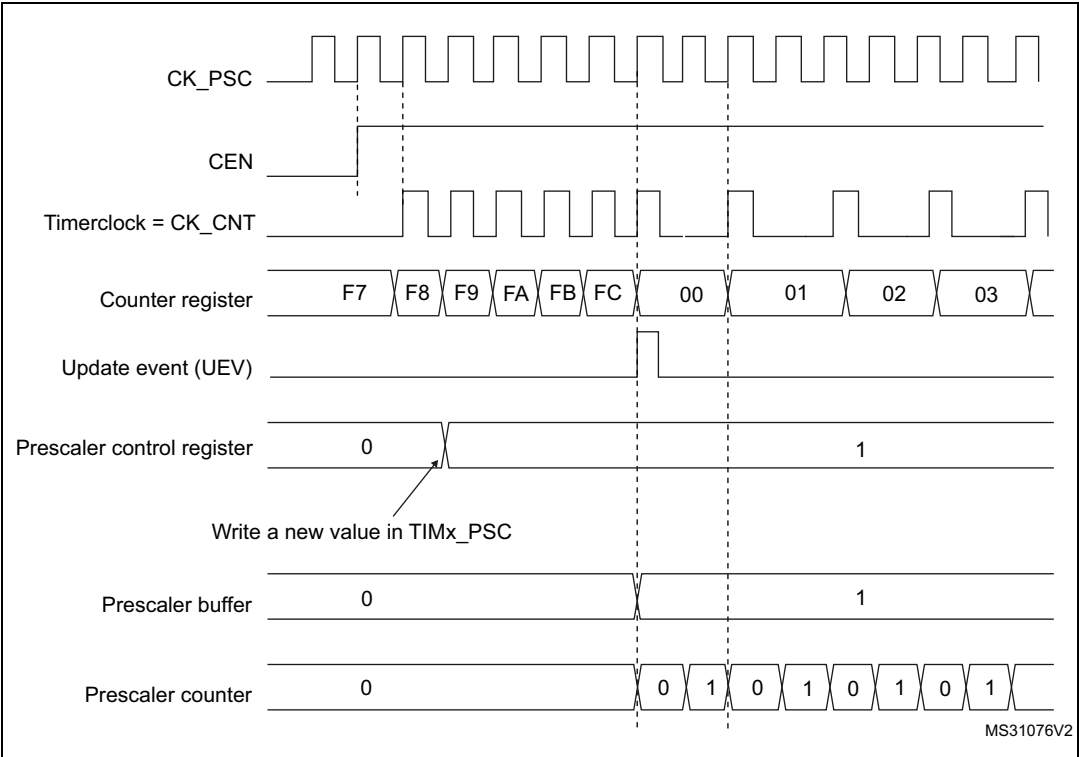
Figure 111. Counter timing diagram with prescaler division change from 1 to 2
