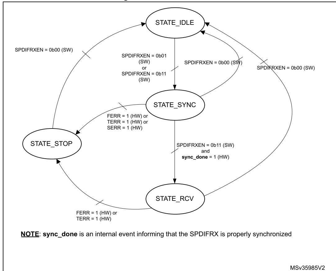
Figure 348. SPDIFRX States
