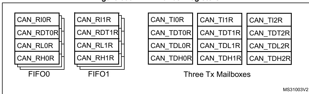
Figure 399. CAN mailbox registers
