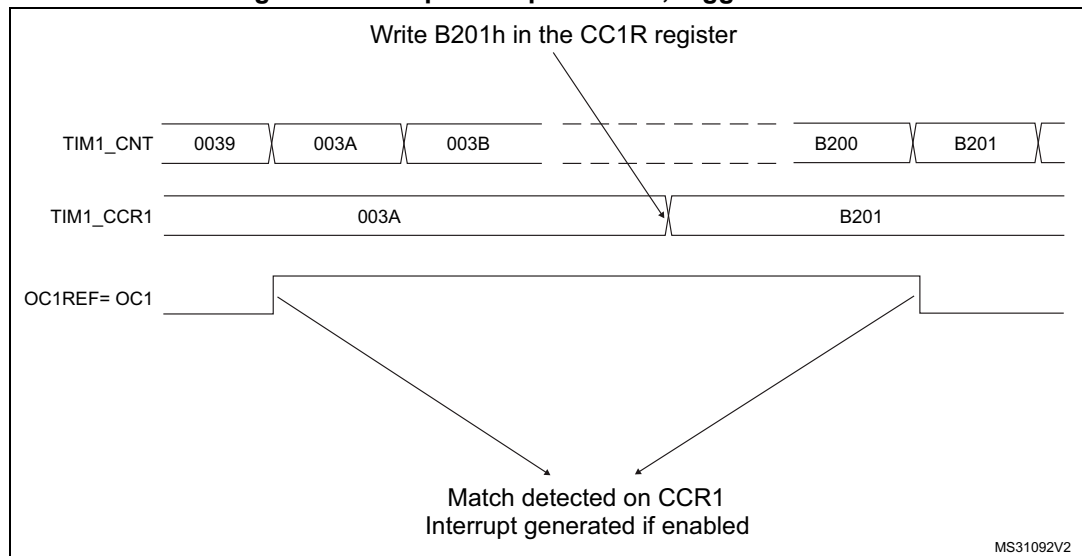
Figure 221. Output compare mode, toggle on OC1.
