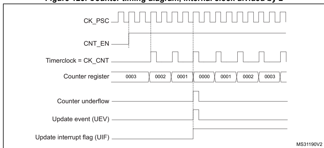
Figure 125. Counter timing diagram, internal clock divided by 2
