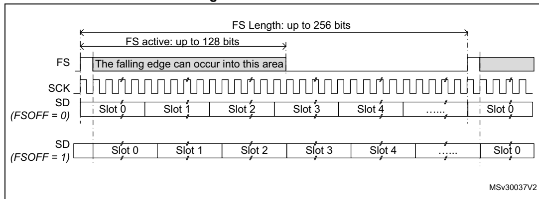
Figure 355. Audio frame
