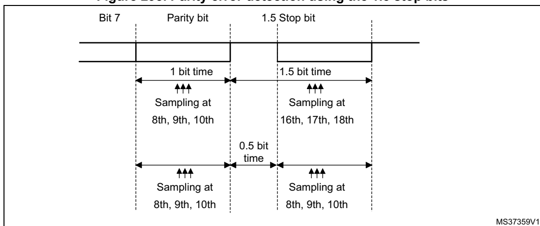
Figure 295. Parity error detection using the 1.5 stop bits
