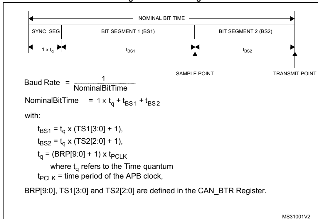
Figure 396. Bit timing
