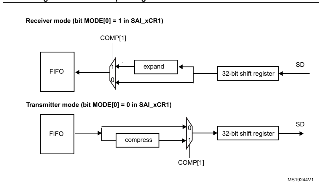
Figure 365. Data companding hardware in an audio block in the SAI
