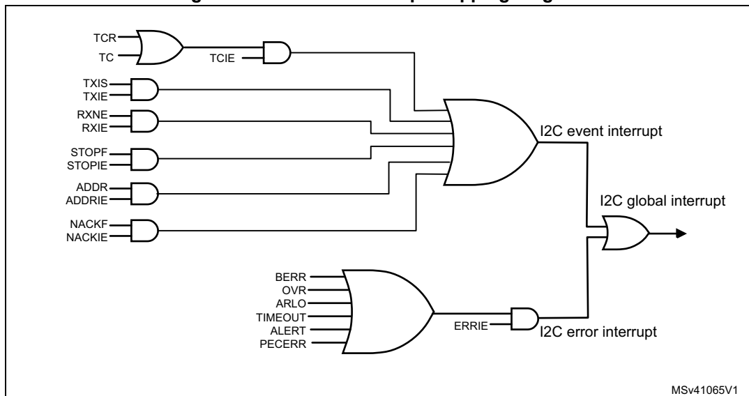
Figure 271. FMPI2C interrupt mapping diagram
