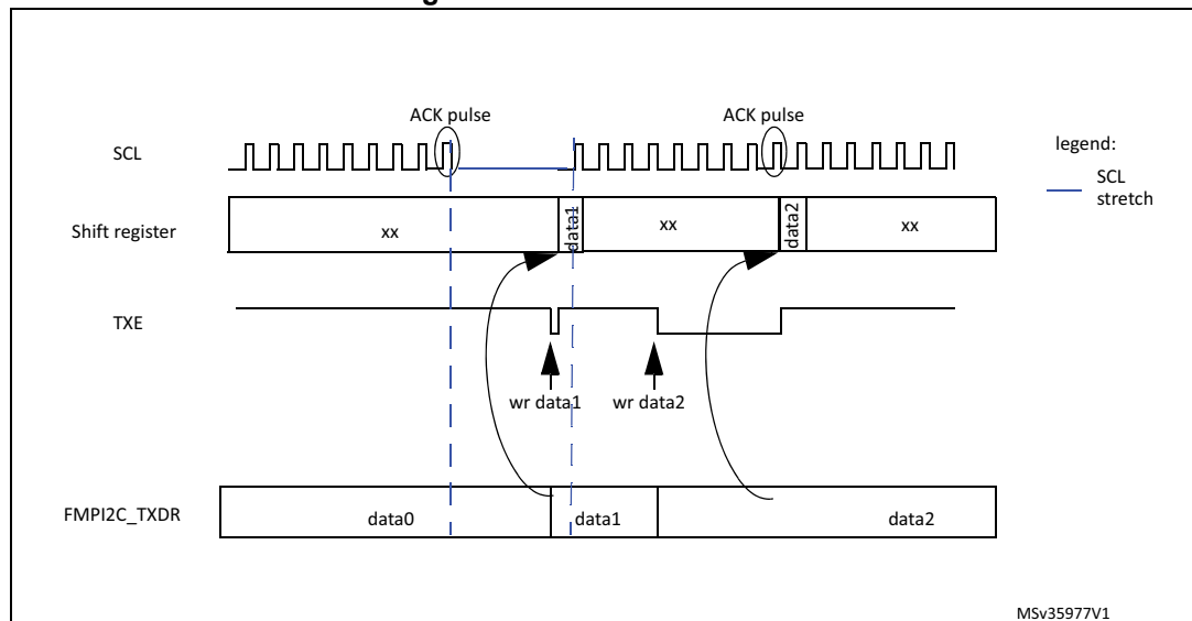
Figure 246. Data transmission
