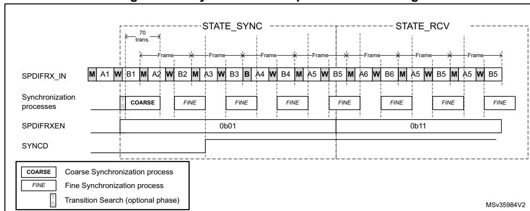
Figure 347. Synchronization process scheduling
