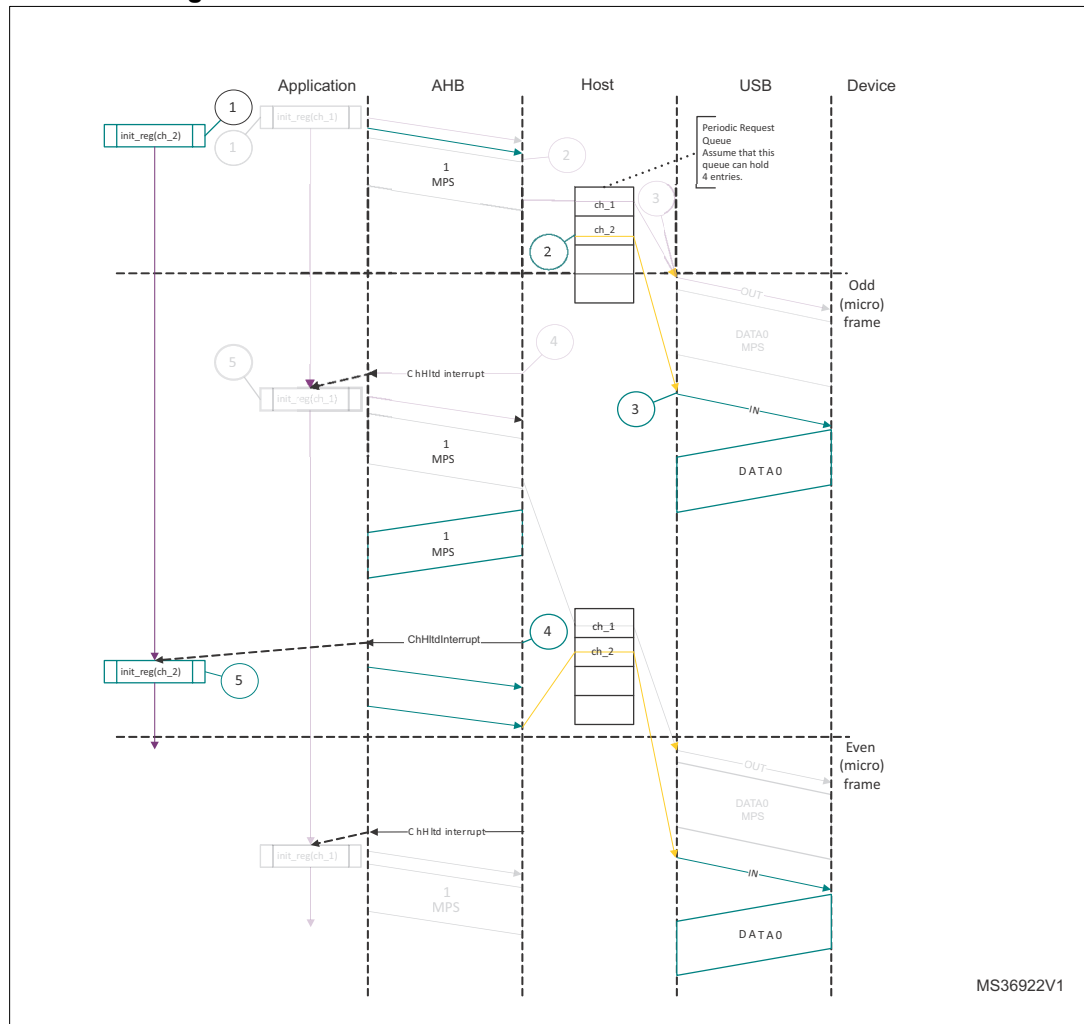
Figure 423. Normal isochronous IN transactions - DMA mode
