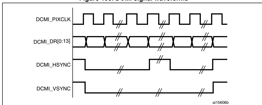
Figure 103. DCMI signal waveforms
