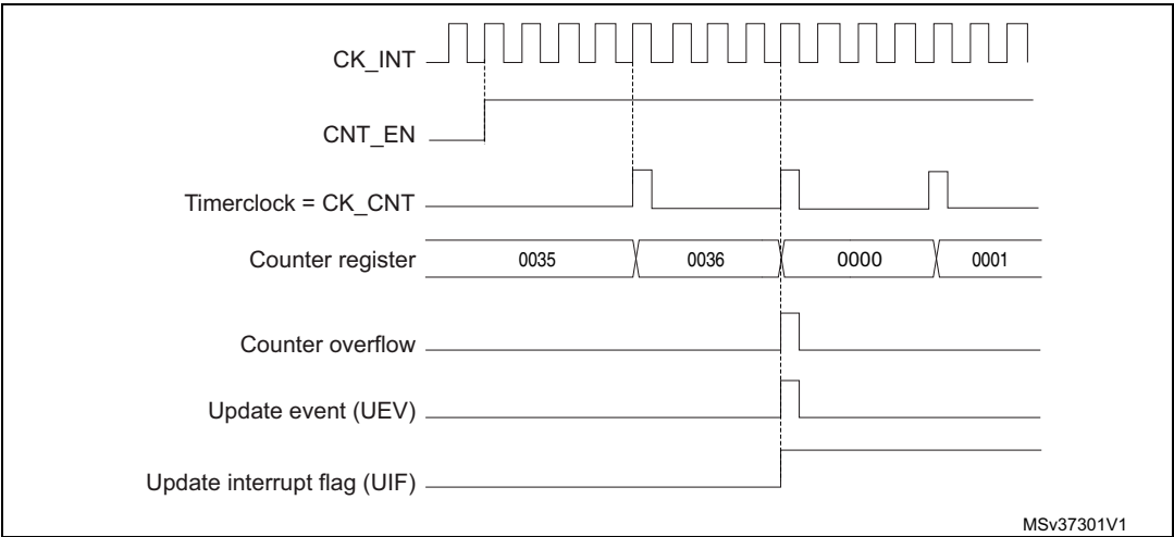
Figure 232. Counter timing diagram, internal clock divided by 4
