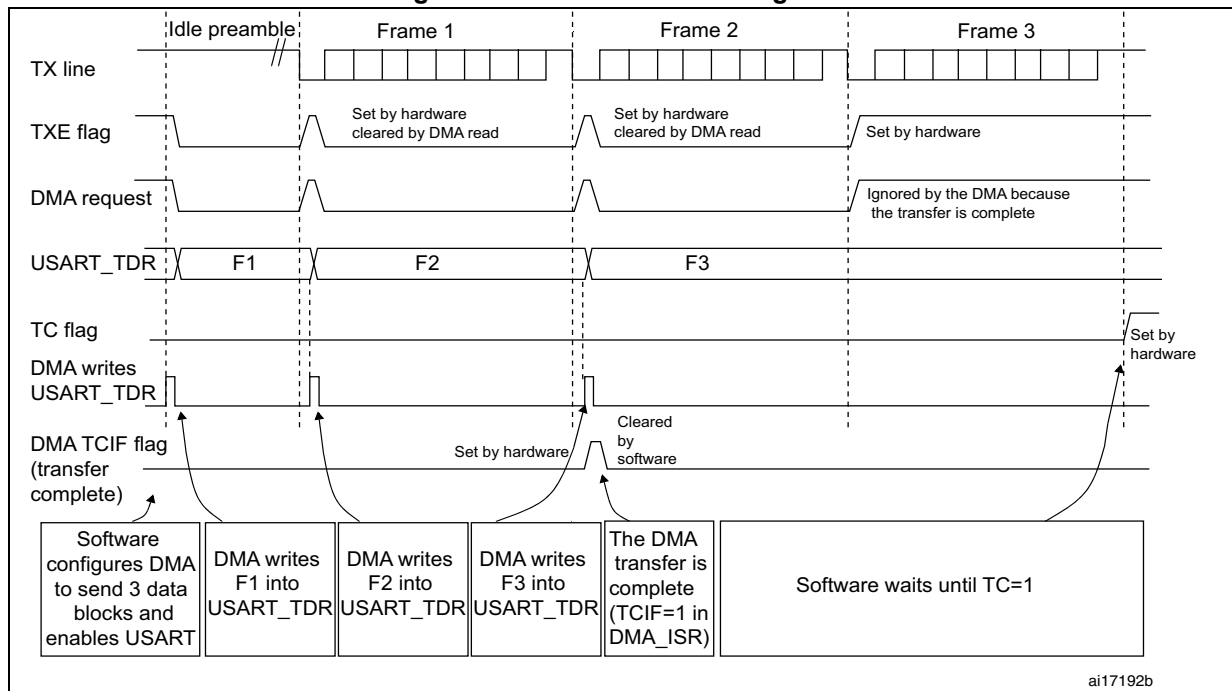
Figure 298. Transmission using DMA
