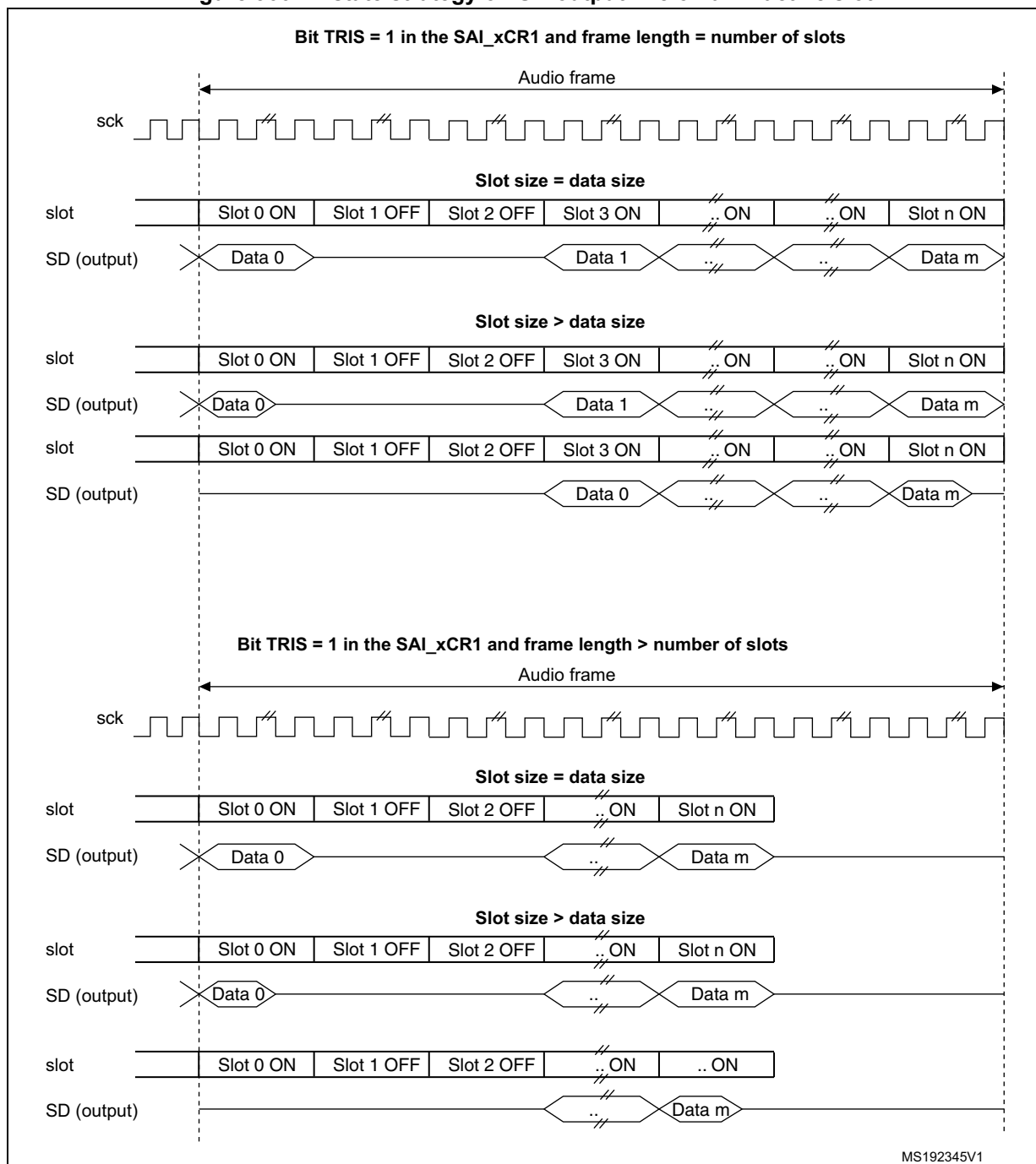
Figure 366. Tristate strategy on SD output line on an inactive slot
