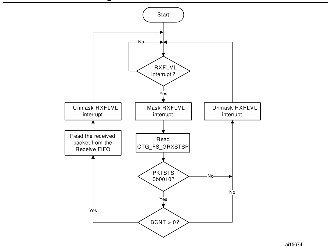
Figure 411. Receive FIFO read task
