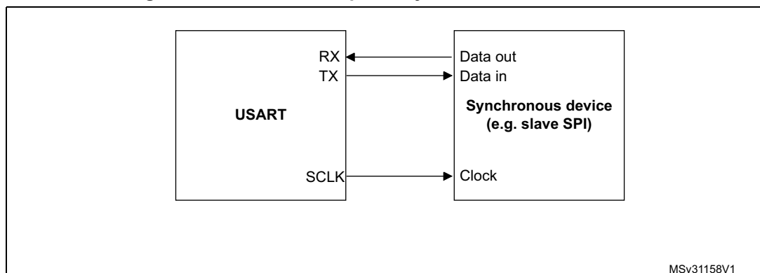
Figure 290. USART example of synchronous transmission
