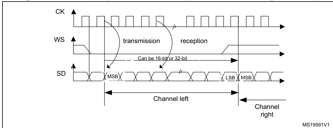
Figure 319. I 2 S Philips protocol waveforms (16/32-bit full accuracy, CPOL = 0)
