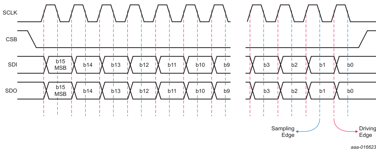
Fig 4. SPI timing protocol
