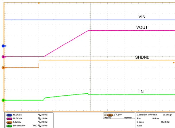
Figure 53. Hot Plug With VIN - No Load
