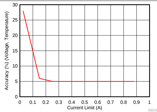
Figure 20. Current Limit Accuracy vs Current Limit, I_{OL}
