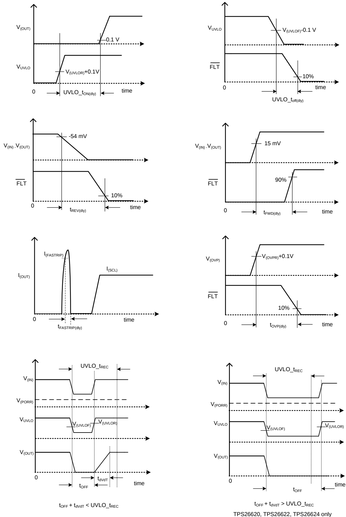
Figure 30. Timing Waveforms
