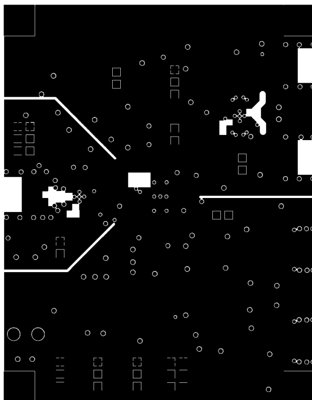
Figure 4. VCC Layer
