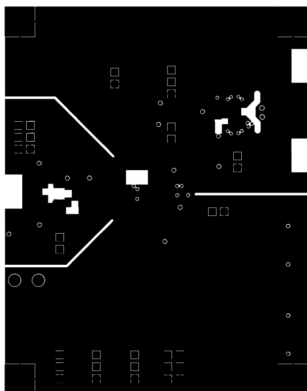
Figure 3. GND Layer
