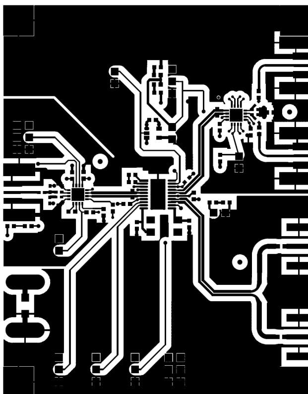
Figure 2. Top Layer
