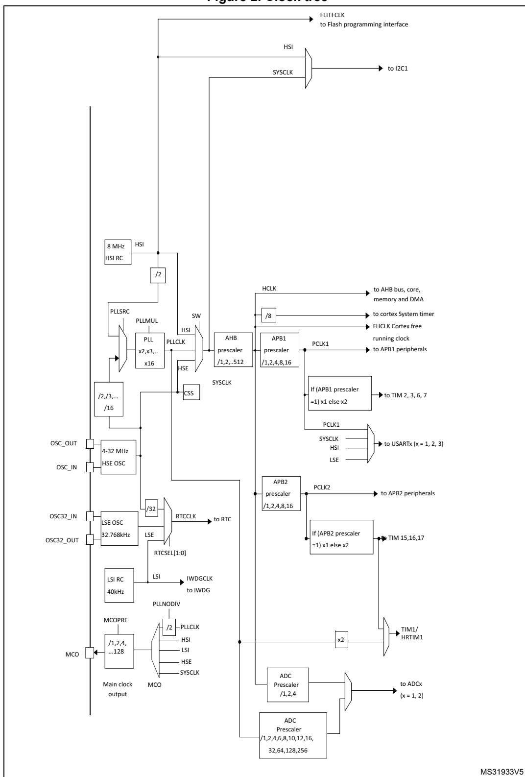
Figure 2. Clock tree
