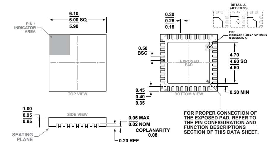
Figure 59. 40-Lead Lead Frame Chip Scale Package [LFCSP] 6 mm × 6 mm Body and 0.95 mm Package Height (CP-40-15)
