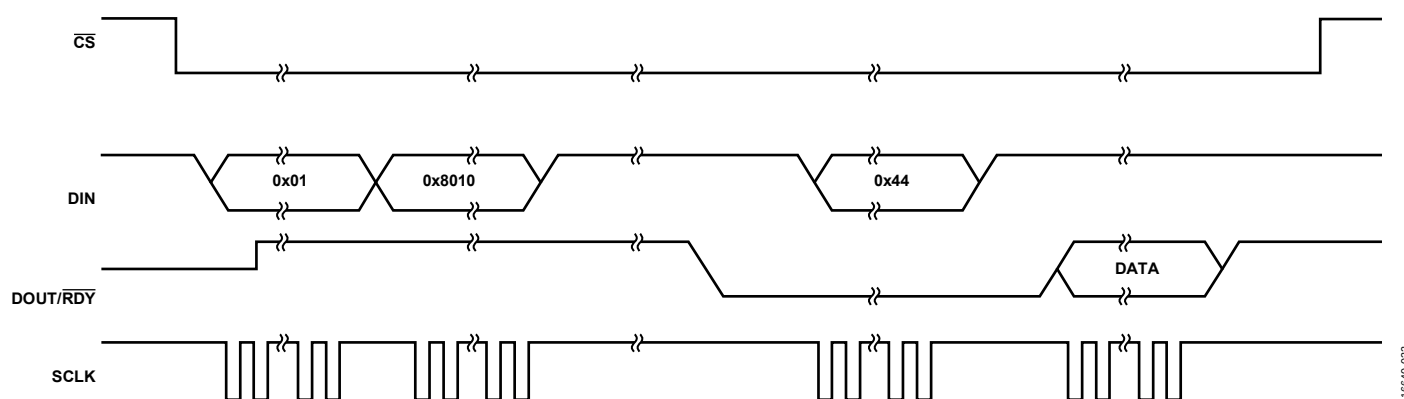
Figure 56. Single Conversion Mode
