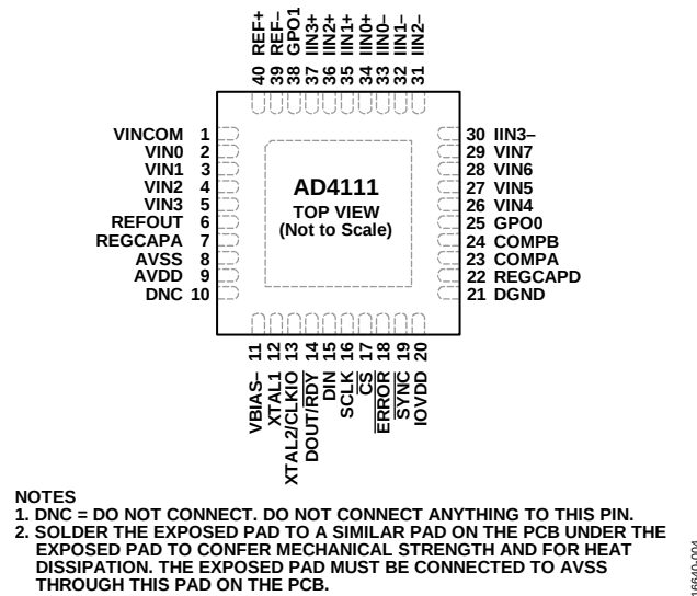
Figure 4. Pin Configuration
