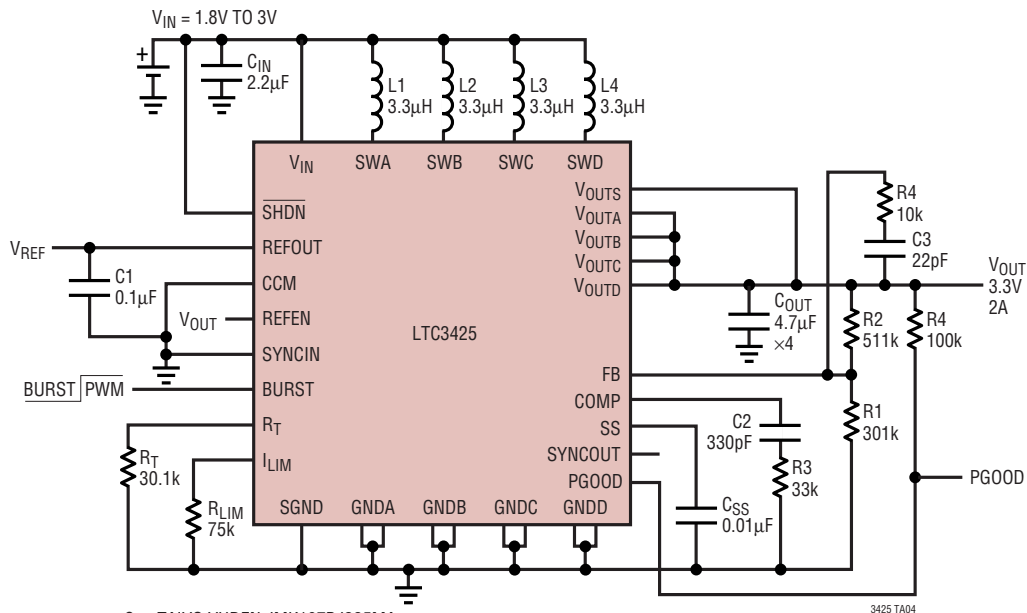
C IN : TAIYO YUDEN JMK107BJ225MA C OUT : TAIYO YUDEN JMK212BJ475MG (×4) L1 TO L4: SUMIDA CDRH4D28
