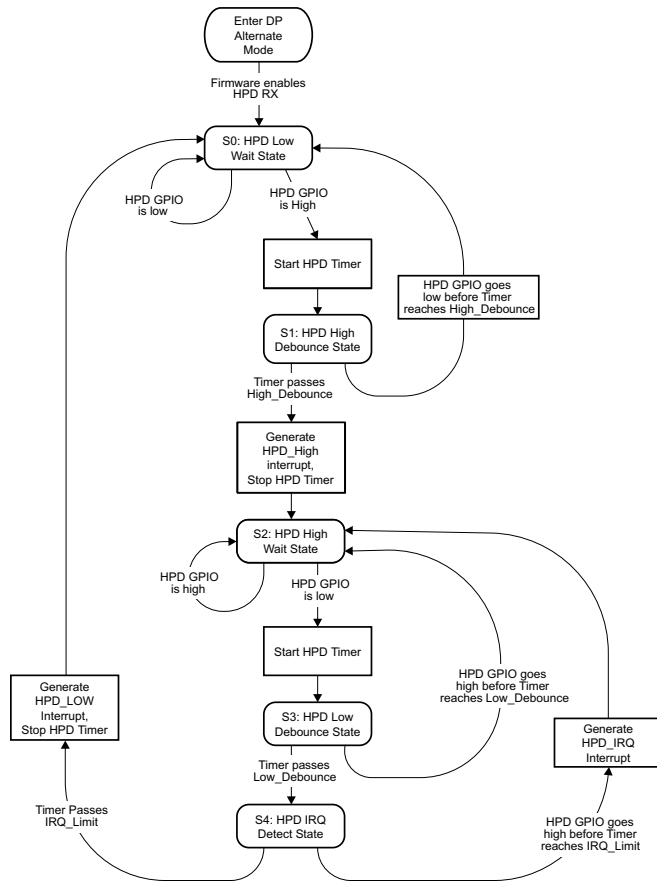
Figure 10-1. DisplayPort Sink-Side Hardware Flow (HPD RX)
