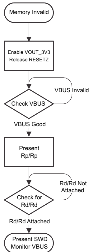
Figure 3-6. Memory Invalid Flow
