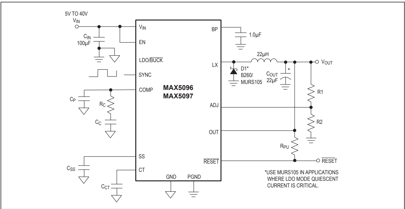
Figure 4. Adjustable Output Voltage Configuration
