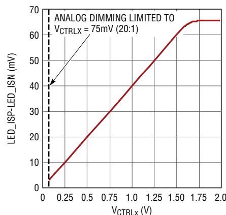
Figure 3. Sense Voltage vs CTRL Voltage
