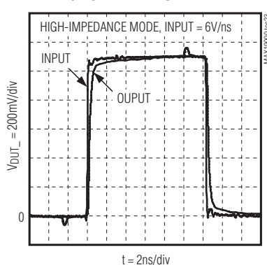
COMPARATOR RESPONSE TO HIGH SLEW-RATE OVERDRIVE
