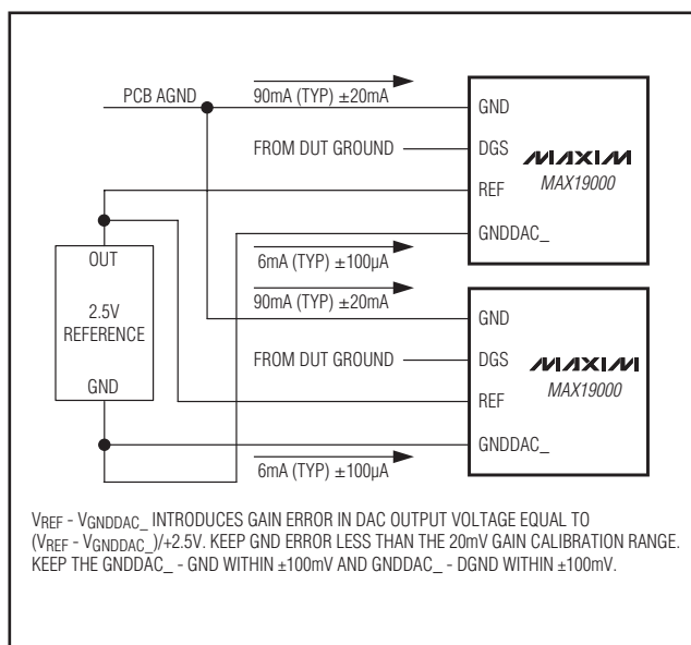
Figure 10. Sample Connection Diagram for Two Parts per Board
