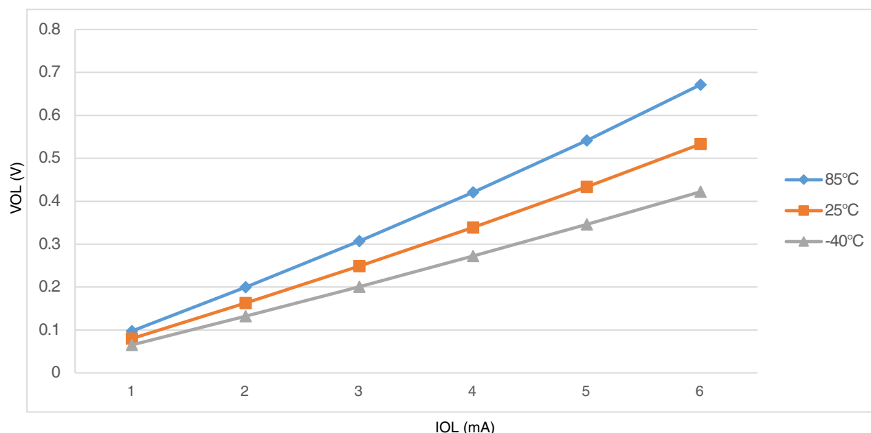
Figure 5. Typical I_{OL} Vs. V_{OL} (standard drive strength) ( V_{DD} = 3\text{ V} )
