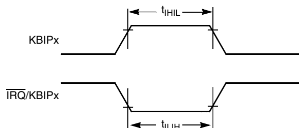
Figure 7. IRQ/KBIPx timing
