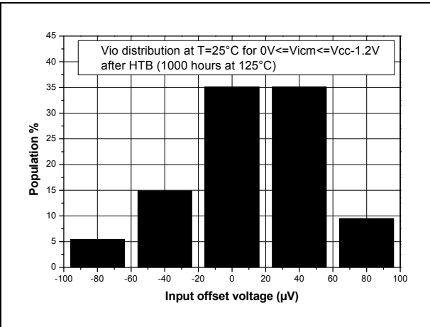
Figure 4. Input offset voltage distribution for V_{icm} \leq V_{CC}-1.2\text{ V} at T=25^\circ\text{C} after HTB
