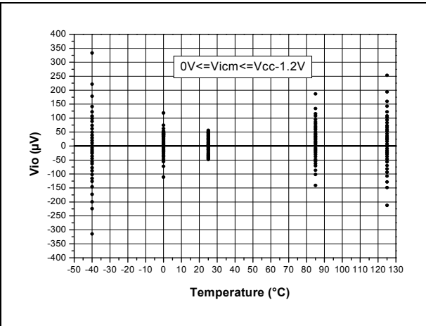
Figure 2. Input offset voltage distribution vs. temperature for V_{icm} \leq V_{CC}-1.2\text{ V}
