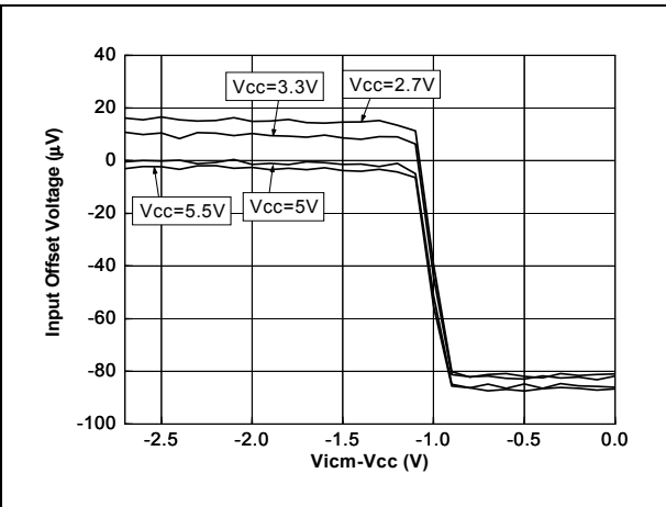
Figure 6. Input offset voltage vs. input common mode voltage at T=25^\circ\text{C}
