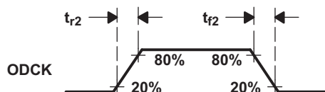
Figure 3. Rise and Fall Times of ODCCK
