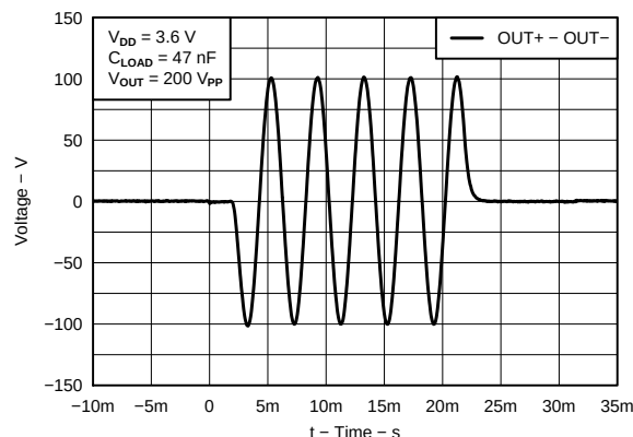
Figure 16. Typical Waveform - Differential
