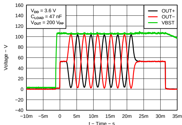
Figure 15. Typical Waveform
