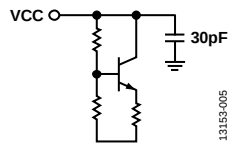
Figure 5. VCC Interface
