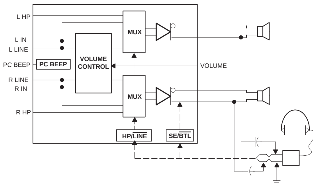
Figure 3–4. TPA0242 Amplifier IC
