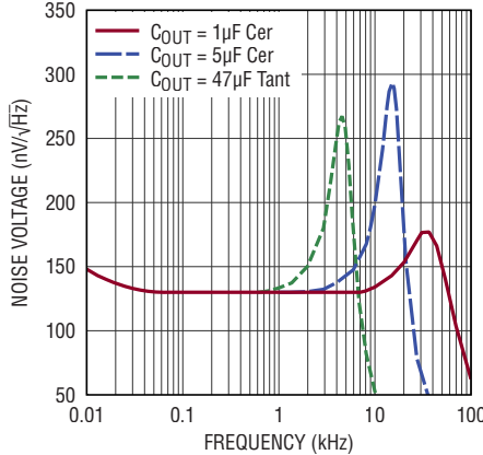
5V Output Voltage Noise Spectrum
