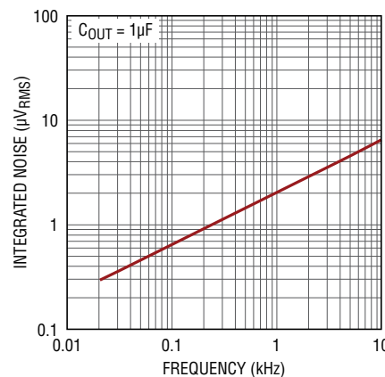
2.5V Integrated Noise 10Hz to 10kHz
