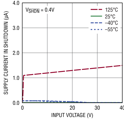
2.5V Supply Current in Shutdown vs Input Voltage
