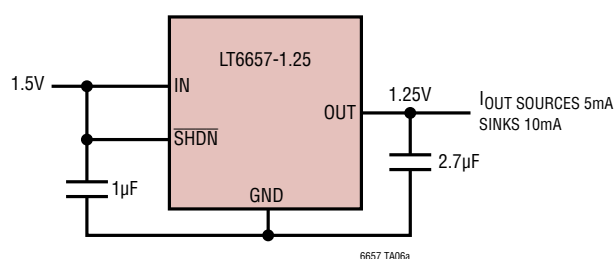
1.5V Minimum Supply Voltage
