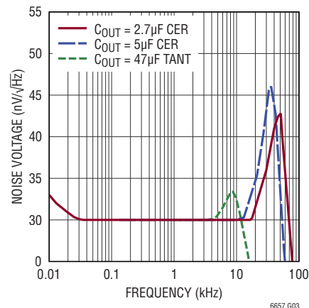
1.25V Output Voltage Noise Spectrum
