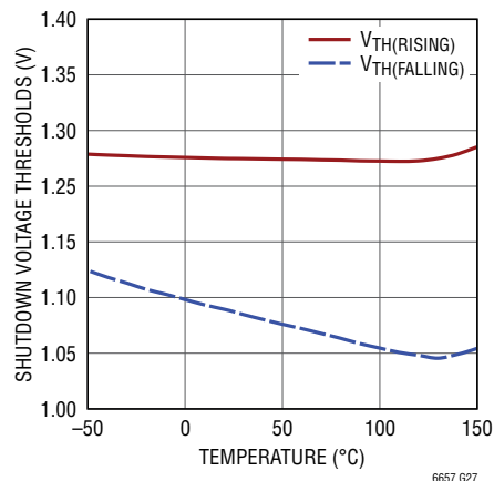
Shutdown Voltage Thresholds vs Temperature
