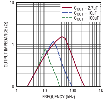
1.25V Output Impedance vs Frequency
