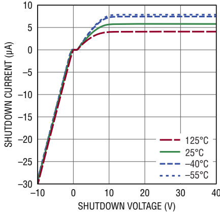
Shutdown Pin Current vs Shutdown Voltage
