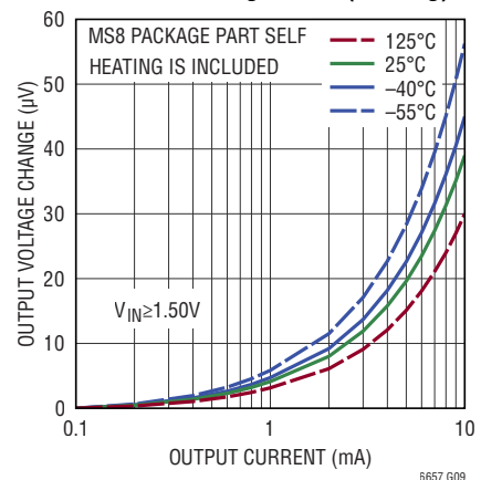
1.25V Load Regulation (Sinking)
