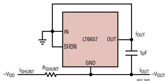
Negative Shunt Mode Reference
