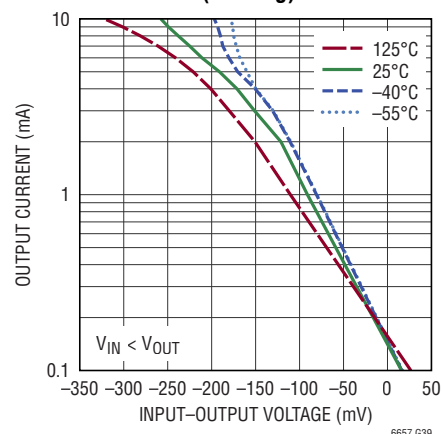
5V Minimum V_{IN} to V_{OUT} Differential (Sinking)
