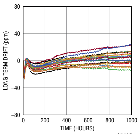
Figure 18a. Long-Term Drift
