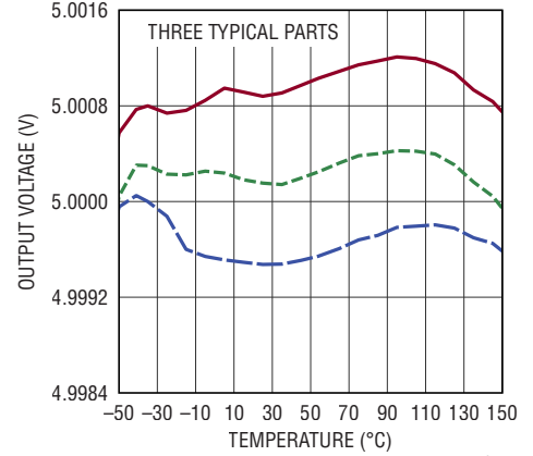
5V Output Voltage Temperature Drift
