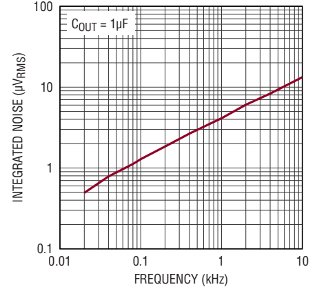
5V Integrated Noise 10Hz to 10kHz
