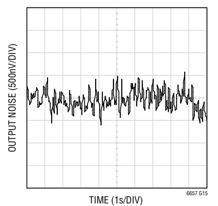
2.5V Low Frequency 0.1Hz to 10Hz Noise
