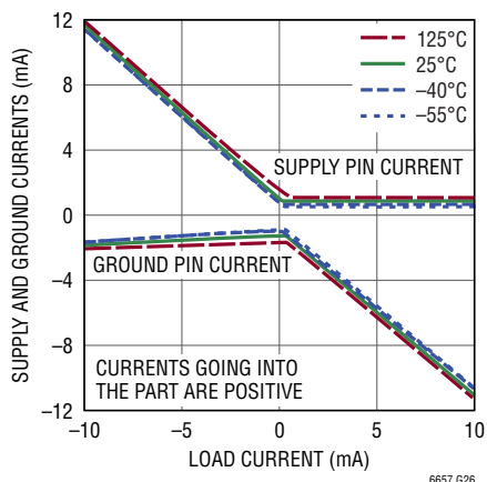
Supply and Ground Currents vs Load Current
