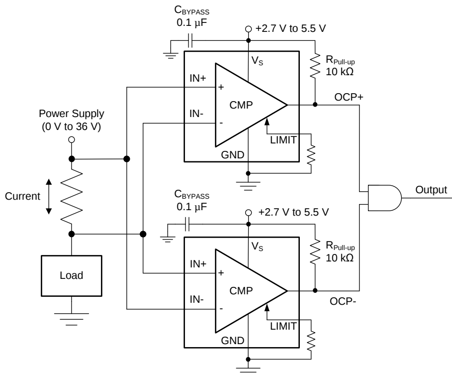
Figure 35. Bidirectional Application
