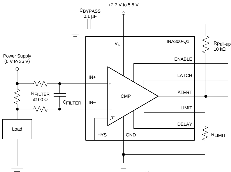
Figure 30. Input Filter
