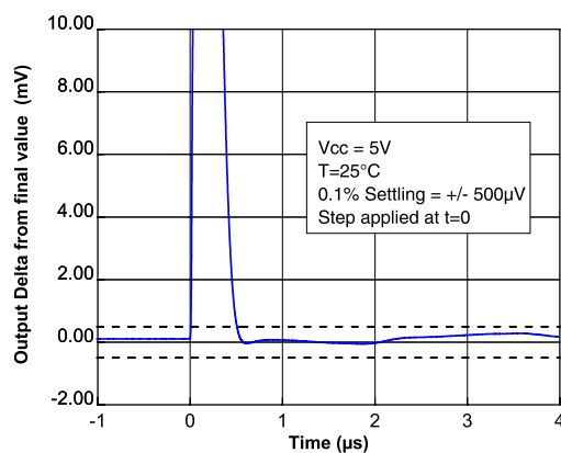
Figure 39. Settling time positive step (-2 V to 0 V)
