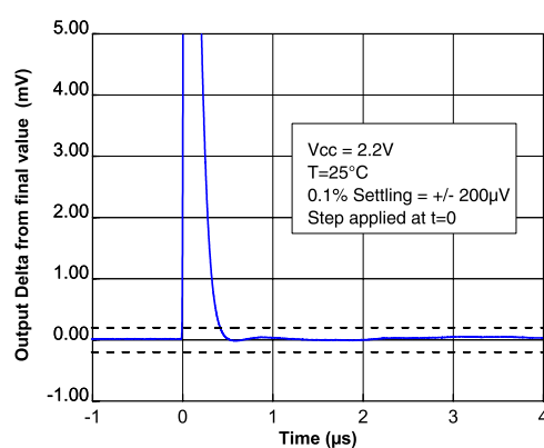
Figure 41. Settling time positive step (-0.8 V to 0 V)
