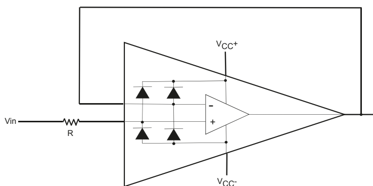
Figure 50. Input current limitation
