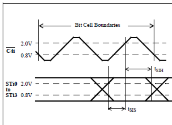
Figure 16 - Serial Inputs
