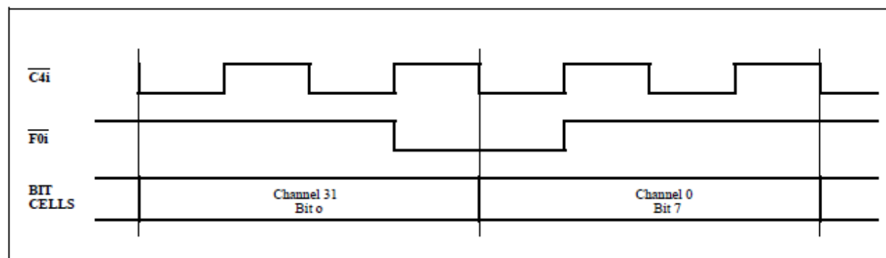
Figure 12 - Frame Alignment
