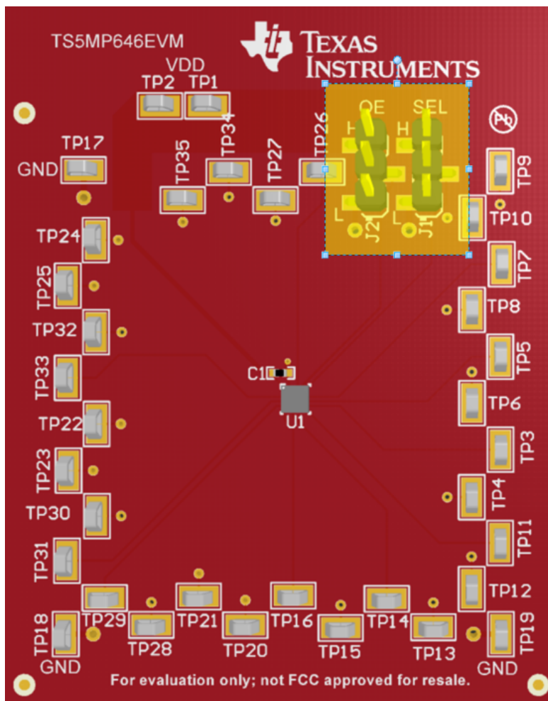
Figure 3. SEL0, SEL1, \overline{EN} Jumpers
