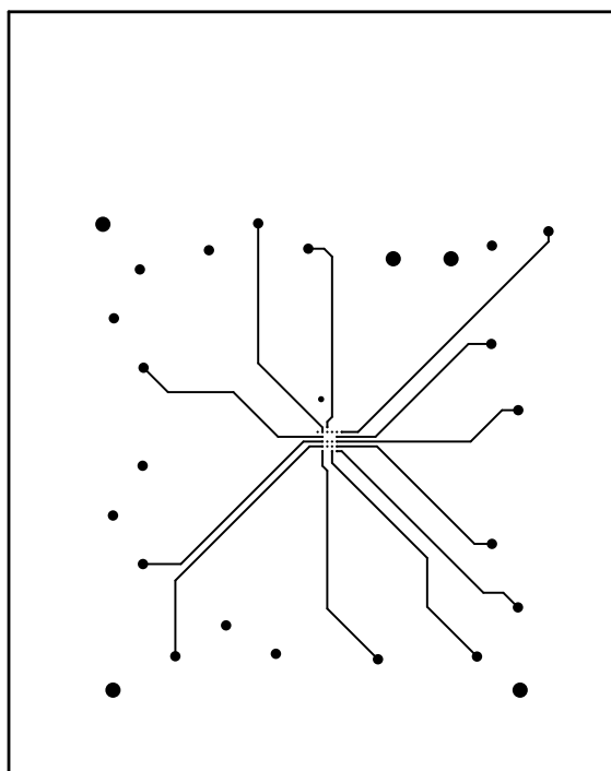
Figure 7. Layer 2
