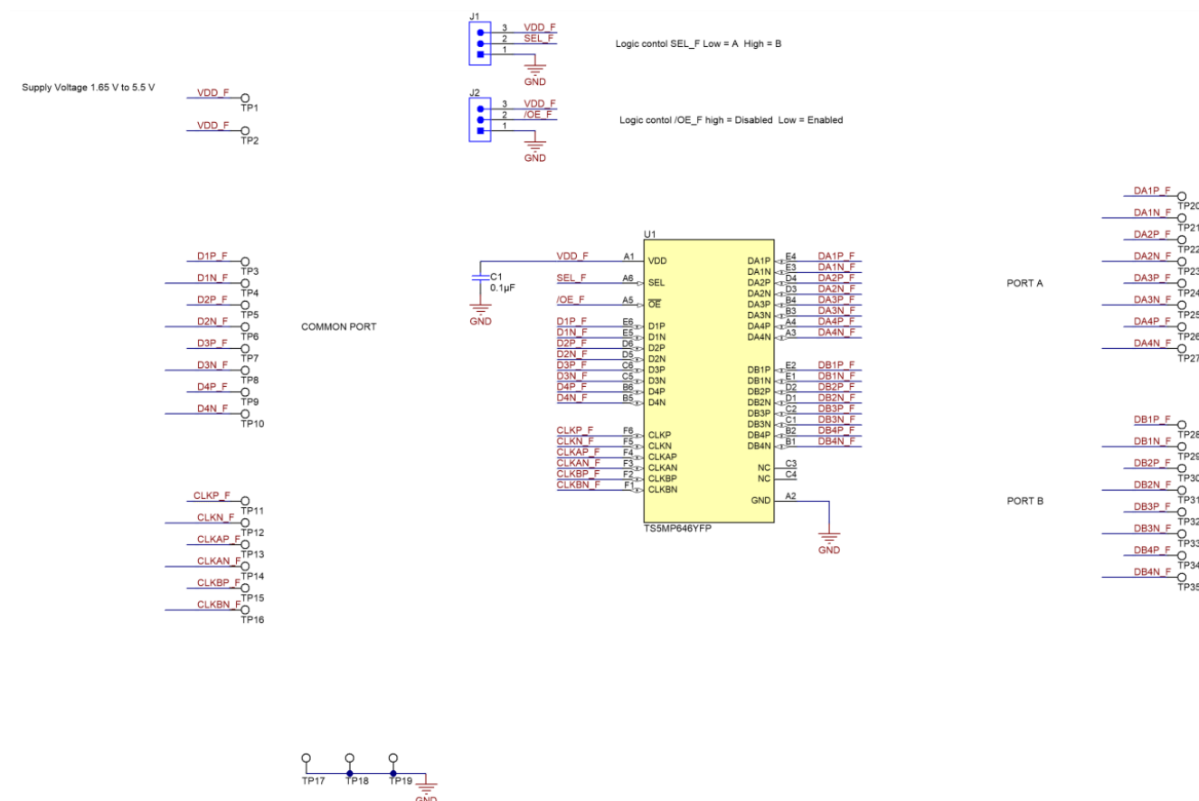
Figure 4. TS5MP646EVM Schematic
