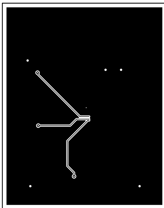
Figure 9. Bottom Copper
