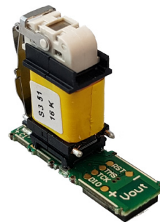
Figure 8. Switch Reference Design without the Wings
