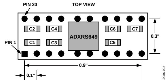
Figure 2. EVAL-ADXRS649Z Layout
