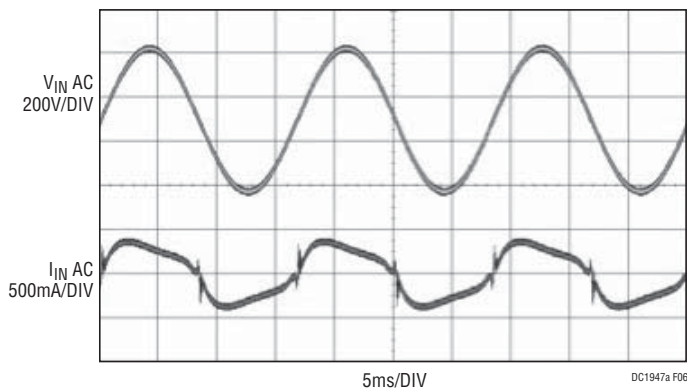
Figure 6. V_{IN} = 230VAC
