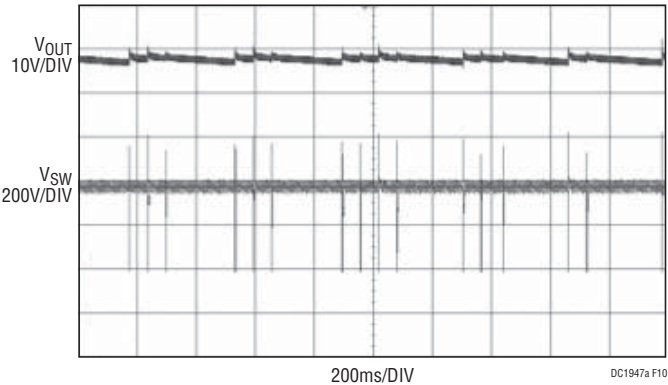
Figure 10. V_{IN} = 230VAC
