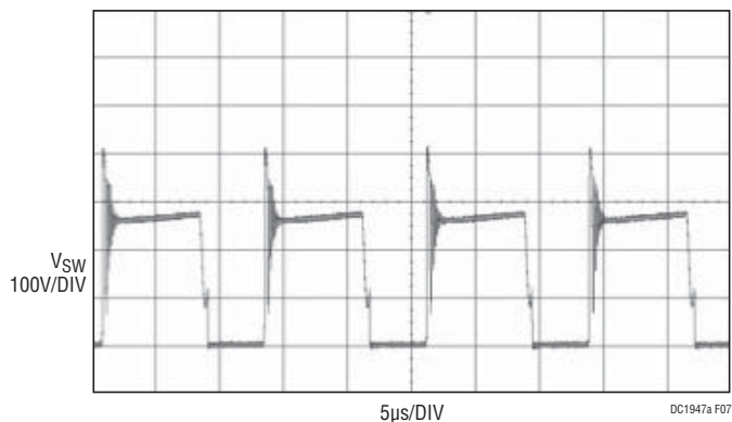
Figure 7. V_{IN} = 120VAC
