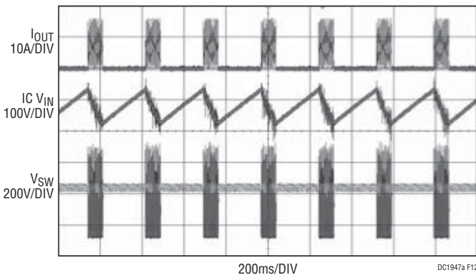
Figure 12. V_{IN} = 230VAC
