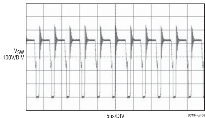
Figure 8. V_{IN} = 230VAC
