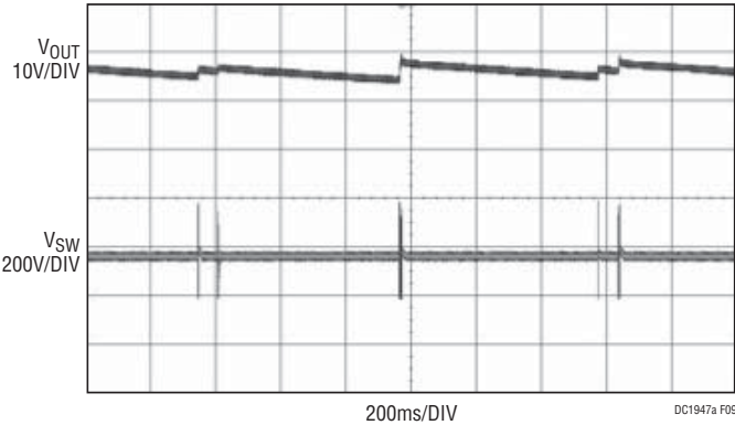
Figure 9. V_{IN} = 120VAC
