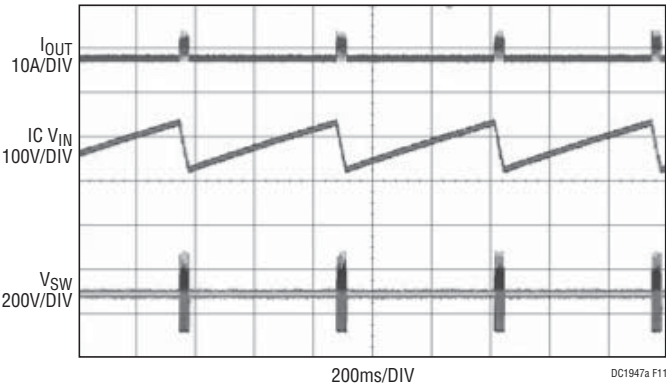
Figure 11. V_{IN} = 120VAC
