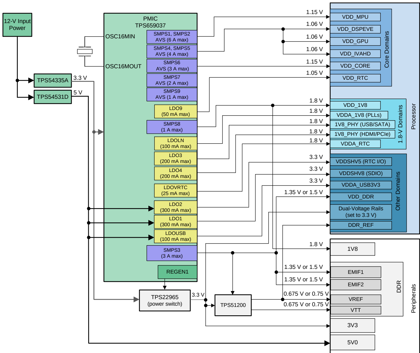
Figure 1. Processor Connection With TPS659037ZWSR
