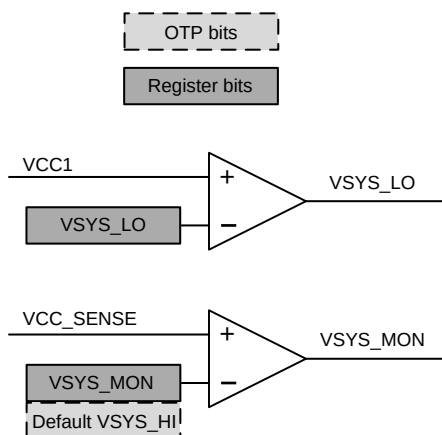
Figure 5. PMIC Comparators
