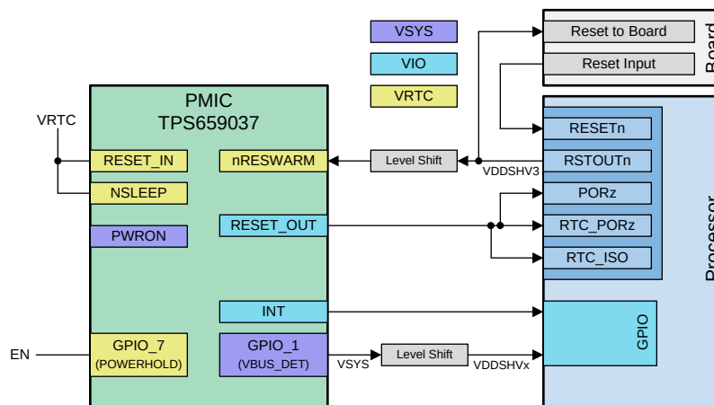
Figure 3. Reset Connections With POWERHOLD Configuration
