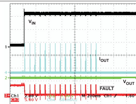
Figure 17. OVP Response for Input Step
