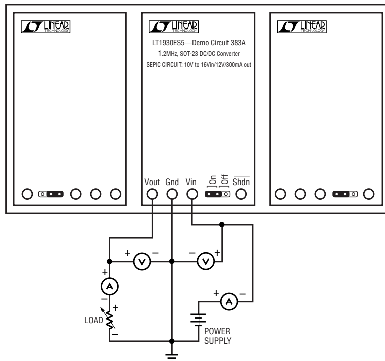
Figure 2. Proper Measurement Equipment Setup for SEPIC Circuit
