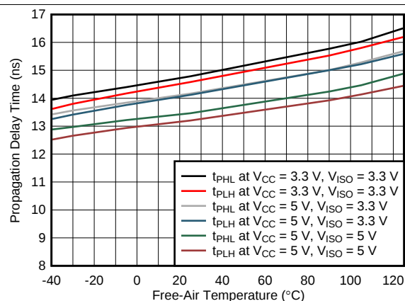
Figure 22. Propagation Delay Time vs Free-Air Temperature
