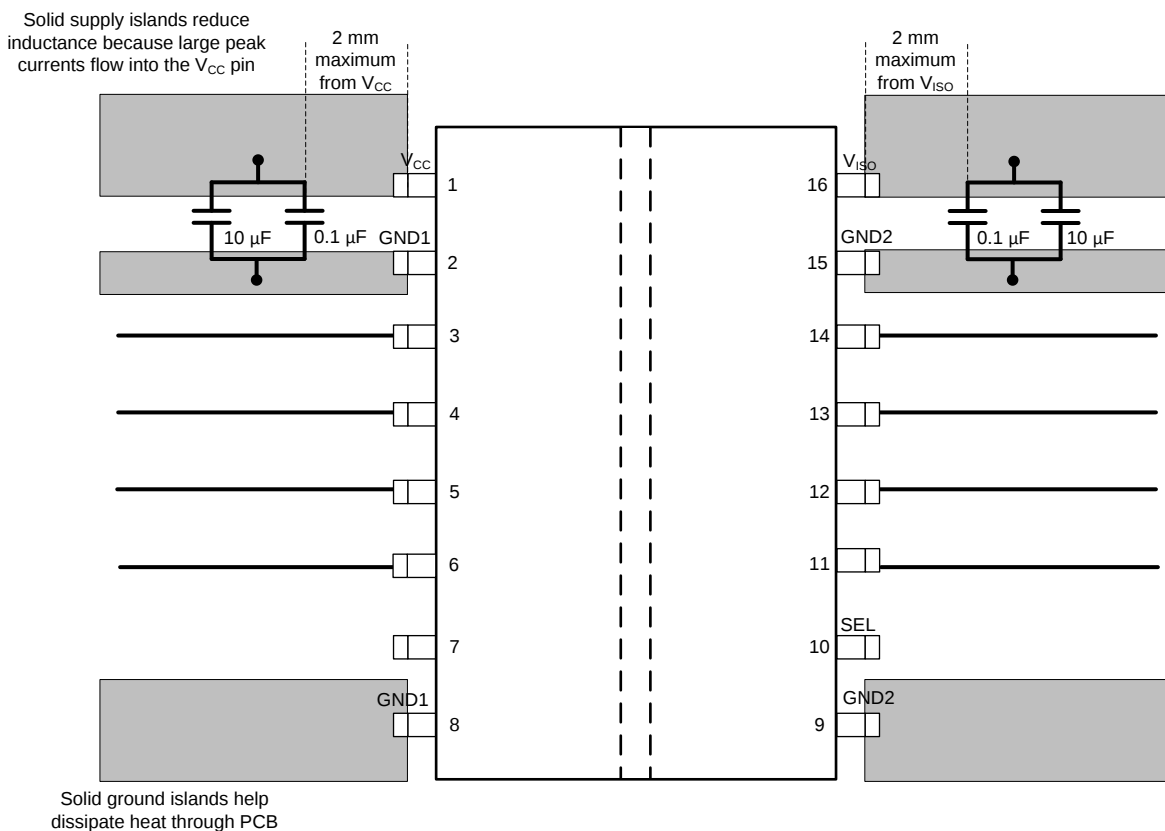
Figure 43. Layout Example
