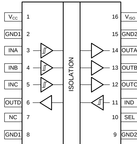
ISOW7841 DWE Package 16-Pin SOIC-WB Top View
