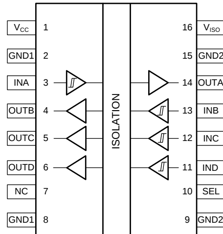
ISOW7843 DWE Package 16-Pin SOIC-WB Top View
