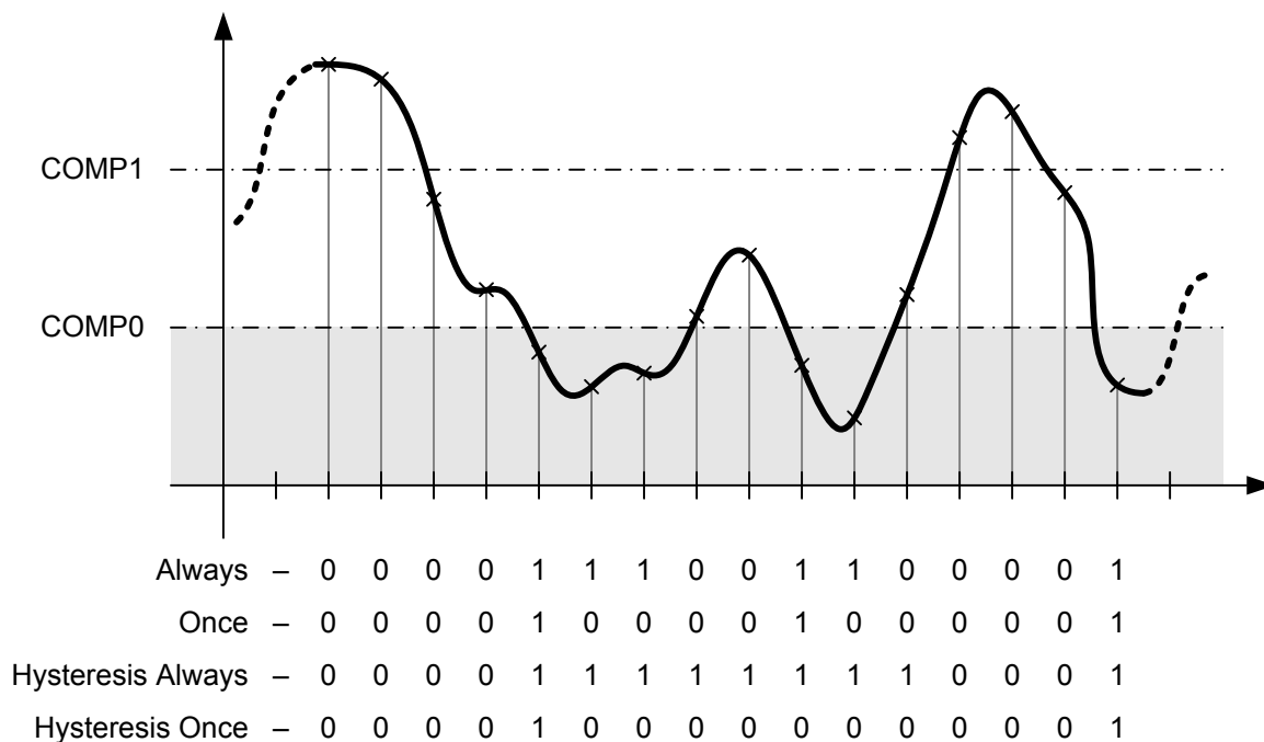
Figure 18-12. Low-Band Operation (CIC=0x0 and/or CTC=0x0)
