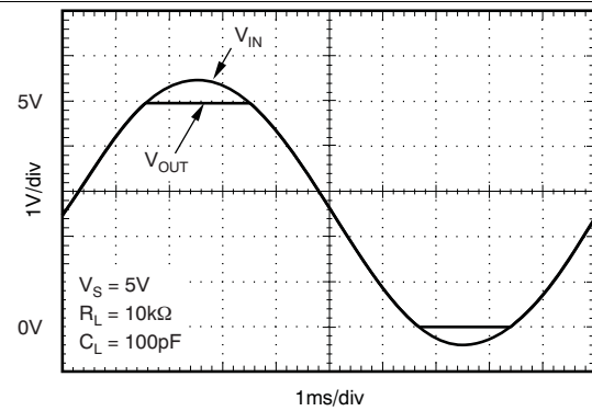
Figure 52. Output Overdrive Performance
