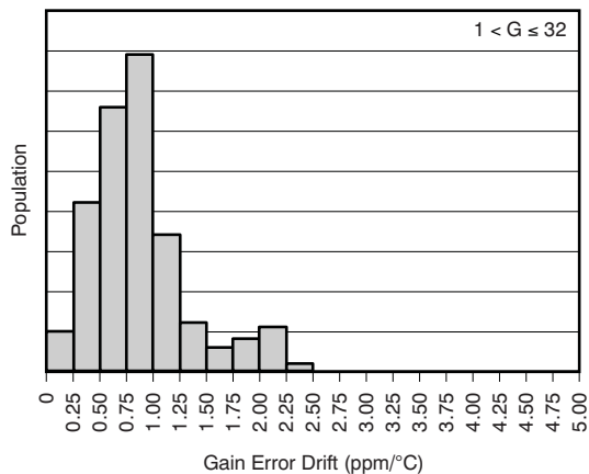
Figure 15. Gain Error Drift ( -40^\circ\text{C} to 125^\circ\text{C} )
