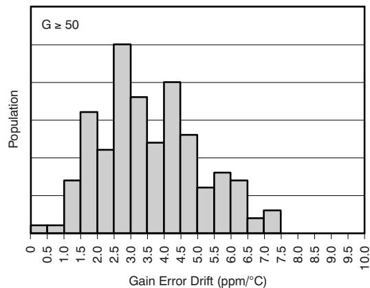
Figure 16. Gain Error Drift ( -40^\circ\text{C} to 125^\circ\text{C} )
