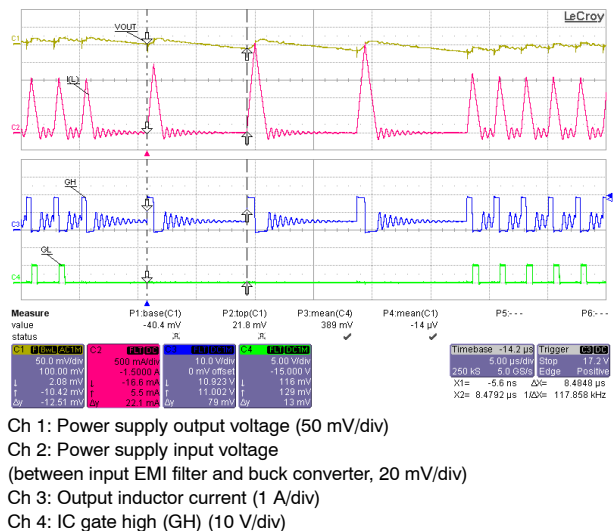
Figure 32. IC Pulse-Skip PWM Behaviour, Borderline Pulse-Skip Region
