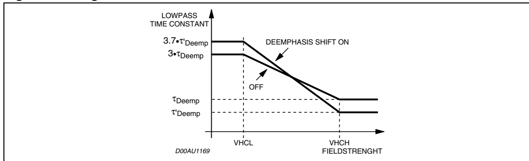
Figure 33. Highcut characteristics
