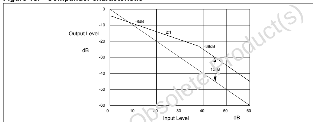
Figure 18. Compander characteristic
