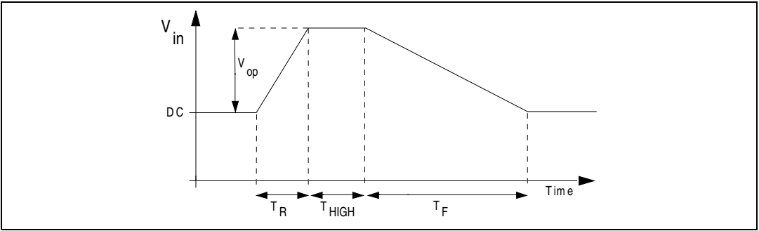
Figure 24. V_n timing diagram
