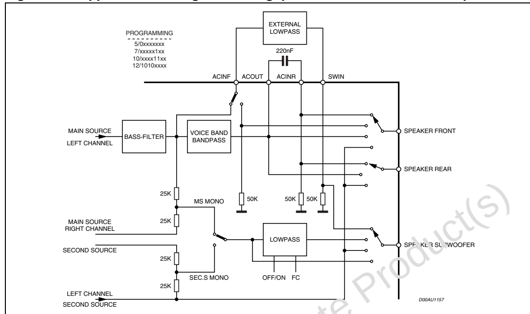
Figure 21. Application 2 using internal highpass and external stereo low pass filter
