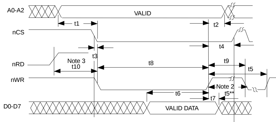
FIGURE 8-10: NON-MULTIPLEXED BUS, 80XX-LIKE CONTROL SIGNALS; WRITE CYCLE
