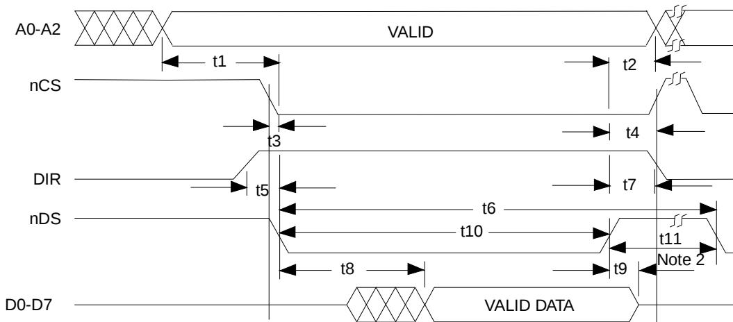
FIGURE 8-7: NON-MULTIPLEXED BUS, 68XX-LIKE CONTROL SIGNALS; READ CYCLE
