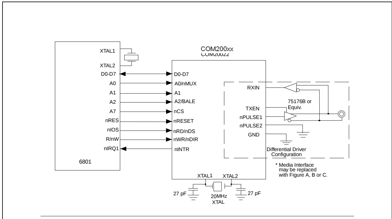
FIGURE 5-2: NON-MULTIPLEXED, 6801-LIKE BUS INTERFACE WITH RS-485 INTERFACE
