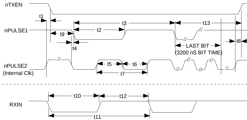
FIGURE 8-13: BACKPLANE MODE TRANSMIT OR RECEIVE TIMING
