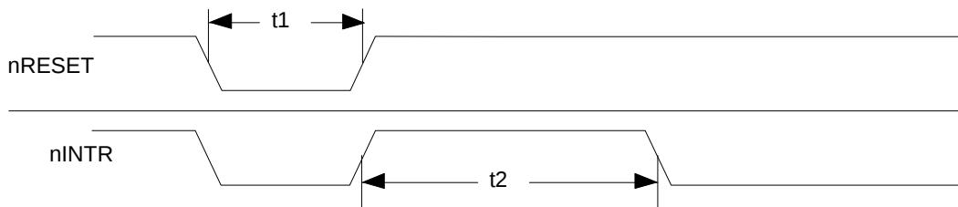
FIGURE 8-15: RESET AND INTERRUPT TIMING
