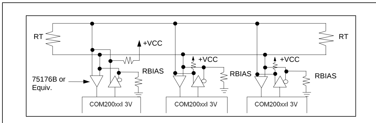
FIGURE 5-4: COM20019i 3V NETWORK USING RS-485 DIFFERENTIAL TRANSCIEVERS
