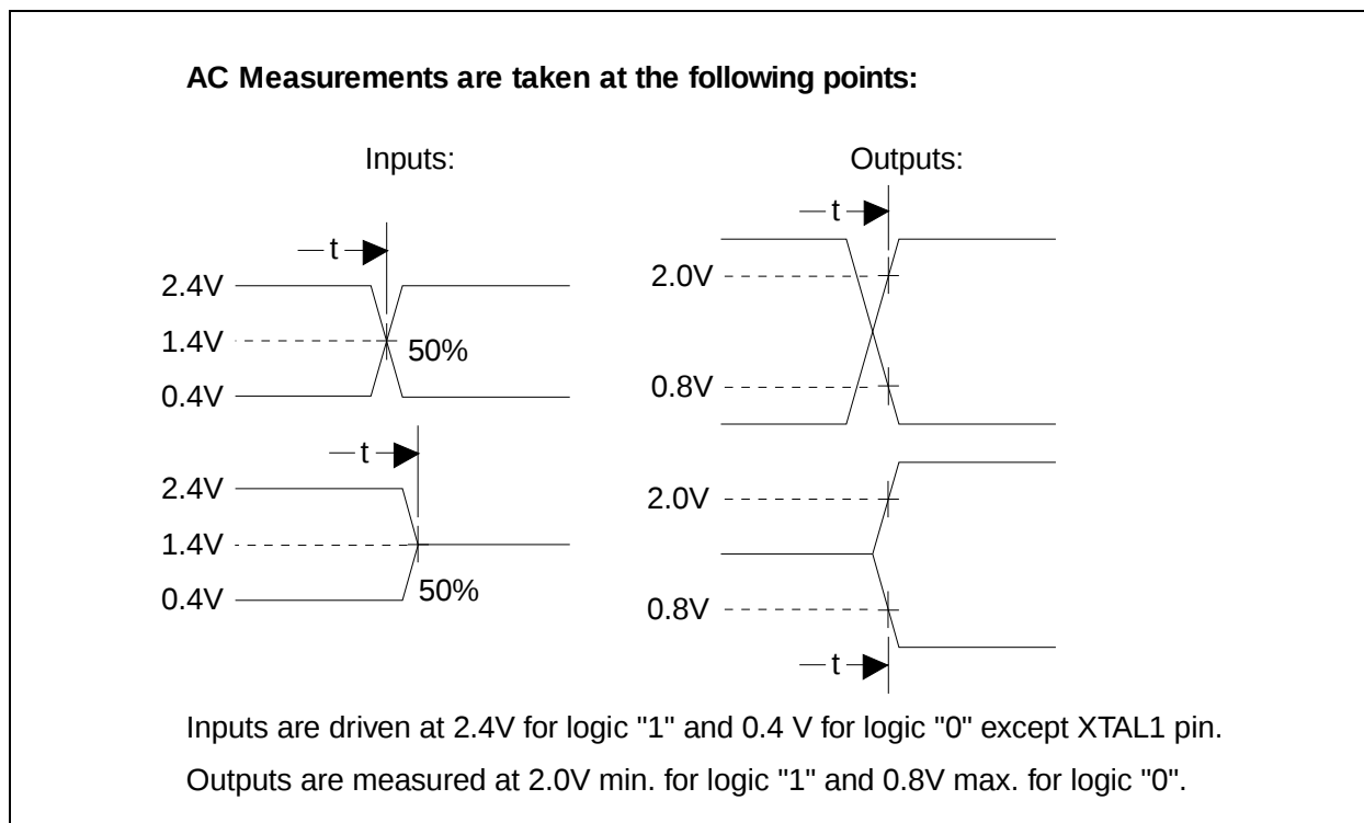
FIGURE 7-1: AC MEASUREMENTS
