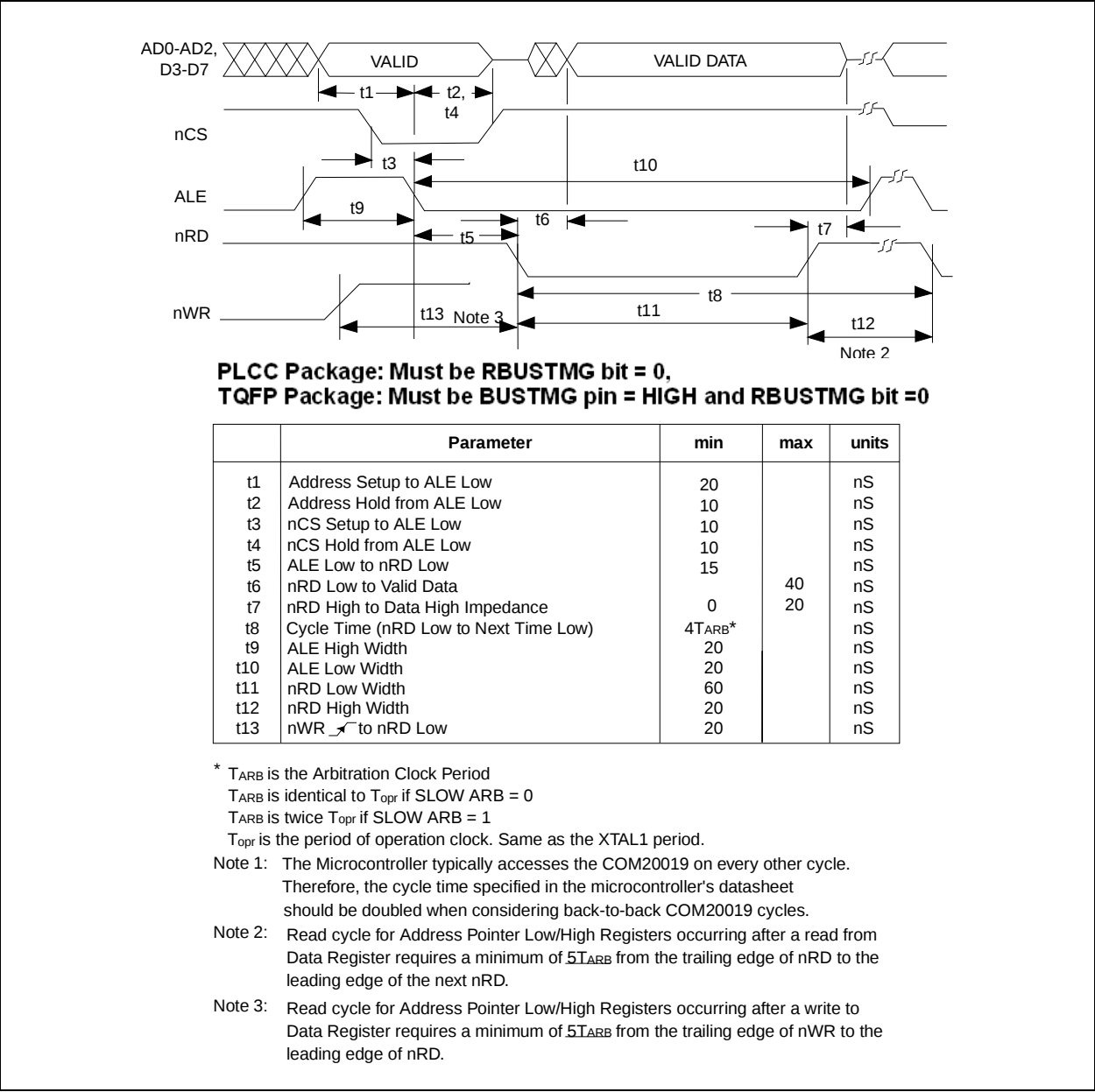
FIGURE 8-2: MULTIPLEXED BUS, 80XX-LIKE CONTROL SIGNALS; READ CYCLE
