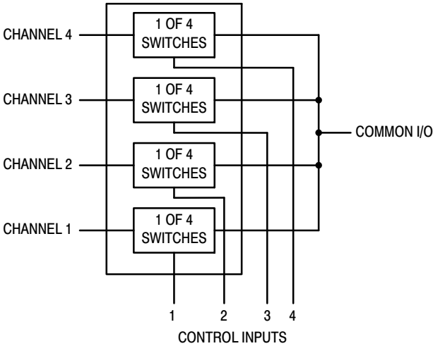
Figure 19. 4-Input Multiplexer
