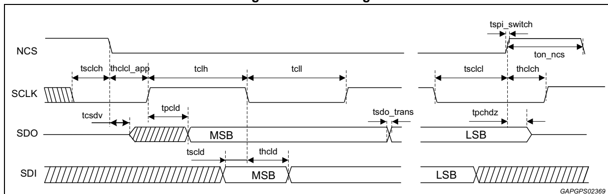
Figure 40. SPI timings
