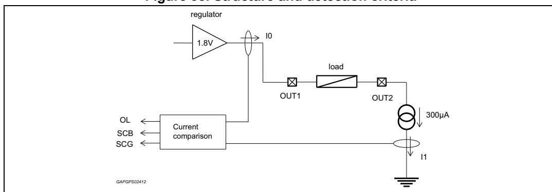
Figure 33. Structure and detection criteria
