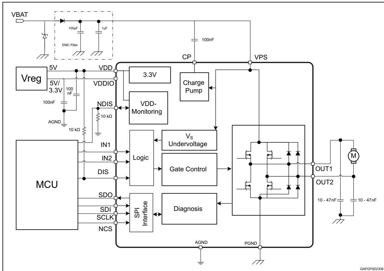
Figure 4. Application diagram
