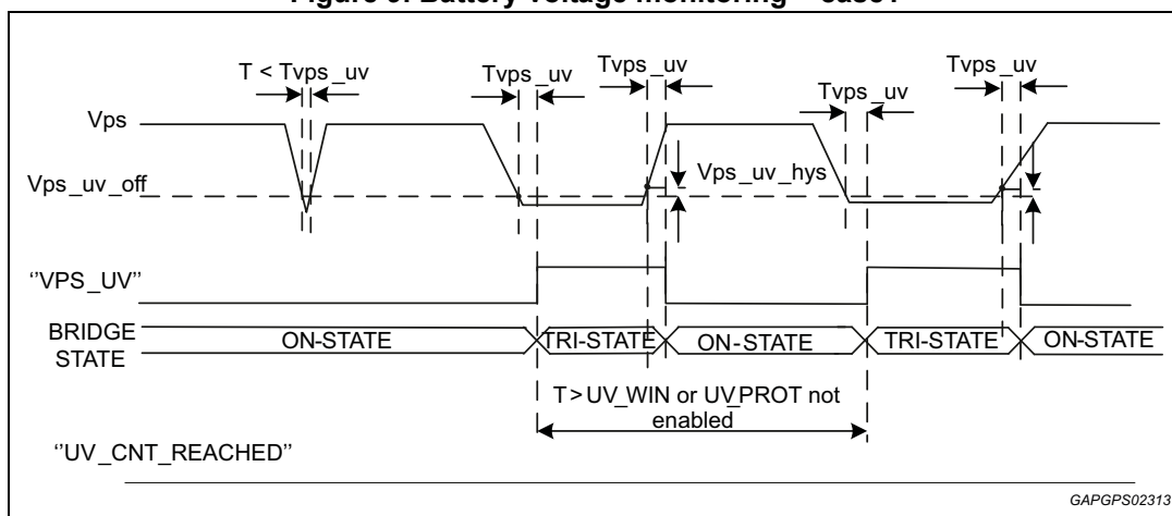
Figure 9. Battery voltage monitoring – case1
