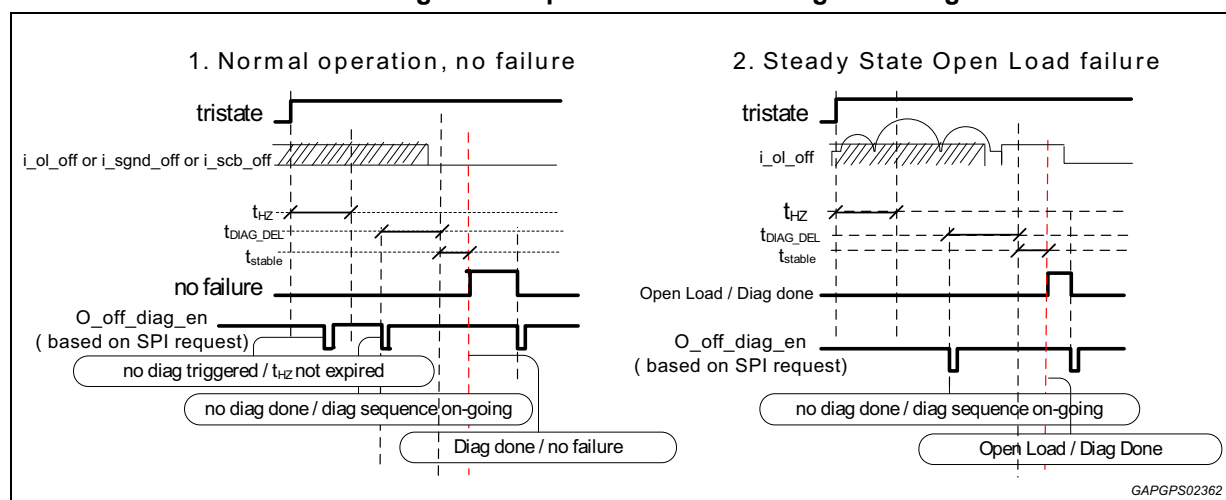
Figure 34. Open load off state diagnosis diagram
