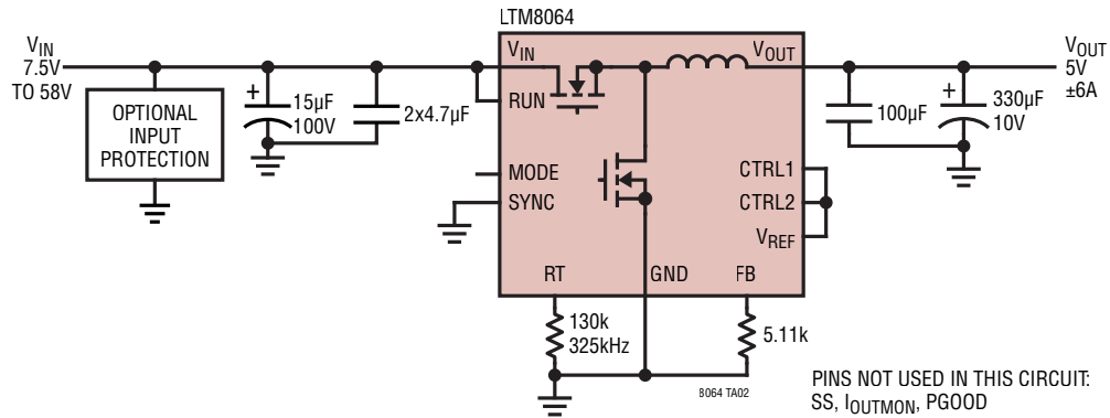
\pm 6A , 5V (2-Quadrant) \mu Module Voltage Regulator
