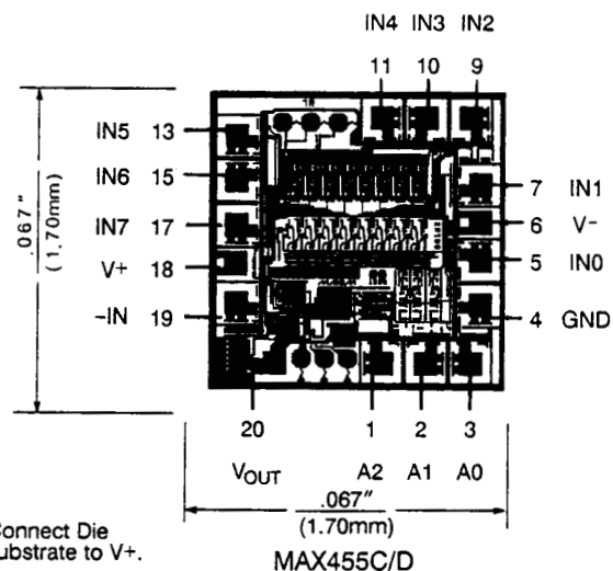
Chip Topographies
